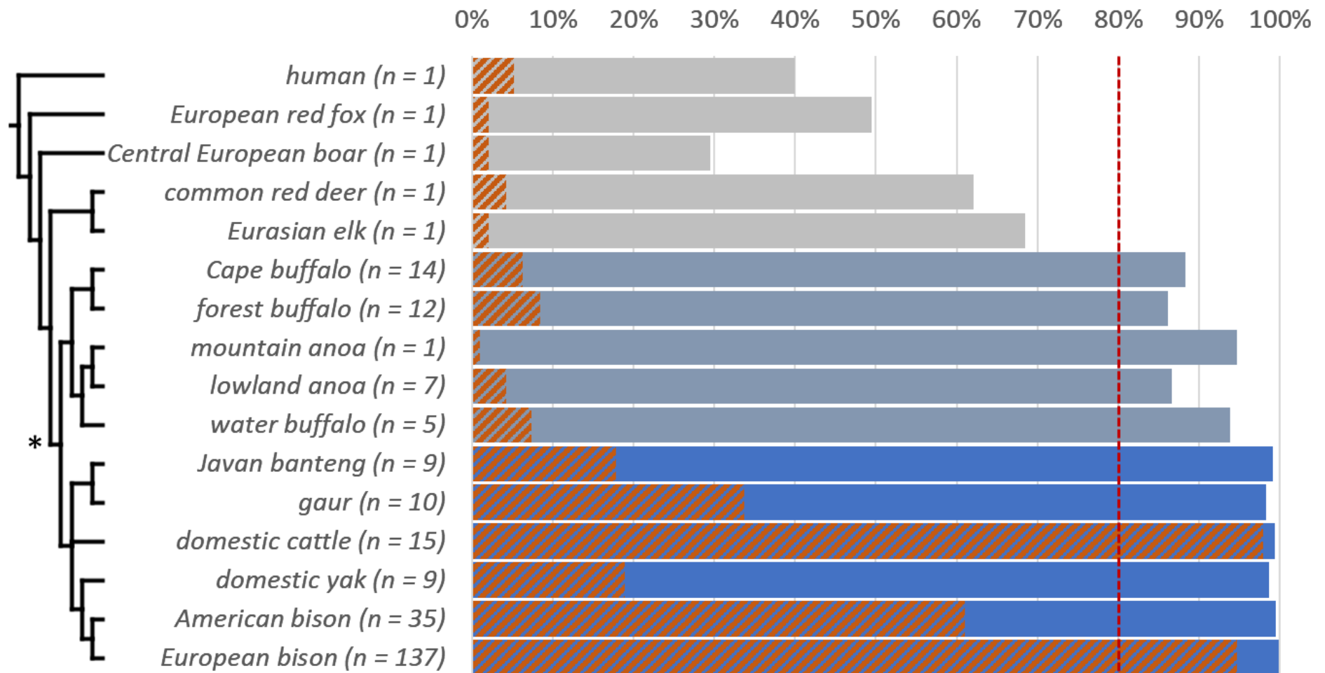
Figure 5: SNP call rate [%] for 95 autosomal SNPs in the European bison and 15 non-target species with corresponding numbers of individuals (n). The length of a solid bar indicates the mean SNP call rate for each analysed species. Blue bars reflect all groups classified to the genus Bos , blue-grey bars groups classified to the subtribe Bubalina and grey bars species outside of Bovini. A SNP call rate of at least 80 % call rate (red dashed line) is the threshold for inclusion into further analysis. The orange-hatched bars show the percentage of found polymorphism over 95 loci within the groups. The cladogram reflects known evolutionary relationships between the species 18 . The asterisk points out the tribe of Bovini.
