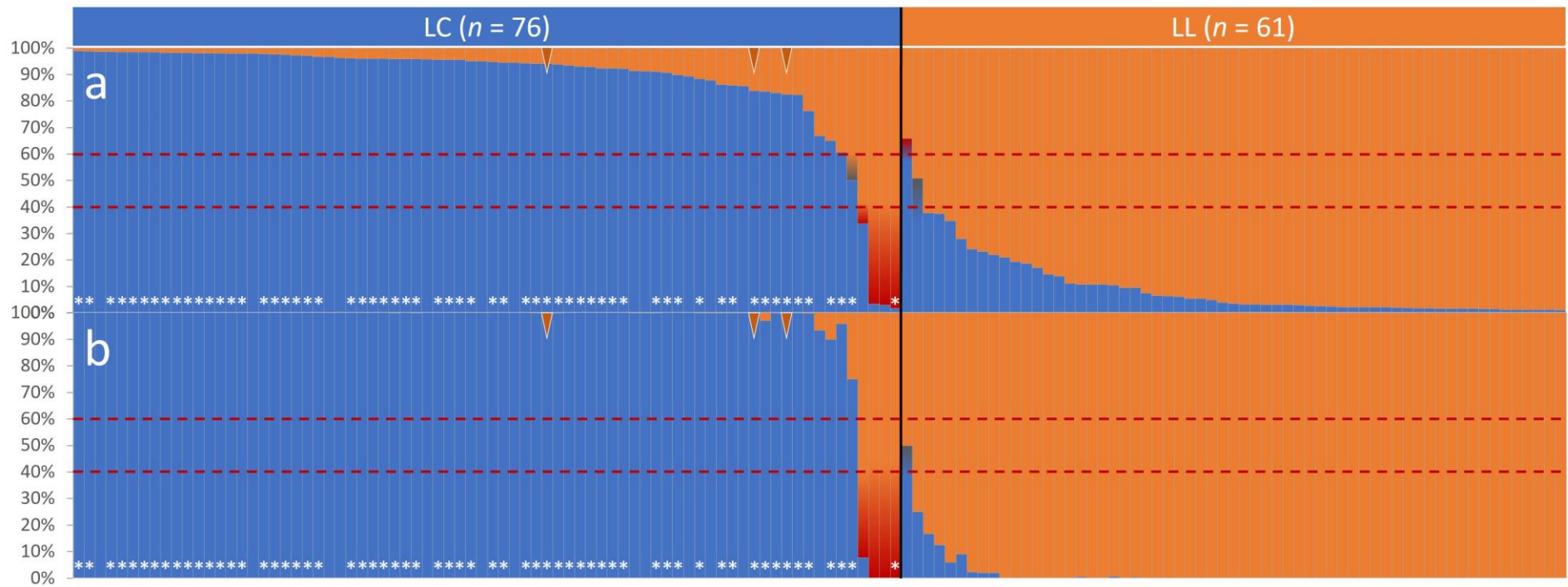
Figure 4: Assignment probabilities [%] based on 18 loci selected for breeding line discrimination between LC ( n = 76 ) and LL ( n = 61 ) in the European bison: (a) Bayesian genetic clustering computed with STRUCTURE ; (b) Maximum-likelihood genetic clustering computed with adegenet . The black line shows the previously assigned lineage distinction (LC: blue; LL: orange). Dashed red lines indicate assignment thresholds. Bars tarnished red mark individuals with unexpected lineage assignment; bars tarnished grey mark individuals not assignable with genotypic data according to the assignment threshold. Brown arrows: F_1 breeding line hybrids. White asterisks: LC individuals with at least one of the six private alleles found in LC. See Supplementary Table S5 for the order of individuals shown here.
