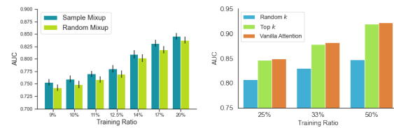
Fig. 4. Ablation Study. Left(a): Sample Mixup corresponds to the current procedure of ScRAT that only mixes cells from the same population. Random Mixup means that we apply mixup to any pairs of cells. The result indicates the validity of current sample mixup method. Right(b): We compare the performance of various attention matrix re-construction strategies to show that attention weights are related to the model performance. For each row of the attention matrix, Top k keeps the top k largest attention weights, and Random k keeps k randomly selected attention weights, before normalizing the matrix for the remaining fields. Here, k is set to 5. The results of ScRAT using the original attention matrix described in Eq. 3 is denoted by Vanilla Attention . The result shows that top k method achieves AUC comparable to using all attention weights, and they are both better than random k attention. This provides strong evidence of the connection between high attention weights and model performance.
