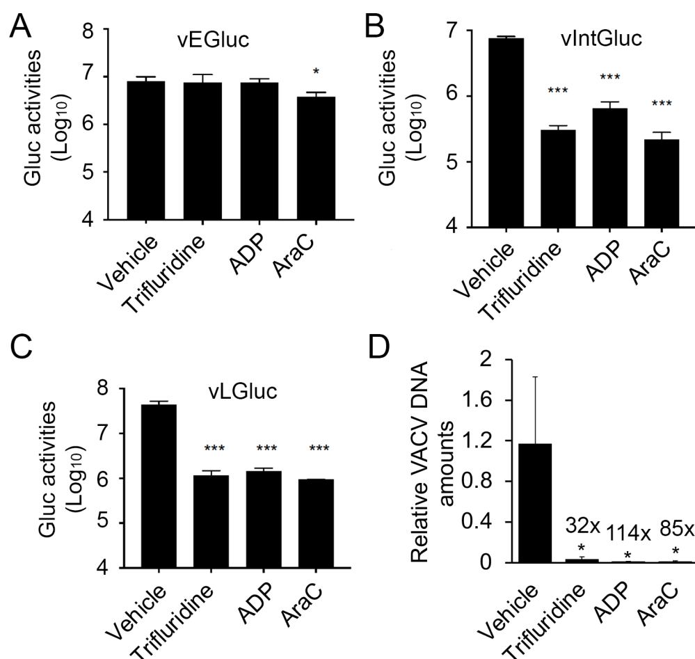
Fig. 4. Trifluridine and adefovir dipivoxil suppress VACV DNA replication and post-replicative gene expression, but not early gene expression. (A-C) HFFs were infected with vEGluc ( A ), vIntGluc ( B ), and vLGluc ( C ) at an MOI of 2 and treated with indicated compounds at 10 \mu M, respectively, or vehicle DMSO. Gluc activities were measured at 4 h (vEGluc), 8 h (vIntGluc), and 8 h (vLGluc), respectively. ( D ) HFFs were infected with VACV at an MOI of 2 in the presence of indicated compounds at 10 \mu M for 8 h. relative amounts of Viral DNA were determined by real-time PCR using VACV specific primers. At least three repeats were performed for all assays. *0.01<p \le 0.05; ***0.001<p \le 0.01; ns, not significant.
