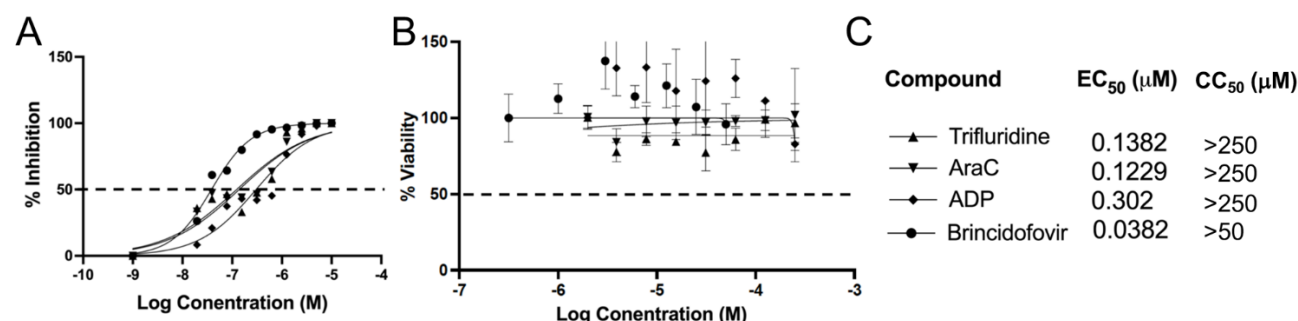
Fig. 3. Measurement of EC 50 and CC 50 of indicated compounds in HFFs. (A) HFFs were infected with vLGluc at an MOI of 0.01 and treated with indicated individual compounds at a series of concentrations (or vehicle DMSO) for 24h. Gluc activities were measured to determine the EC 50 . (B) HFFs cell viabilities were determined by an MTT assay after incubated with indicated compounds at a series of concentrations for 24 h. (C) EC 50 and CC 50 of the compounds in A and B are shown. At least three repeats were performed for all experiments.
