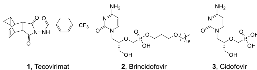
Fig. 1. Structures of FDA-approved smallpox drugs. Tecovirimat ( 1 ) inhibits viral release by targeting the envelop protein VP37. Brincidofovir ( 2 ) is the prodrug of Cidofovir ( 3 ) which targets viral polymerase.
