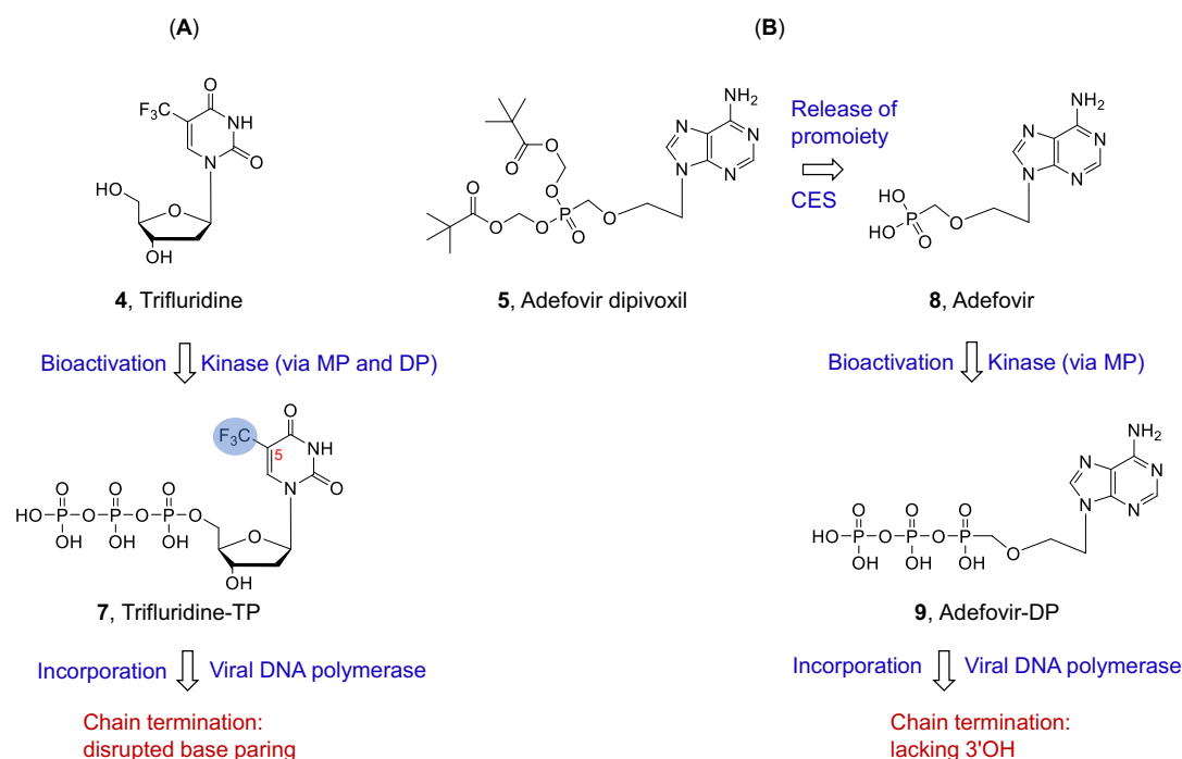
Fig. 6. Mechanism of action of nucleoside analog trifluridine ( 4 ) and nucleotide analog prodrug adefovir dipivoxil ( 5 ). (A) Trifluridine is intracellularly converted into TP by thymidine kinases. Upon incorporation by viral DNA polymerase, the -CF_3 group at the 5 position disrupts base pairing and terminates viral DNA. (B) Ester prodrug adefovir dipivoxil is intracellularly converted into adefovir first under the action of carboxylesterase (CES). The subsequent phosphorylation by AMP kinase produces the active adefovir-DP. When incorporated, obligate termination of the viral DNA chain occurs due to the lack of the 3'OH.
