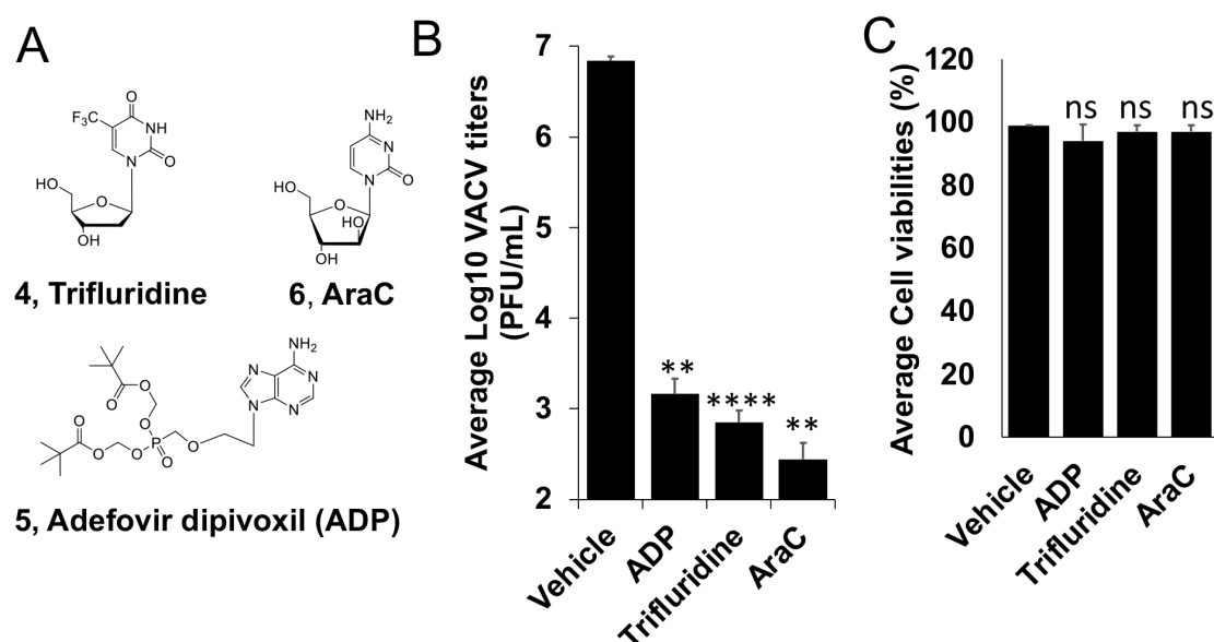
Fig. 2. Inhibition of VACV replication by trifluridine and Adefovir dipivoxil (ADP) by plaque assay. (A) Structures of trifluridine (4), adefovir dipivoxil (ADP, 5), and AraC (6). (B) HFFs were infected with VACV at an MOI of 0.01 treated with indicated compounds at 10 \mu M for 48 h. Viral yields were titrated using a plaque assay on BS-C-1 cells. (C) HFF cell viabilities were measured 48 h after the cells were treated with indicated compounds at 10 \mu M. At least three repeats were performed for all assays. **0.001 < p \leq 0.01, ns, not significant.
