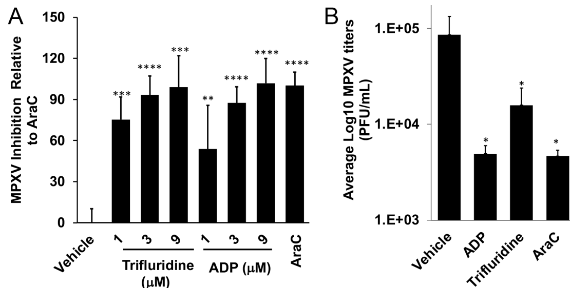
Fig. 5. Inhibition of MPXV replication by trifluridine and Adefovir dipivoxil (ADP). (A) HFFs were infected with MPXV-WA-2003-Fluc (luc+MPXV) under an early/late promoter (MOI=0.01) treated with indicated compounds at indicated concentration for 24 h. Firefly luciferase activities were measured. The inhibition by AraC were normalized to 100. (B) MPXV-MA001 2022 isolate was added to cells at an MOI of 2 for 1 h. Virus was removed, cells were washed with PBS and trifluridine or adefovir dipivoxil was added at 10 μM. Cells were harvested 24 h post infection. AraC treatment was used as the positive control. Viral yields were titrated using a plaque assay on E6 cells. Each treatment was tested in triplicate. * p \leq 0.05 , ** 0.001 < p \leq 0.01 , *** 0.0001 < p \leq 0.001 , **** 0.00001 < p \leq 0.0001 , ns, not significant.
