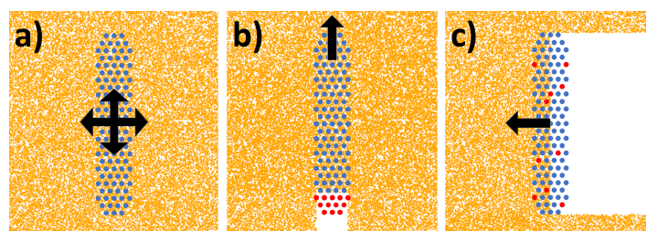
FIG. 10. (a) In reaction-limited diffusion, without catalytic activity, the distribution of the center of mass trajectories is uniform, irrespective of the particle's shape. 24 (b) Polarized particles preferentially move along the particle's axis. (c) Particles featuring uniform distributions of NA ligands preferentially move orthogonally to the particle's axis.
