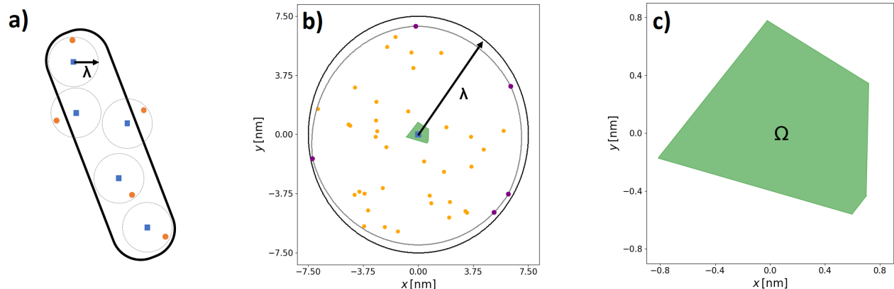
FIG. 3. (a) The possible positions and orientations of the virion are determined by the bridges as the ligand-receptor distance is constrained to remain smaller than \lambda . (b) Geometrical construction employed in Ref. 24 in which each pair of bound molecules (represented by squares and circles in a) is rigidly translated to overlap all ligands' position (squares) with the center of mass of the particle. The dynamics of the system (at a given \theta ) are then described by a circle of radius \lambda rattling around the receptors (circles). The n_{cb} constraining bridges correspond to the receptors that can enter into direct contact with the border of the rattling circle (purple points). For clearness, in a we use fewer bridges than in b (in b we have n_b = 40 as in most of the systems studied in this work). (c) \Omega is the configuration space scanned by the center of mass in the rattling dynamics. \Omega is constituted by a number of vertices equal to n_{cb} jointed by arcs of radius \lambda . 24 For 40 bridges and \lambda = 7.5 nm, the size of \Omega is \approx 1 nm.
