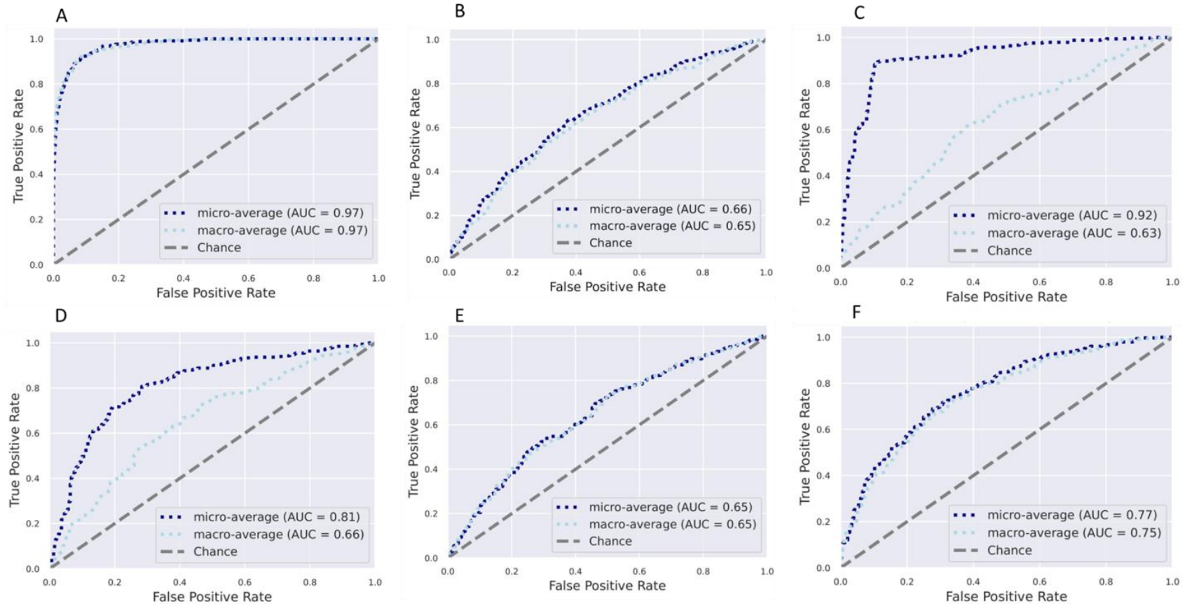
Figure 2. Receiver operating characteristic curves showing the classification accuracy of gut microbiota in a Random Forest model. Classification accuracy for estimating (A). All countries; (B) Obesity status, (C). Diabetes status; (D). Glucose status; (E). Hypertensive status; (F). Sex are presented. AUC= area under the curve
