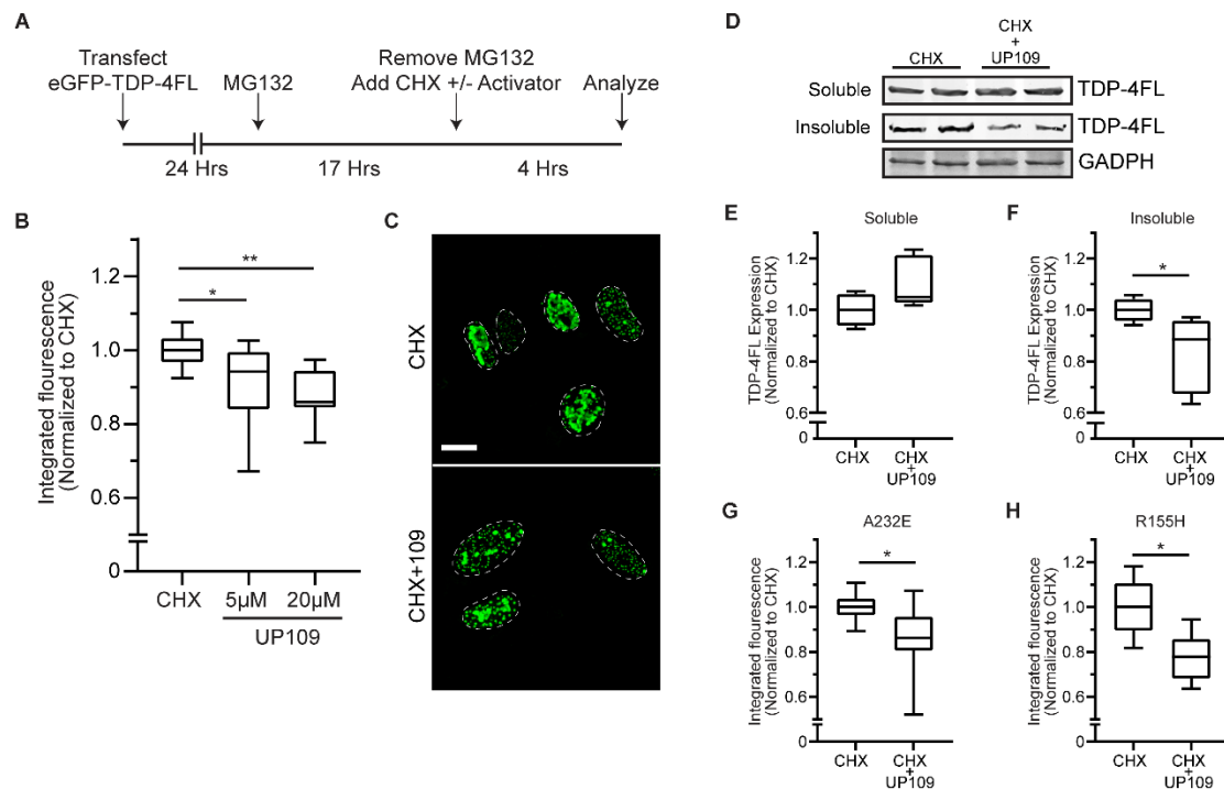
Figure 7: VCP activator enhances clearance of intranuclear TDP-4FL inclusions.
