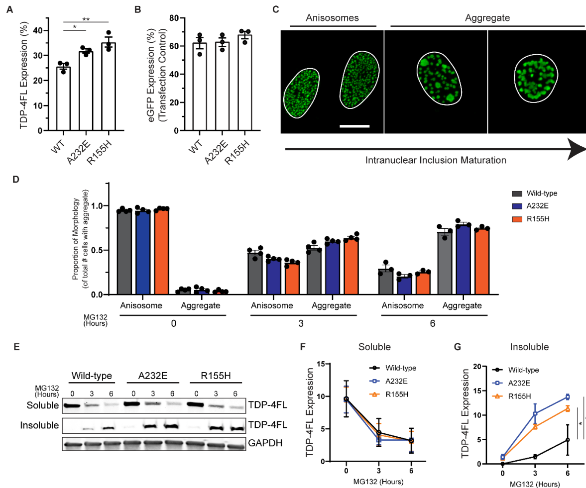
Figure 3: TDP-4FL anisosomes become larger and more insoluble due to pathogenic A232E and R155H VCP variants.
