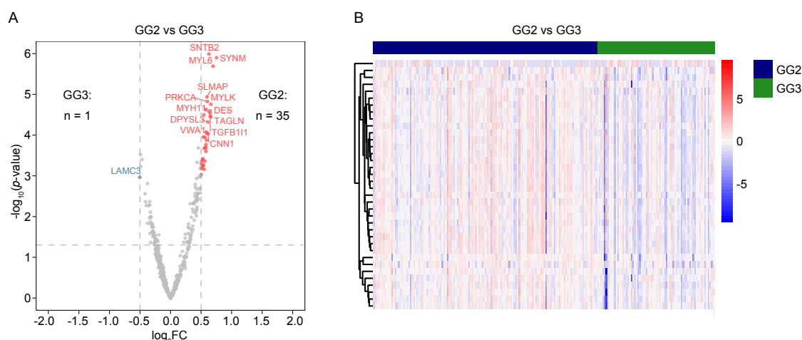
Figure 2. Differentially expressed proteins in GG2 vs GG3. A. A volcano plot showing the GG2 (n = 35) and GG3 (n = 1) enriched proteins in tumours with FC > 1.5 and < 0.67 and p\text{-value} < 0.01 . Significant proteins are presented in red and blue colour, whereas other proteins are coloured in grey. Only a small number of proteins were found to be significant using differential expression analysis while most of them showed low FC. B. Heatmap representation of the expression levels of differentially expressed proteins between GG2 and GG3 samples shown in A. Expression data are converted to z-scores. Samples are shown on the x-axis whereas proteins are clustered on the y-axis.
