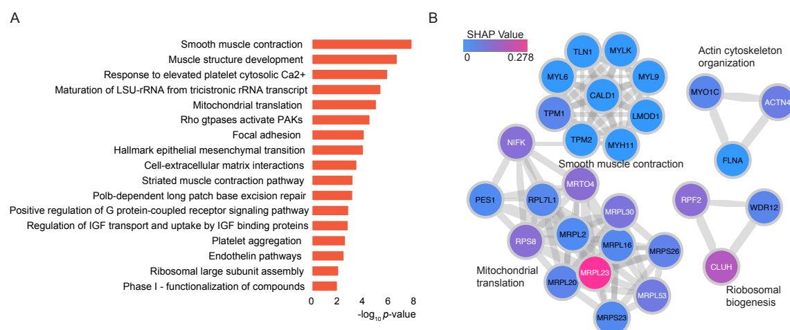
Figure 4. Differentially expressed proteins and pathways in GG2 and GG3 PCa. A. GO biological processes, Reactome pathways and hallmark gene sets enriched for the selected significant proteins. B. PPI network components obtained using MCODE algorithm, showing the enriched biological processes and proteins. Proteins are coloured according to the absolute mean SHAP values. The width of the edge (between nodes) indicates the strength of the connection. Functional description is provided beside each component.
