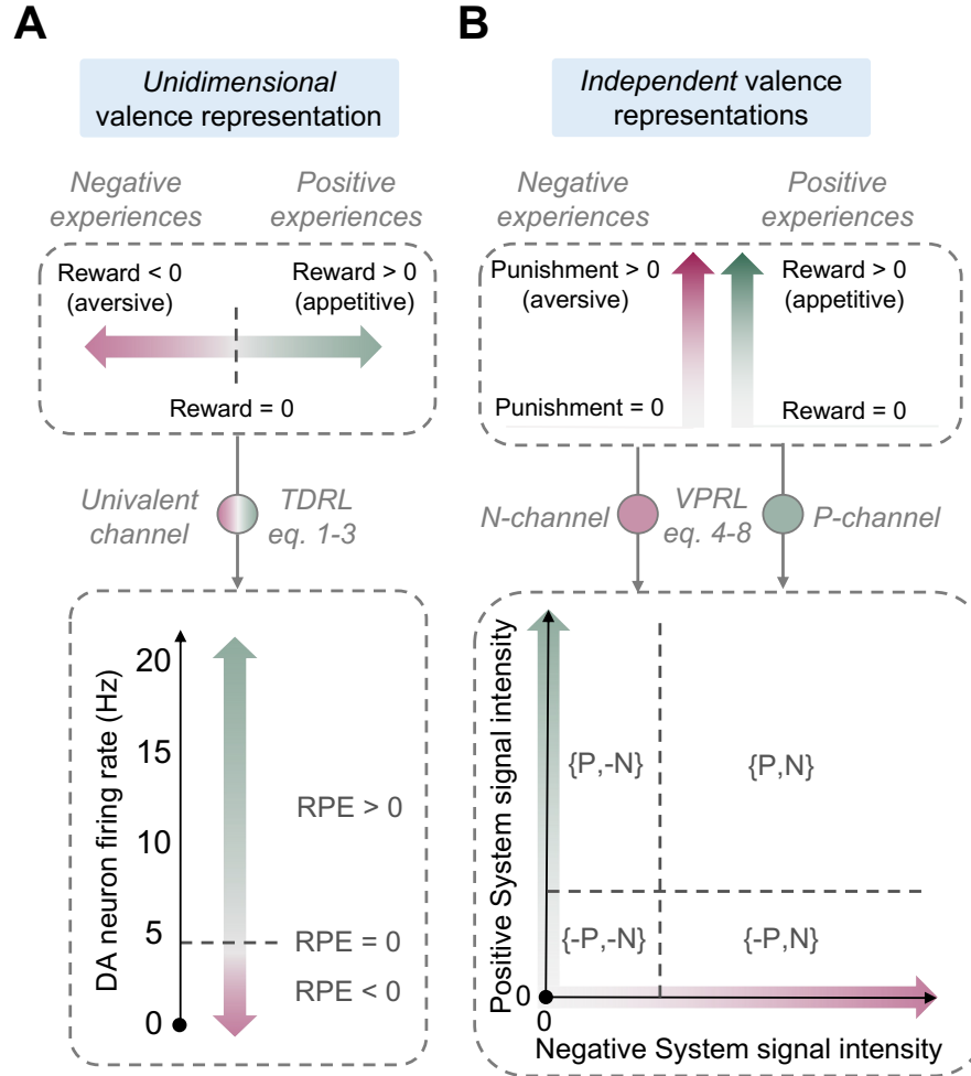
Fig. S1. Alternative computational theories of valence processing in reinforcement learning. (A) Traditional temporal difference reinforcement learning (TDRL) theory represents rewards and punishments unidimensionally as opposite ends of a single continuous valence dimension. The physiological support for this traditional view is limited by how dopamine neurons might encode aversive outcomes. (B) A valence-partitioned reinforcement learning (VPRL) approach instead specifies that rewards and punishments are processed by independent valence-processing systems in parallel. The space spanned by the activity within these two systems of VPRL (the Positive system and Negative system \{\pm P, \pm N\} space) captures all combinations of possible valent experiences.
