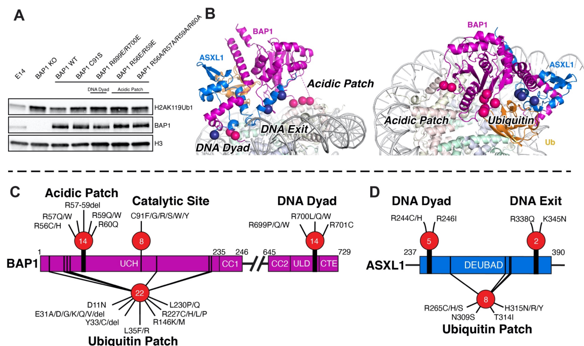
Fig. 4. BAP1/ASXL1-nucleosome contacts are extensively mutated in cancers. (A) Western blot analysis using the indicated antibodies of total protein extracts from BAP1 WT (E14) or KO mESC with stable expression of WT and various BAP1 mutations (C91S, R699E/R700E; R56E/R59E; R56A/R57A/R59A/R60A). (B) Structure of the BAP1/ASXL1-H2AK119Ub nucleosome complex highlighting three key nucleosome anchors (left) and Ub interactions (right) with cancer mutations shown as colored spheres. Bar diagram showing cancer-associated point mutations and deletions to BAP1 (C) and ASXL1 (D) at nucleosomal anchors and the Ub patch shown in (B) identified in several cancers that can be mechanistically explained by studies presented here. The number of unique cancer types at each interface is shown inside the red spheres.
