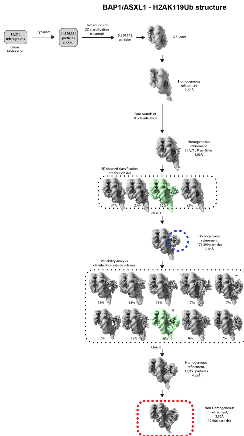
Fig. S4. 3D classification scheme of BAP1/ASXL1-H2AK119Ub nucleosome samples. Processing scheme for classification of BAP1/ASXL1-H2AK119Ub nucleosome complex dataset collected on Titan Krios operated at 300 kV. Images represent the path that led to the final subset, with particles and map selected for each step shown in green. A mask applied to BAP1/ASXL1 in 3D focused classification and variability analysis is shown in a blue circle. In the variability analysis step, the most stable conformation (classes 5 and
