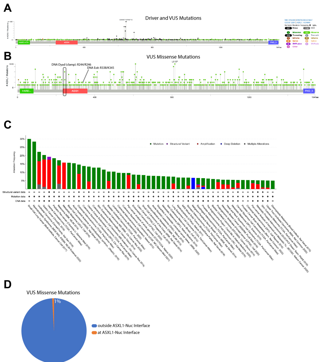
Fig. S15. ASXL1 mutations found in cancer. Searching the cBioPortal database for a curated set of non-redundant cancer studies on ASXL1. A and B) Driver and VUS mutations are mapped across the amino acid sequence of ASXL1 with mutational frequency represented as high. C) ASXL1 cancer associated mutations compared with alteration frequency and associated disease. D) Pie chart representation of the total number of VUS mutations and the number of VUS mutations at BAP1-Nucleosome interfaces.
