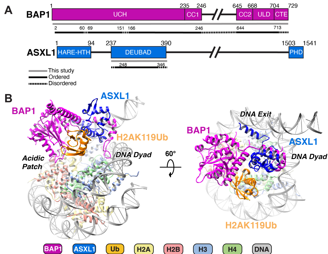
Fig. 1. Overview of the structure of BAP1/ASXL1 bound to H2AK119Ub nucleosome.
