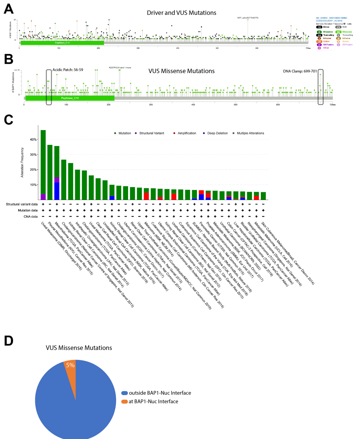
Fig. S14. BAP1 mutations found in cancer. Searching the cBioPortal database for a curated set of non-redundant cancer studies on BAP1. A and B) Driver and VUS mutations are mapped across the amino acid sequence of BAP1 with mutational frequency represented as high. C) BAP1 cancer associated mutations compared with alteration frequency and associated disease. D) Pie chart representation of the total number of VUS mutations and the number of VUS mutations at BAP1-Nucleosome interfaces.
