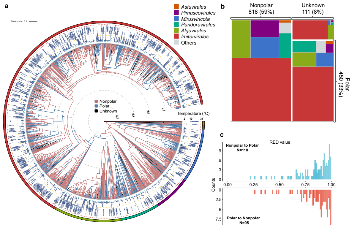
Fig. 2 | Inferred ancestral polar and non-polar niches for viruses. a, Ancestral “Polar” and “Nonpolar” states were estimated using the phylogenetic tree based on a one-parameter equal rates model. The outermost layer shows the taxonomy of six main groups. The boxplots in the second layer show the temperature optima of the viral genomes. Only polar and nonpolar genomes were included in the tree. b, The treemap diagram shows the number of viruses assigned to Polar, Nonpolar or “Unknown” biomes. Colours indicate the main taxonomic groups. c, Histograms of Relative Evolutionary Divergence (RED) values for the nodes at which “polar” or “nonpolar” adaptation events were inferred.
