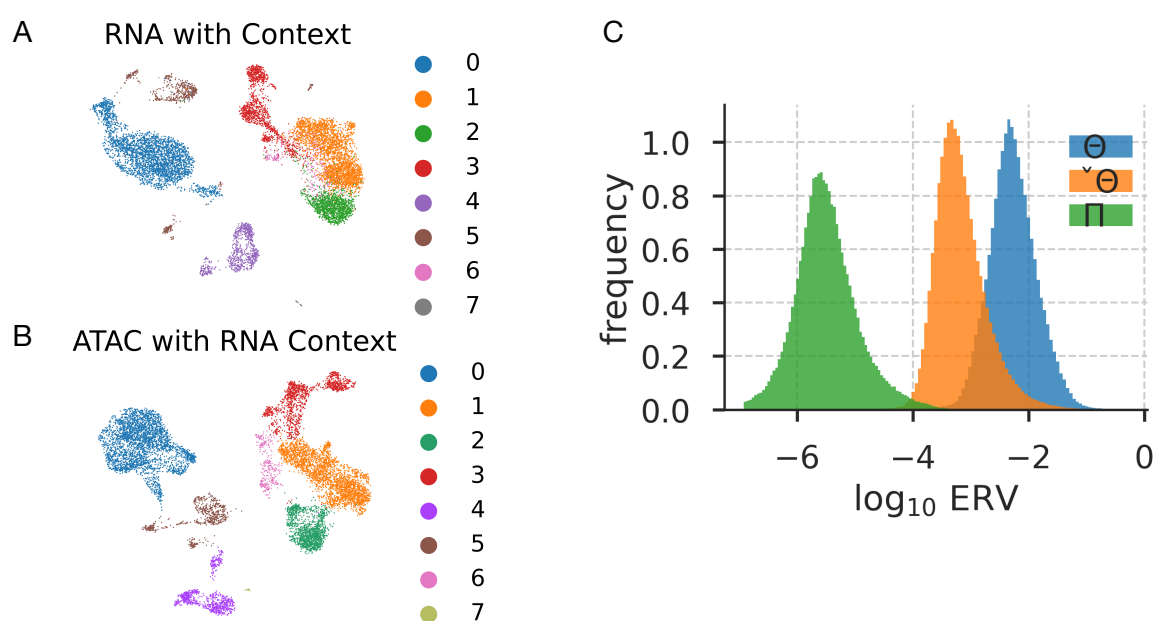
S11: Single cell PBMC Contexts and Networks A: UMAP projection of the scRNA-Seq PBMC dataset with “Context” via leiden clustering (0.2) B: UMAP projection of the scATAC-Seq PBMC dataset with “Context” via leiden clustering (0.2) C: Distribution of ERV for \hat{\Theta} , \Pi and \Theta networks
