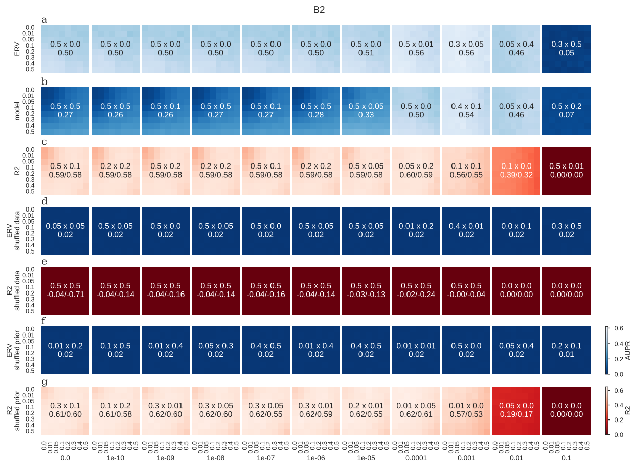
S5: Dataset B2[66]. Description as in Figure S2
