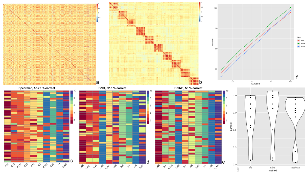
Figure 7. (a) Heatmap of BZINB-based correlation between Kraken2/Bracken counts of 400 of the species in ZOE2.0 in a random order; (b) Heatmap of BZINB-based correlation of the Kraken2/Bracken count data (in the same order as in (a)) after introducing simulated clusters; (c-e) Each column of cells represents a true cluster based on the simulation (b), and the colors represent the predicted clustering using affinity matrix made from (c) BNB, (d) BZINB, and (e) Spearman correlations; (f) Distance (Frobenius norm) between the correlation matrices of nested predicted clusters between data with (as in Figure 7b) and without (as in Figure 7a) increased correlations that represented the clusters: the first set (number of clusters = 1) is the predicted cluster with the greatest distance between correlation matrices. For each increase in the number of clusters, we included an additional cluster in the order of decreasing distances. This was done using the BNB-based, BZINB-based, and Spearman correlation matrices and their corresponding cluster predictions; (g) Violin plot of cluster-wise percent accuracy for each of the 10 clusters, comparing BNB, BZINB, and Spearman correlation-based affinity matrices.
