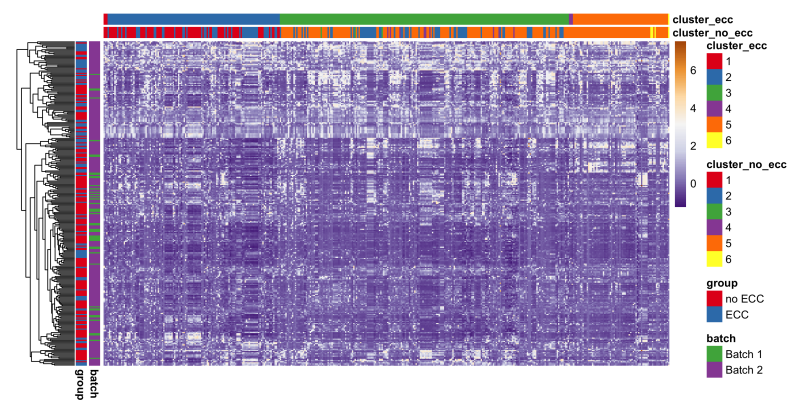
Figure A6: Heatmap of species abundance illustrating species modules identified by spectral clustering (shown as the two top bars). Columns represent individual species and are ordered by the clusters predicted from the affinity matrix based on the BZINB correlations between species in the diseased (ECC) group. Columns are annotated to show and compare the predicted clusters between health (no ECC) and disease (ECC) groups. Each row represents a participant ( n=289 ). The rows are ordered based on hierarchical clustering and are annotated to illustrate health and disease groups and the sequencing batch. Standardized counts were used.
