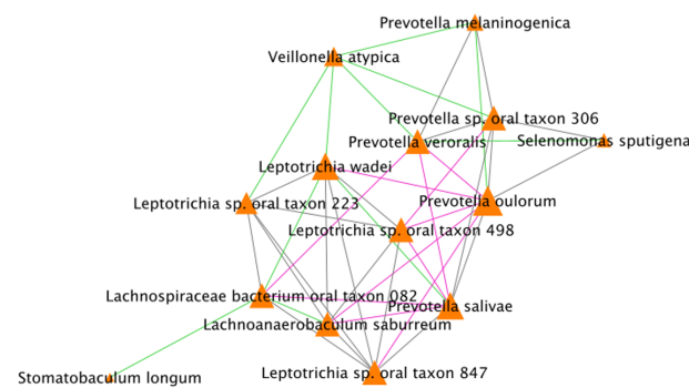
Figure 11. Spearman correlations between species. The strongest 30% of correlations are included in the diagrams, and the color of the lines represent whether the correlation was strong in one or both of the health/disease groups.
