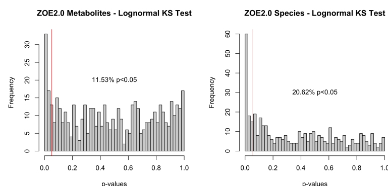
Figure 3. P-values obtained from lognormal (parameters from models fitted on nonzero counts for ZOE 2.0 metabolites and Kraken2/Bracken microbiome species) Kolmogorov-Smirnov test for ZOE 2.0 metabolites and Kraken2/Bracken microbiome species.
