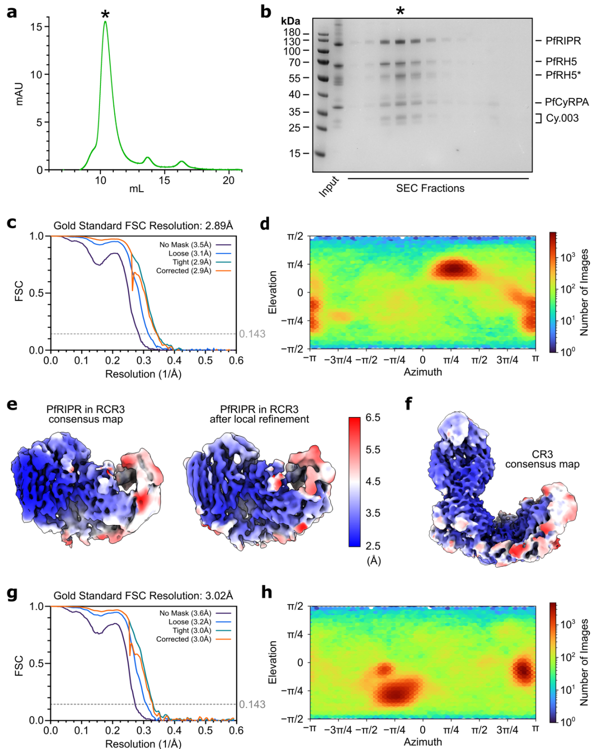
Extended Data Figure 1: Purification of PfRCR-Cy.003 complex and cryo-EM processing statistics
