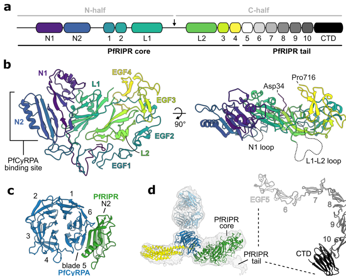
Figure 3: The structure of PfrIPR
