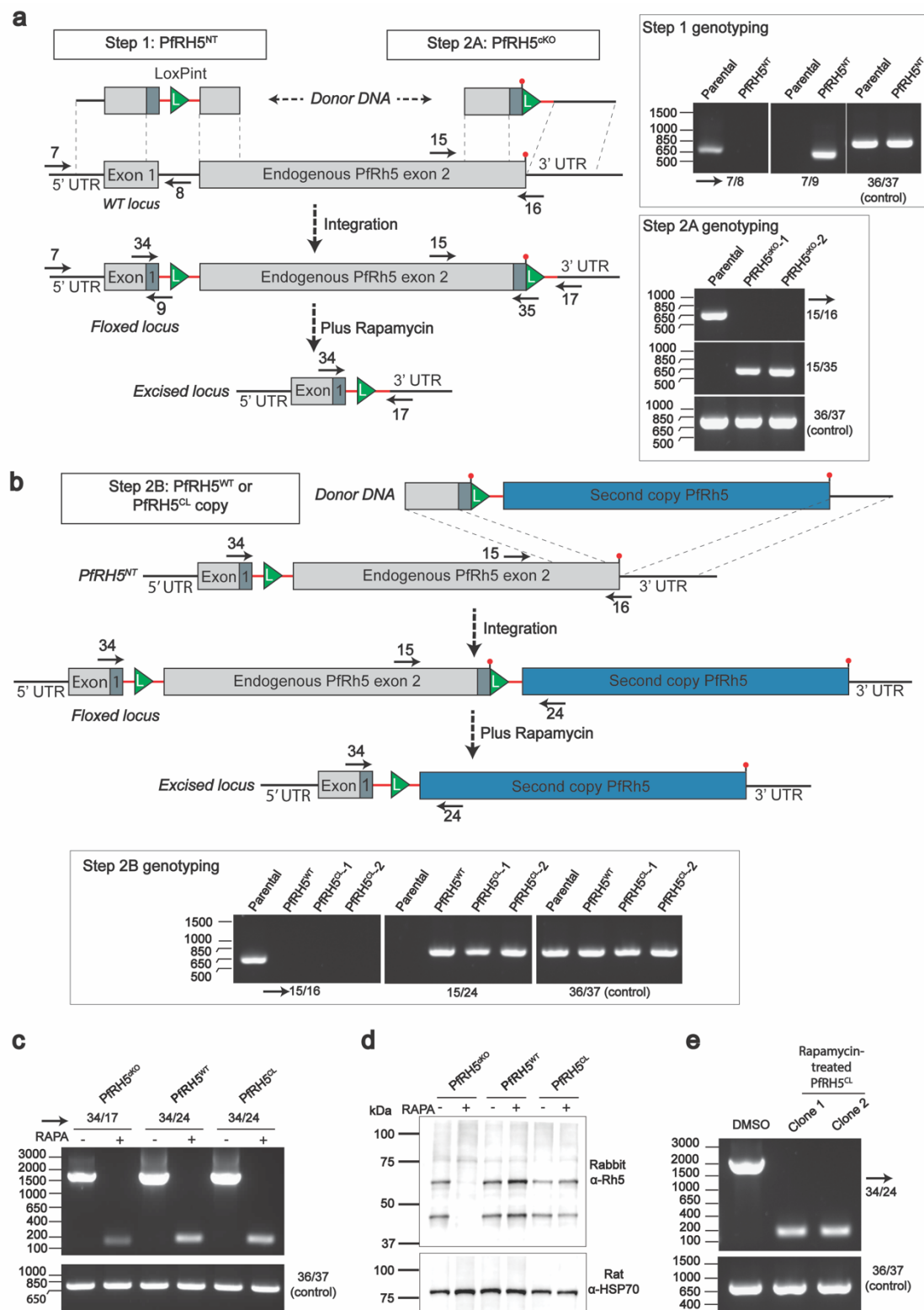
Extended Data Figure 6: Generation of PfrH5 conditional knockout and complemented parasites
