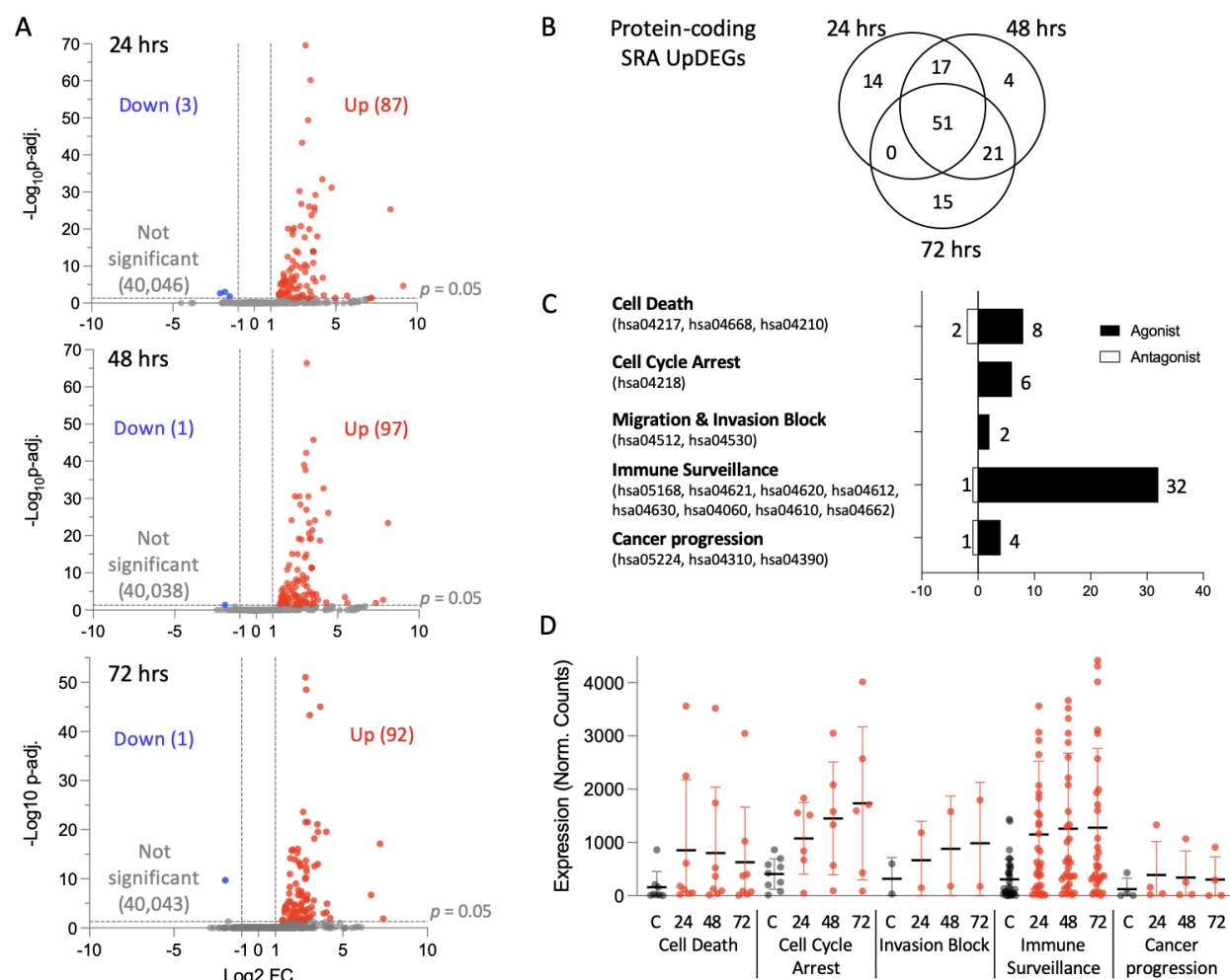
Figure 4. Transcription profiling of SRA-PcTF-expressing BT-549 cells. (A) Volcano plot of log2 fold change ratios for each time point. Differentially regulated genes (DEGs, |\text{FC}| \geq 2 , adjusted p < 0.05 ) are highlighted blue for downregulation or red for upregulation. (B) Venn diagram of protein-coding SRA-upregulated DEGs (UpDEGs) from each time point. (C) Functional categorization of SRA UpDEGs. KEGG pathway IDs are shown. Genes are listed in Supplemental Table 3. (D) Expression values (average normalized counts for two replicates) of UpDEGs within the five functional categories in panel C. Data for the Cell Death group exclude antagonists BIRC3 and TNFAIP3 . Data for the Cancer Progression group exclude the antagonist CDKN1A .
