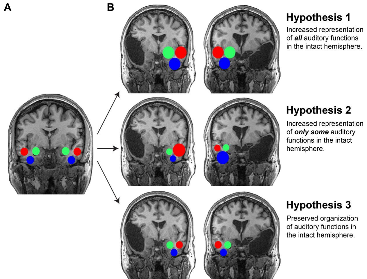
Figure 2 – Hypotheses for functional organization of the auditory cortex in the presence of extensive contralateral temporal lobe lesions. The colored circles represent neural activation to functional auditory component (each color corresponds to a different component). A – Activations observed in neurotypicals. B – Hypotheses for activations observe in individuals missing one temporal lobe from birth.
