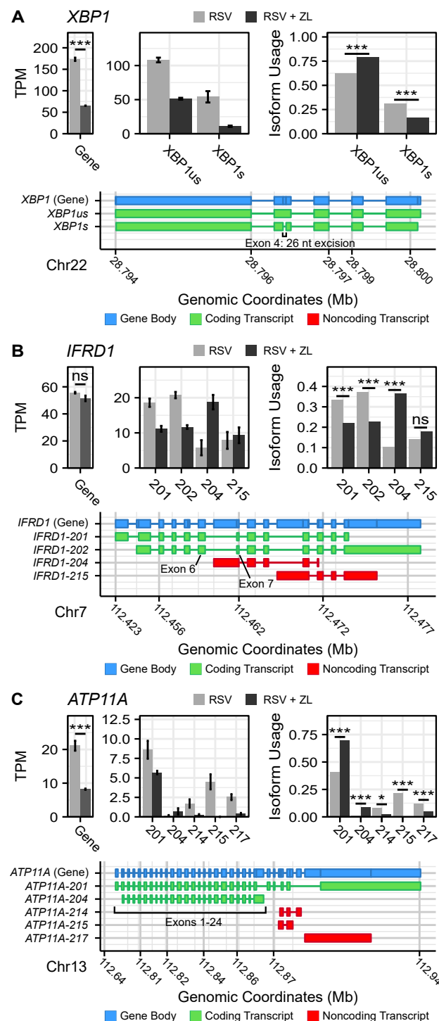
Figure 2: BRD4 inhibition induces isoform switching in key innate inflammation co-regulators. Transcript maps, RNA-seq quantitation in Transcripts-per-Kilobase Million (TPM), and isoform usage of detected transcripts belonging to (A) XBPI , (B) IFRD1 , and (C) ATP11A . Mapped transcripts are plotted in compressed genomic coordinates and color coded according to gene body and coding status. Barplots represents the mean of n=4 replicates per group. Error bars indicate the 95% confidence interval. Transcripts with less than 5% of total detected transcript abundance were omitted from this figure. *P_{Adj} < 0.05 ; ***P_{Adj} < 0.001 .
