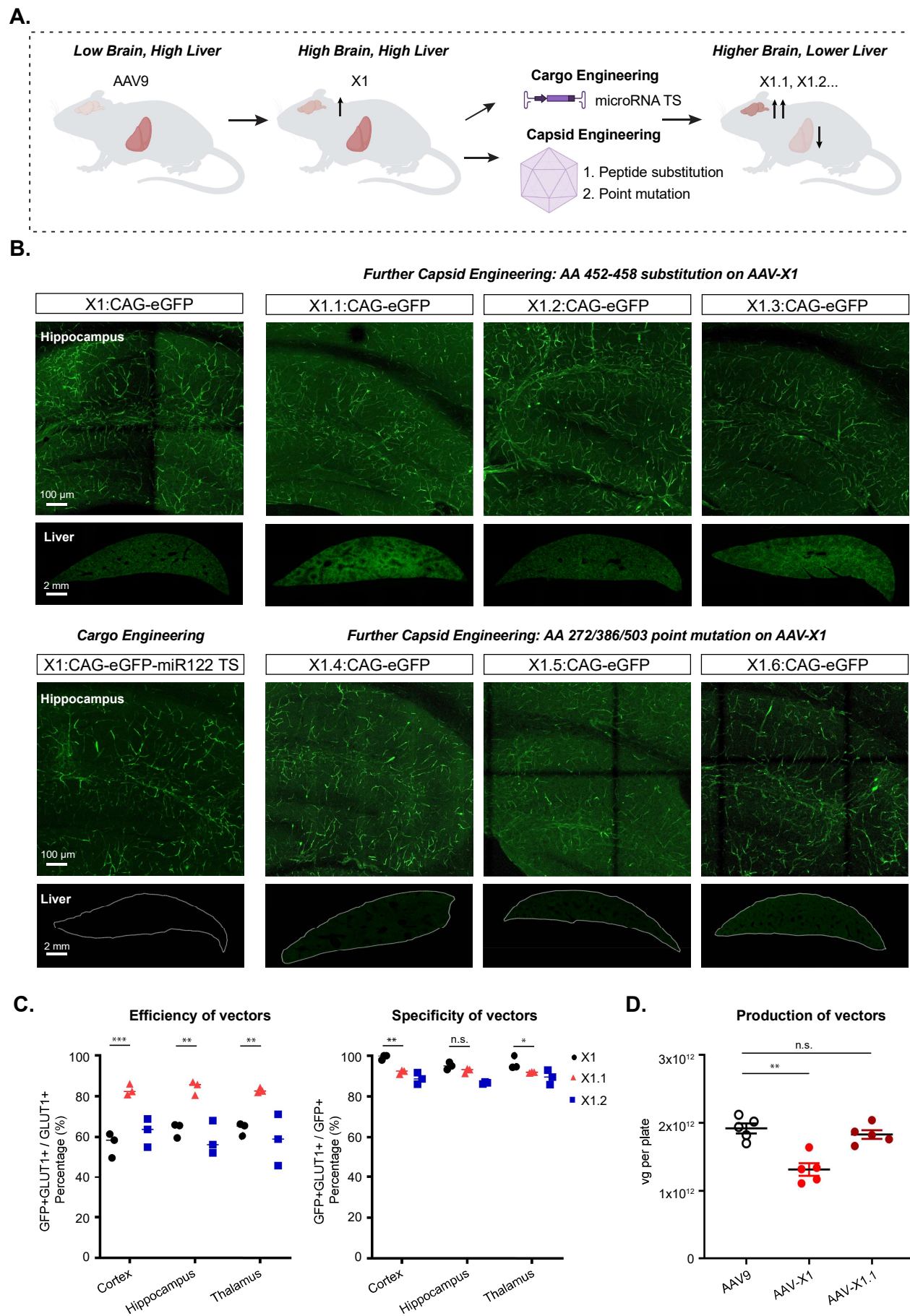
Figure 2: Semi-rational refinement of X1 capsid's tropism by further cargo and capsid engineering.
