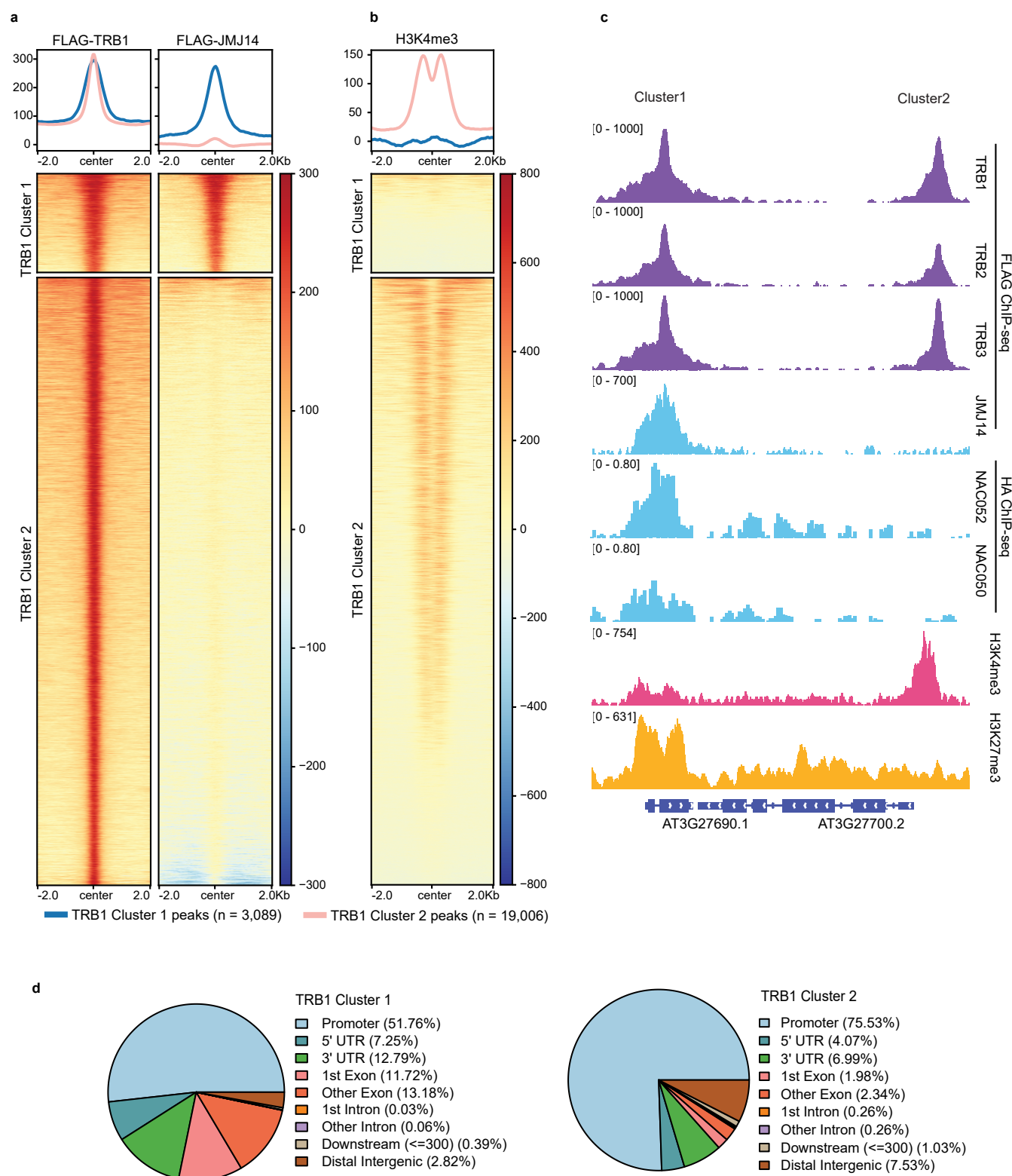
Fig. 2 TRB1 peaks overlap with JMJ14 peaks at H3K4me3 depleted regions. a-b Heatmaps and metaplots showing ChIP-seq signals of FLAG-TRB1 ( a , left panel), FLAG-JMJ14 ( a , right panel), and H3K4me3 ( b ) over TRB1 Cluster 1 peaks (n=3,089) and Cluster 2 peaks (n=19,006) respectively. c Screenshot displaying the ChIP-seq signals of FLAG-TRB1, FLAG-TRB2, FLAG-TRB3, FLAG-JMJ14, HA-NAC052, HA-NAC050, H3K4me3, and H3K27me3 over a representative locus containing TRB1 Cluster 1 and Cluster 2 peaks. d Pie Charts depicting the annotations of the TRB1 Cluster 1 peaks (left panel) and Cluster 2 peaks (right panel).
