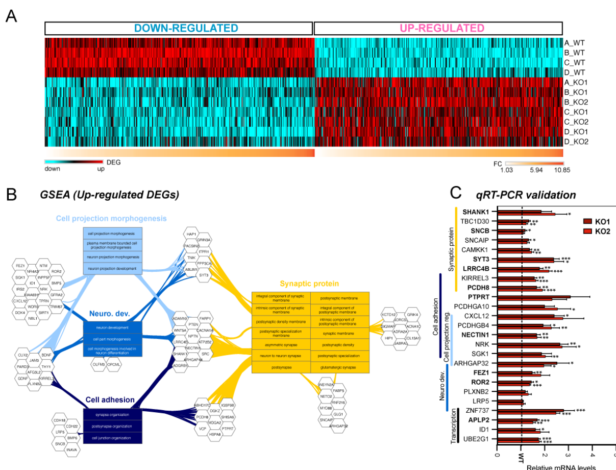
Figure 2. Differential gene expression analysis in d7 CASK KO immature iNs using bulk RNA-sequencing. (A) Heatmap showing both up- and down-regulated DEGs across independent culture replicates (4 replicates for WT & KO#1, 3 replicates for KO#2). Cutoff for DEGs was set at FC \geq 1.2 or \leq 0.8 , p < 0.05 ; minimum of 5 TPM per gene). A total of 876 shared DEGs were identified in CASK KO#1 and KO#2, as compared to WT control, with 420 genes upregulated and 456 genes downregulated. (B) Gene set enrichment analysis (GSEA; ToppCluster) of commonly upregulated DEGs (Bonferroni p < 0.05 ) identified 3 major biological pathways (BP; cell projection morphogenesis p < 9.60E-07 ; neurodevelopment p < 1.26E-05 ; cell adhesion; p < 5.85E-06 ) and 1 cellular component (CC; postsynapse; p < 2.01E-08 ) affected by CASK LOF. (C) qRT-PCR validation of specific up-regulated DEGs for both KO#1 and KO#2 relative to WT (set to 1). GAPDH probe was used as a normalization control. Bolded probes indicate genes cross-referenced with SynGO. Four independent replicates per genotype were validated, and each qRT-PCR experiment was performed in triplicate for 26 upregulated DEGs. qRT-PCR data represents means \pm SEM, and statistical analysis was performed using Student's t-test comparing WT to each individual KO (* P < 0.05 , ** P < 0.01 , *** P < 0.001 ; nonsignificant comparisons are not indicated).
