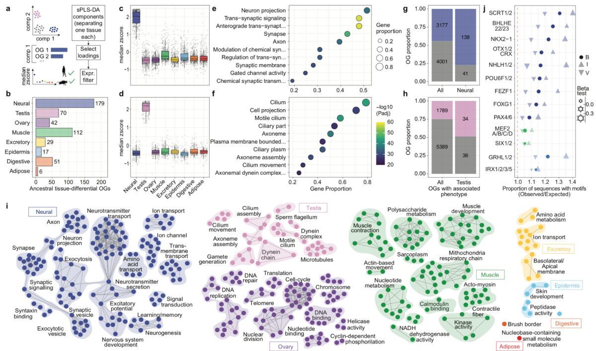
Fig. 2: Reconstruction of ancestral bilaterian tissue-differential expression modules. a. Scheme depicting the procedure for the definition of the ancestral tissue-differential modules. We performed an sPLS-DA on the expression of the ancestral bilaterian best-hits orthogroups, where each component specifically separated the meta-samples of one tissue group from all the others. We selected loadings of each component, which corresponded to orthogroups with the most distinctive expression profile in the isolated tissue compared to the rest. Finally, we required these orthogroups to show the highest median expression (after z-scoring expression within each species) in that particular tissue among both vertebrates and insects. b: Number of orthogroups included in each ancestral tissue-differential module. c,d. Expression profiles across tissues of best-hits orthogroups in the ancestral neural- (c) and testis- (d) differential modules. Expression values were first z-scored by species, and each dot represents the median expression among vertebrates, insects or outgroups. e,f. Top 20 most significantly enriched GO categories in the ancestral neural- (e) and testis- (f) differential modules. Only GOs containing at least 5 genes in the tested set were considered. g,h: Proportion of all bilaterian-conserved orthogroups (left) and ancestral neural (g) or testis (h) modules (right) associated with experimentally validated phenotypes (in the respective tissue) in mammals and/or fruit fly. i: Representation of GO networks of significantly enriched categories for all ancestral tissue-differential modules, where only categories containing at least 5 genes in the tested set were considered (see Methods). j. TFs included within each tissue-differential module whose known
