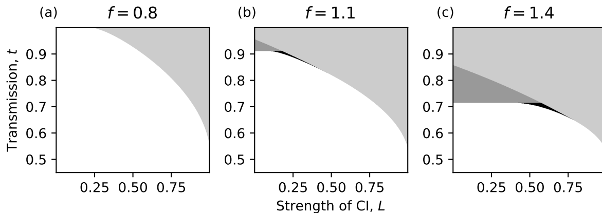
Figure 4. Properties of equilibria of the diplodiploid model shown across parameter space. The parameter regions are categorized as featuring only the trivial equilibrium at p = 0 (white), a non-trivial stable equilibrium \hat{p}_2 > 1/2 with or without invasion threshold (light grey), and non-trivial stable equilibrium \hat{p}_2 < 1/2 without (dark grey) or with (black) an invasion threshold. Values of parameter f (fecundity) are indicated above each panel.
