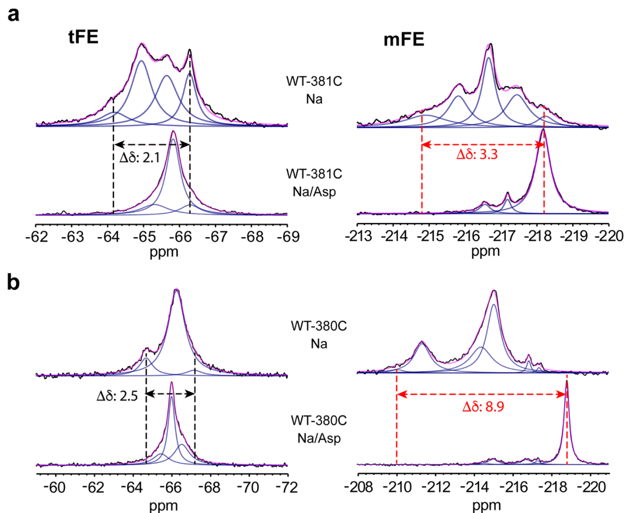
Extended Data Fig. S3. Comparison of chemical shift dispersion of tFE- and mFE-labeled Glt Ph variants. 19 F NMR spectra of WT-A381C (a) and WT-A380C (b) labeled with tFE (left) and mFE (right). Shown are spectra in the presence of 400 mM Na + (upper panel) and 100 mM Na + and 2 mM Asp (lower panel). All spectra were recorded at 25 °C. \Delta\delta indicates the largest observed chemical shift difference in ppm.
