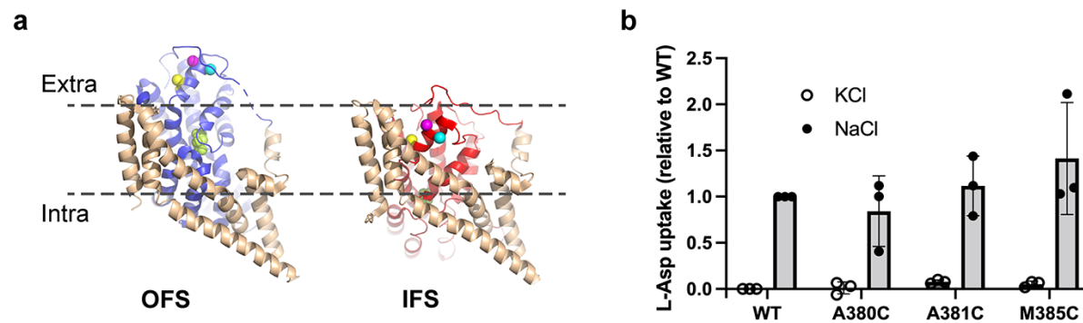
Extended Data Fig. S1. Labeling positions and ^3\text{H} -aspartate uptake assay. (a) Cysteine mutations introduced into Glt Ph : A380C (magenta), A381C (cyan), and M385C (yellow). A single protomer in the outward-facing state (OFS, left) and inward-facing state (IFS, right) is shown in cartoon representation with scaffold domain colored wheat and transport domains blue and red, respectively. Bound substrate Asp is shown as lime-colored spheres. (b) ^3\text{H} -Asp uptake assay of WT Glt Ph and mFE-labeled single-cysteine mutants (see Methods). Shown are initial ^3\text{H} -Asp uptake rates (measured at 2 min) of mFE-labeled Glt Ph variants relative to an unlabeled cysteineless WT Glt Ph . Data was normalized to WT uptake in the presence and absence of sodium gradients (closed circles and open circles, respectively). Experiments were repeated in triplicates on independently prepared protein samples.
