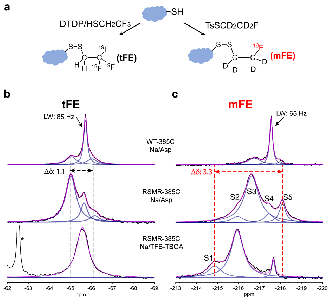
Figure 1. mFE-labeled Glt Ph variants show wide chemical shift dispersion. (a) Site-specific Glt Ph protein labeling (see Methods for details). (b, c) ^{19}\text{F} NMR spectra of Glt Ph -M385C variants labeled with tFE (b) and mFE (c). Shown are from top to bottom: WT and RSMR mutant in 100 mM \text{Na}^+ and 2 mM aspartate (Asp), and RSMR mutant in 100 mM \text{Na}^+ and 0.6 mM TFB-TBOA. All spectra were recorded at 25 °C. Asterisk denotes signal from the \text{CF}_3 group of TFB-TBOA. S1-S5 denote resolved resonance peaks observed using the mFE probe, and \Delta\delta is the largest observed chemical shift difference. All ^{19}\text{F} NMR spectra here and elsewhere were recorded at least twice on independently prepared protein samples, producing similar results.
