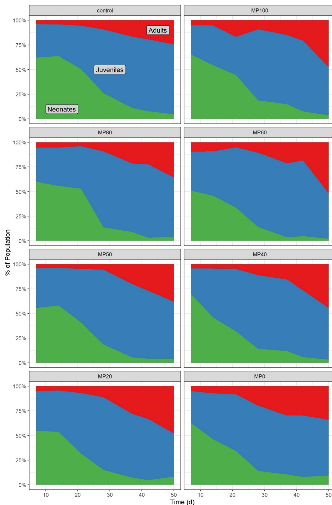
Figure 3: Population structure of Daphnia magna exposed to polystyrene microplastics (MP100), diatomite (MP0), or their mixtures over 50 d. Data presented as mean relative ratios of neonates (green), juveniles (blue), and adults (red) compared to the overall population density (n = 3).
