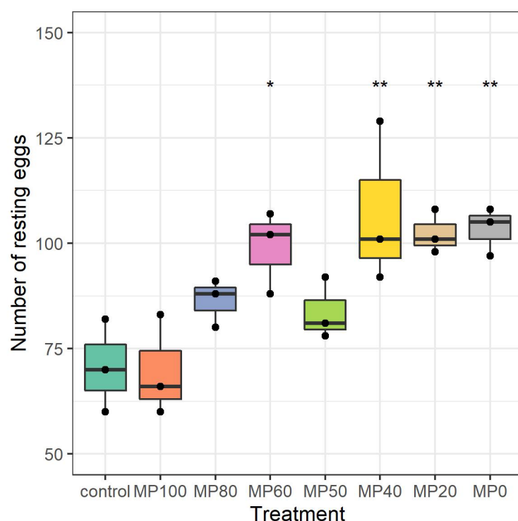
Figure 2: Total number of resting eggs produced by Daphnia magna populations exposed to polystyrene microplastics (MP100), diatomite (MP0), or their mixtures over 50 d ( n = 3 ). Significant differences compared to control populations are indicated by asterisks: * p < 0.05 , ** p < 0.01 .
