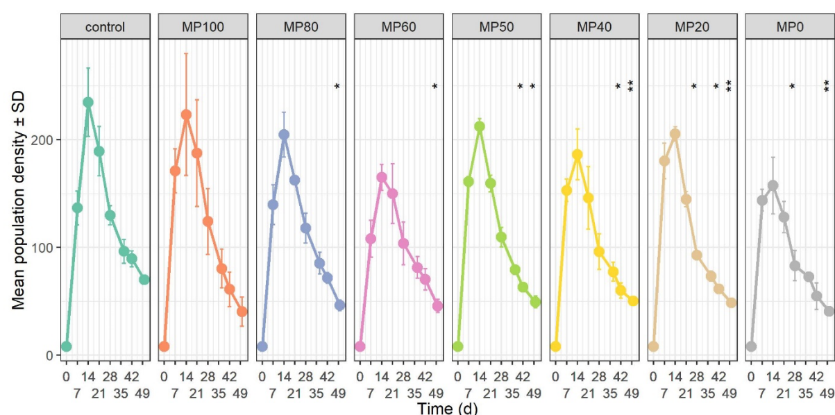
Figure 1: Mean population density of Daphnia magna exposed to polystyrene microplastics (MP100), diatomite (MP0), or their mixtures over 50 d. The error bars represent the standard deviation, significant differences compared to control populations are indicated by asterisks: * p < 0.05 , ** p < 0.01 .
