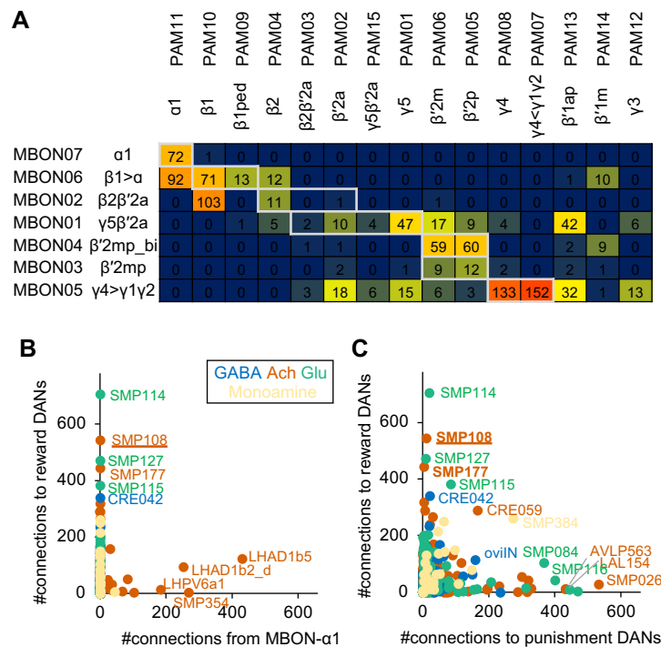
Figure 3-figure supplement 1 Connections of MBON- \alpha 1 and SMP108
