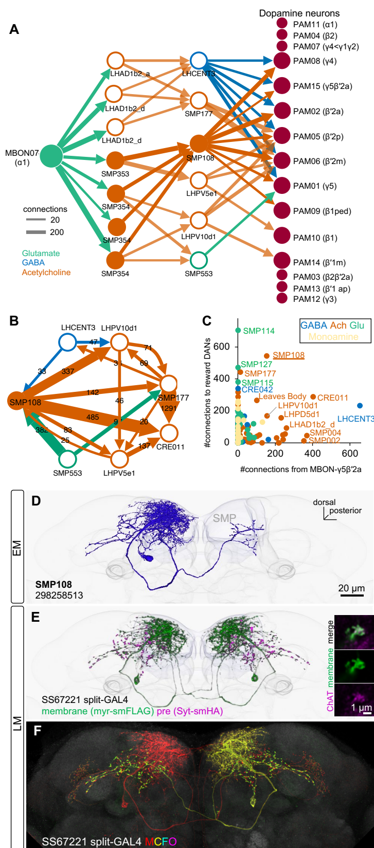
Figure 3 SMP108 is a key interneuron between MBON-α1 and DANs
