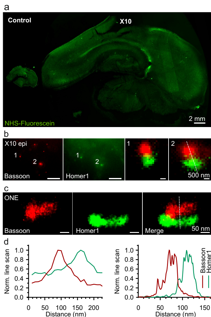
Extended Data Fig. 9. ONE analysis of brain slices. a , Images of a 200 \mu m-thick rat brain section before (left) and after (right) expansion, relying on autoclaving for homogenization 69 . The scale bar does not take the expansion factor into consideration. The sections were labeled by using NHS-ester fluorescein incubations. b , Epifluorescence images of expanded brain slices, focusing on Bassoon and Homer1 as pre- and postsynaptic markers, respectively. c , Similar images, taken using the ONE procedure. d , Line scans executed over the areas indicated in panels b and c. As expected, far more detail can be observed in ONE than in simple epifluorescence microscopy.
