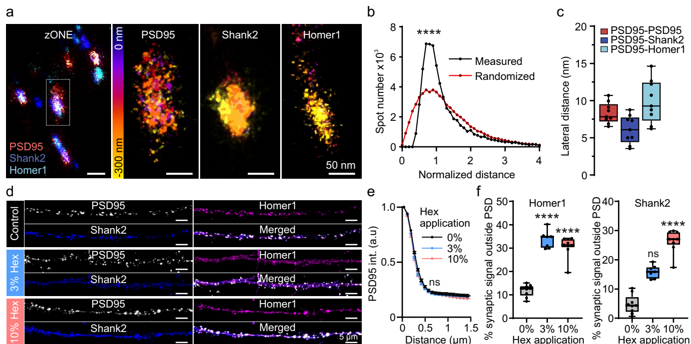
Extended Data Fig. 7. A detailed analysis of the PSD. a , The PSD was immunostained for PSD95, Homer1 and Shank2, as in Fig. 3, and images were taken at different heights along the Z-axis (zONE imaging). An overlay (summed image) is shown in the left panel, along with an analysis of the proteins at different Z levels, using a colormap that describes the positions along the Z axis (right panel). b , The distance between PSD95 spots was computed from images as in panel a, and was compared to that obtained from positioning the molecules randomly within the PSD95, N = 10 synapses, Friedman test followed by Dunn-Sidak, p=0.0001 . c , The lateral distance between PSD95 spots and between PSD95 and Homer1 or Shank2. The minimal distance between each PSD95 spot and a Homer1/Shank2 spot is shown (measured in the lateral plane, in 2D projections of the PSD). N = 10 synapses, from 2 independent experiments. While the distance between PSD95 spots has a non-random character, as indicated in panel b, the distances to Homer1 or Shank2 spots are not different from randomized distributions (Dunn-Sidak tests, p > 0.1 ), possibly also because these two molecules are immunostained using antibodies, which causes the fluorescence signals to scatter broadly. d , Confocal microscopy analysis of the PSDs, in non-expanded samples. In control conditions all three components analyzed here (PSD95, Homer1, Shank2) are well colocalized. The addition of 3% 1,6-hexanediol (Hex) causes the dispersion of Homer1 (magenta), while 10% Hex also disperses Shank2 (blue). PSD95 remains largely unaffected by Hex. e , An analysis of the average PSD95 spot profile confirms this impression, N = 10 -7-10 neurons, a set from 3 independent experiments. f , We analyzed the dispersion of Homer1 (left) and Shank2 (right) away from the PSD95 spots. The signal present in synapses (near the PSD95 labeling, but not within the PSD) was analyzed, to determine the % that is not correlating to the PSD structure. The same samples were analyzed as in panel e.
