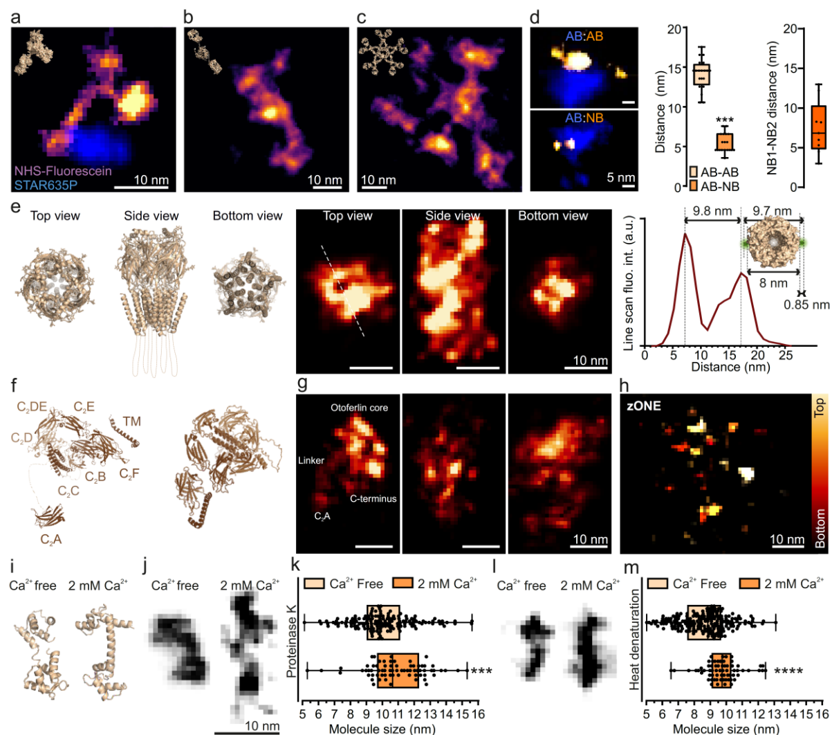
Figure 2. ONE analysis of single molecules. a-c , Images of isolated immunoglobulins (IgG, IgA, IgM), labeled with NHS-ester fluorescein after homogenization. The IgGs were secondary anti-mouse antibodies, carrying STAR635P (blue). d , Distances between fluorescently-conjugated IgGs and fluorescently-conjugated secondary antibodies (top) or secondary nanobodies (bottom). In panels a-d we used a different fluctuation analysis, termed temporal radially pairwise product mean, TRPPM, unlike the temporal radially auto-cumulant to the order of 4 (TRAC4) 6 approach used in most other figures. Unlike TRAC4, which aims to separate the individual fluorophores, TRPPM enhances the cohesiveness of the fluorophores decorating the single antibodies, resulting in cloud-like signals whose distances are easily measured (N = 20/19, for AB:AB/AB:NB). Right panel: distance between the two secondary nanobodies binding single IgGs (N = 9). e , A similar analysis of purified GABA A receptors. Line scans across specific profiles seem to detect the receptor pore. f , AlphaFold-derived structure of otoferlin. g , ONE examples of otoferlin images. h , Z-axis ONE imaging, indicating that two components (presumably C 2 A and TM domains) are relatively far from the main body of the molecule. i , PDB structures of the Ca 2+ sensor calmodulin, in presence or absence of its ligand, along with ONE images, after proteinase K-based homogenization and expansion (see Supplementary Fig. 6 for more images). j , The expected elongation by ~1 nm was reproduced ( p = 0.0006 , Mann-Whitney test; N = 70-155). k-l , Similar analysis, after homogenization using autoclaving ( p < 0.0001 , N = 66-197). The box plot shows the medians, the 25 th percentile and the range of values. m , Heat denaturation analysis.
