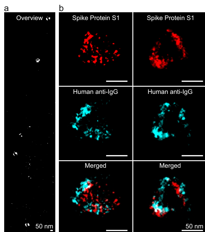
Supplementary Fig. 10. ONE analysis of SARS-CoV-2 viral particles. a , ONE overview of a sample containing SARS-CoV-2 viral particles immunostained against Spike Protein S1. b , More detailed views of two particles, indicating the Spike Protein S1 and the native IgG molecules from the serum of the patients. Interestingly, a domain-like structure is observed, which is presumably induced by the native IgGs gathering the spike proteins together, by the dual binding capacity of the IgG molecules.
