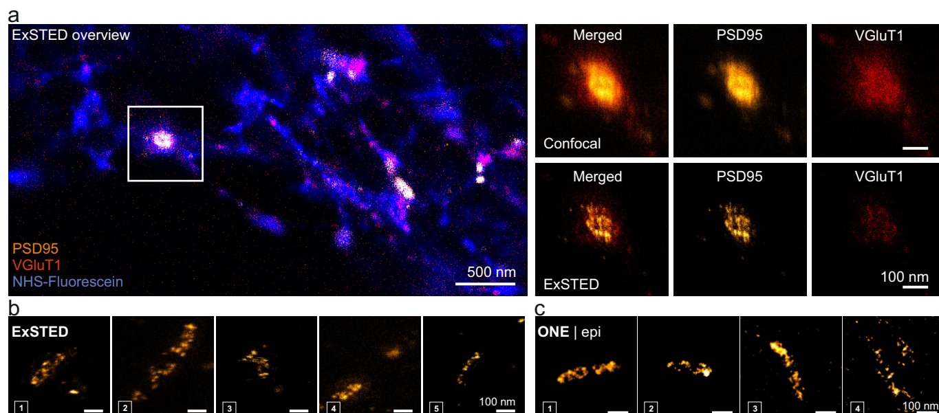
Extended Data Fig. 8. ExM-STED (ExSTED) imaging of PSDs. a , Hippocampal cultures were immunostained for PSD95 and VGluT1, and were additionally labeled with NHS-ester fluorescein, after homogenization. b , A gallery of high-zoom ExM-STED views of synapses, with a focus on PSD95. Relatively large PSD domains are visible, as in most previous works in the literature, and unlike most of our ONE images. c , To determine if this is simply an issue of resolution, we aimed to generate ExM-STED-like images with ONE microscopy, by reducing its resolution. We employed an epifluorescence microscope (as opposed to a rapidly scanning confocal in the panels dealing with PSD95 in Fig. 3), and we used the temporal radially pairwise product mean (TRPPM) option of analysis, which broadens the resulting spots. The results are very similar to ExM-STED images, demonstrating that the modular/domain appearance of the PSD95 stainings is a result of insufficient resolution, with a reticulum being evident only at very high resolution (under optimal ONE imaging).
