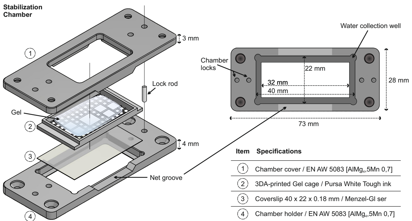
Supplementary Fig. 2. Technical scheme of the stabilization chamber used in this work. The exact measurements and materials for the stabilization chamber are included in the figure text. The 3D-printed gel cage patterning can be organized according to the user's preferred design. Only a suggested design is included here (many others work equally well).
