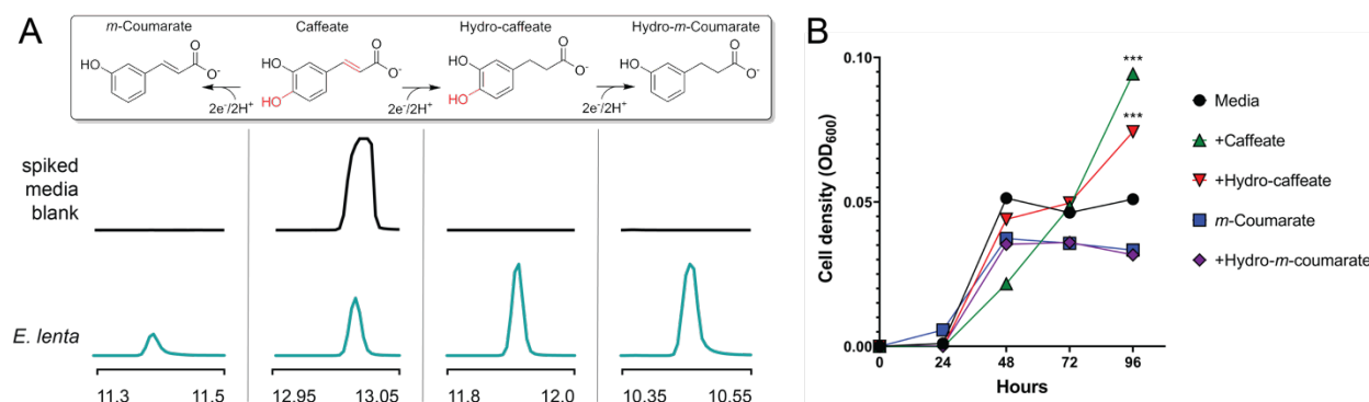
Figure S7. Caffeate utilization by E. lenta . (A) GC-MS analysis of supernatant collected from E. lenta DSM2243 grown in caffeate-spiked media. Proposed reaction pathways are shown, with peaks for each compound provided beneath its chemical structure. The previously characterized hydrocaffeate dehydroxylase may catalyze the observed dehydroxylation reactions. The observed caffeate reduction to hydrocaffeate provides evidence of a caffeate reductase, while the accumulation of m -coumarate suggests that this enzyme may specifically use caffeate. (B) E. lenta DSM2243 growth in media supplemented with formate and different cinnamates. The pattern of cinnamate-dependent growth enhancement supports the conclusions that: (1) dehydroxylation can support respiratory growth and (2) m -coumarate is a poor electron acceptor for E. lenta . Data are mean (n = 3). *p < 0.05, **p < 0.01, *** p < 0.001. Two-way ANOVA, multiple test vs media alone.
