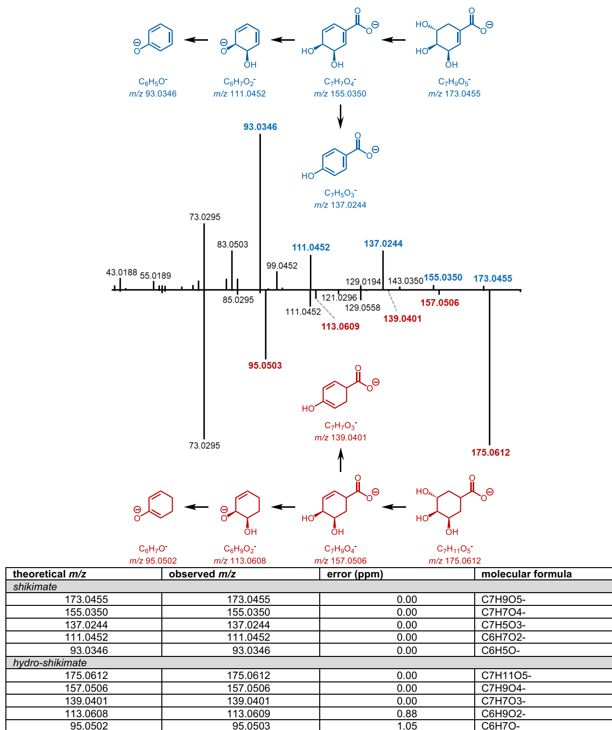
Figure S11. Butterfly plot of LCMS-MS fragmentation spectra for shikimate at top with key putative fragment ions highlighted in blue and hydro-shikimate at bottom with key putative fragment ions highlighted in red. The difference in two Dalton between the key putative fragments in these spectra support the assignment of m/z 175.0612 as hydro-shikimic acid as shown.
