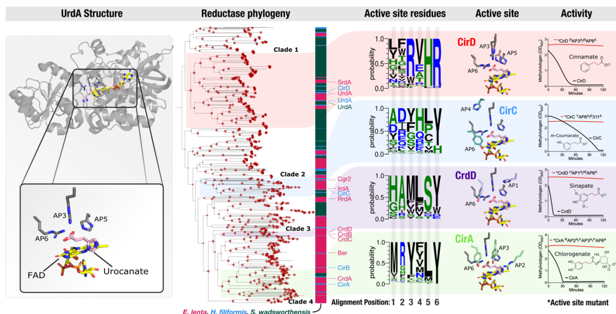
Figure 5. Independent evolutionary trajectories and distinct active sites distinguish flavin reductases with related electron acceptors. UrdA structure – crystal structure of urocanate- and FAD-bound UrdA (PDB code 6T87). Reductase phylogeny – phylogenetic tree of flavin reductases from E. lenta , S. wadsworthensis , and H. filiformis genomes. Bootstrap support values are indicated by the size of red dots at nodes of the tree and range from 70 to 100. Active site residues – representation of sequence identity of active site amino acids in reductase clades 1–4 scaled to frequency within the multiple sequence alignment. Positions within the multiple sequence alignment have been renumbered to active site alignment position (AP). Active site – AlphaFold models of CirD, CirC, CrdD, and CirA cinnamate reductases superimposed to the UrdA crystal structure. Activity – reductase activity of CirD, CirC, CrdD, and CirA and active site point mutants (indicated by an asterisk). Active site mutations and alignment positions they correspond to: *CrdD H313A (AP1) and W510A (AP6); *CirA R417A (AP2), Y469A (AP3), and Y634A (AP6); *CirC E311A and Y511A (AP6); *CrdD R542A (AP3) and R716A (AP6). The y-axis shows the amount of reduced methylviologen in the presence of the indicated electron acceptor.
