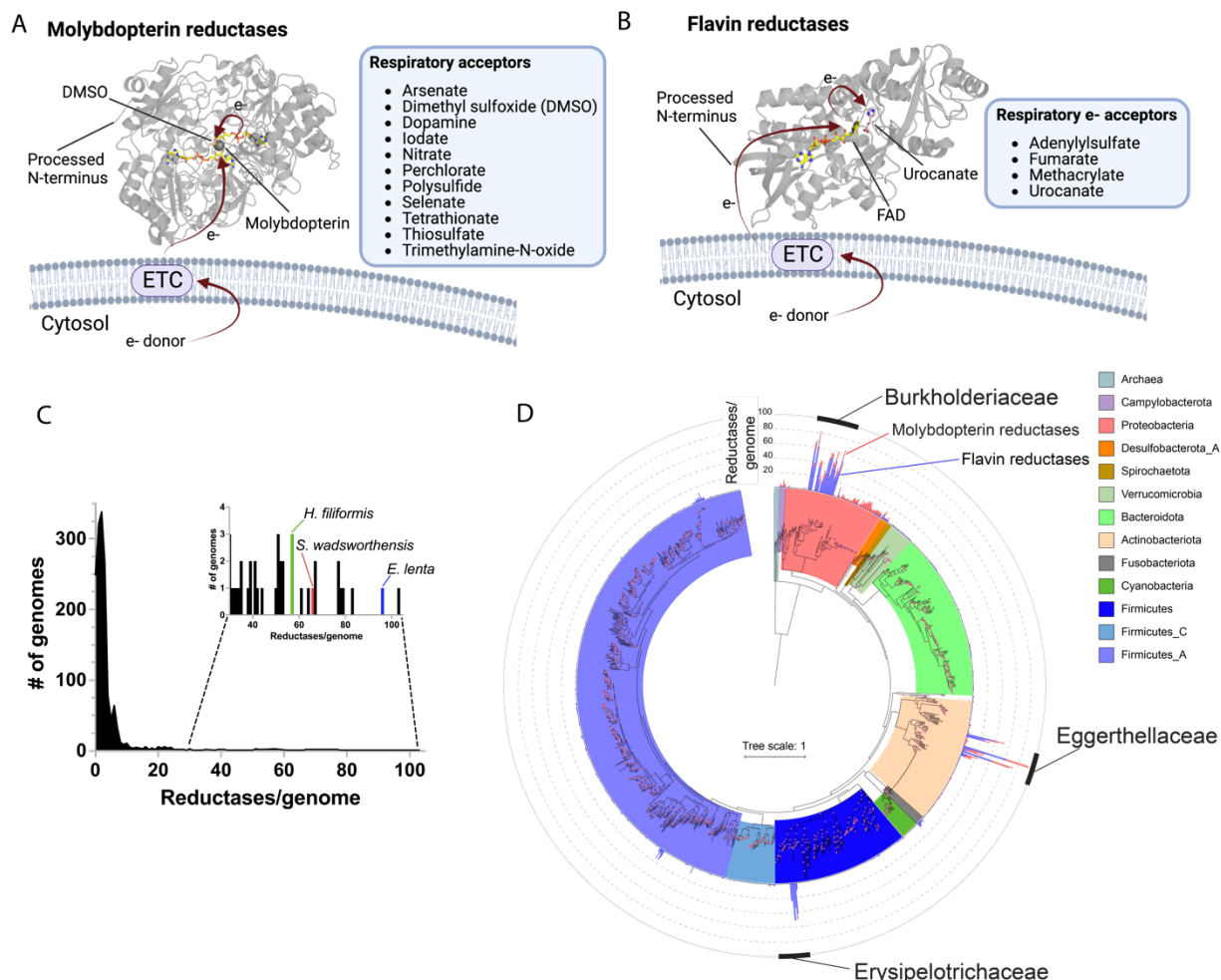
Figure 1. Respiratory reductase orthologs are highly overrepresented in three distinct lineages of gut bacteria. (A) General mechanism and electron acceptors used by different previously characterized respiratory molybdopterin reductases (Pfam PF00384). Arrows highlight electron (e-) transfer path from the electron transport chain (ETC) to dimethylsulfoxide (DMSO) in the DMSO reductase crystal structure (PDB code 4DMR). (B) Electron acceptors and general electron transfer mechanism used by previously characterized respiratory flavin reductases (Pfam PF00890). Arrows highlight electron transfer to substrate in the urocanate reductase co-complex crystal structure (PDB code 6T87). (C) Distribution of the number of flavin/molybdopterin reductases in 1533 representative human gut bacteria genomes and metagenomes genomes. (D) Phylogenetic reconstruction of the evolutionary history of these reductases. The maximum likelihood tree was constructed based on a concatenated alignment of 14 ribosomal proteins under an LG + I + G4 model of evolution (2092 amino acid sites). The number of flavin (blue) and molybdopterin (red) reductases with a computationally predicted signal peptide in each genome are graphed on the outer ring of the tree.
