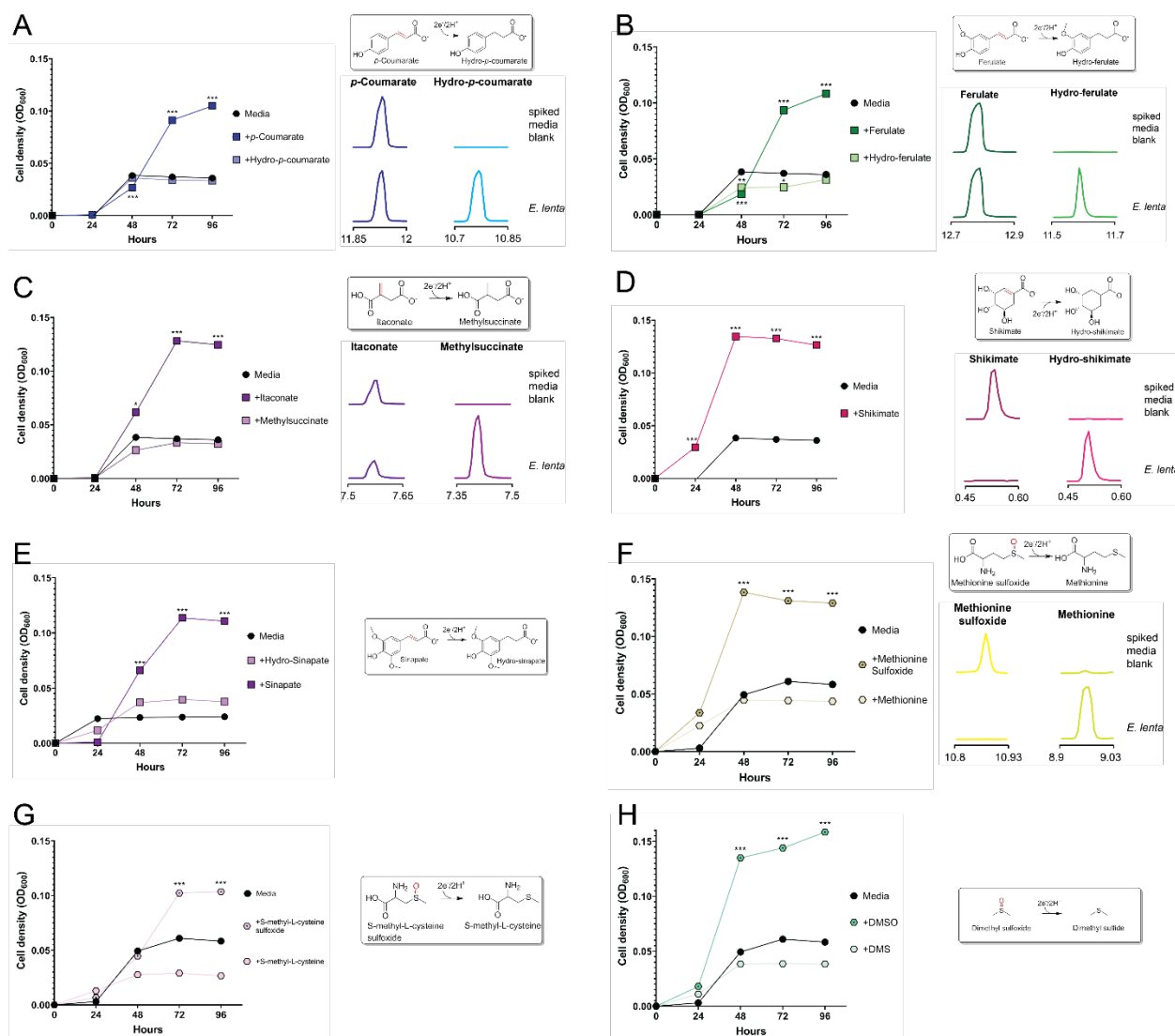
Figure S3. E. lenta uses multiple respiratory electron acceptors. E. lenta DSM2243 growth in formate-supplemented media provisioned with electron acceptors: (A) p -coumarate, (B) ferulate, (C) itaconate, (D) shikimate, (E) sinapate, (F) methionine sulfoxide, (G) S-methyl-L-cysteine sulfoxide, and (H) dimethyl sulfoxide. A 'no electron acceptor' condition and conditions with predicted reduction products are included as controls. GC- or LC-MS analyses show peaks for electron acceptors and their reduced products in uninoculated and inoculated growth media. (A), (B), (C), (E) were measured by GC-MS; (D) was measured by LC-MS; support for identification of hydro-shikimate in (D) is provided in Figure S11 . Data are mean (n = 3). *p < 0.05, **p < 0.01, *** p < 0.001. Two-way ANOVA, multiple test vs media alone.
