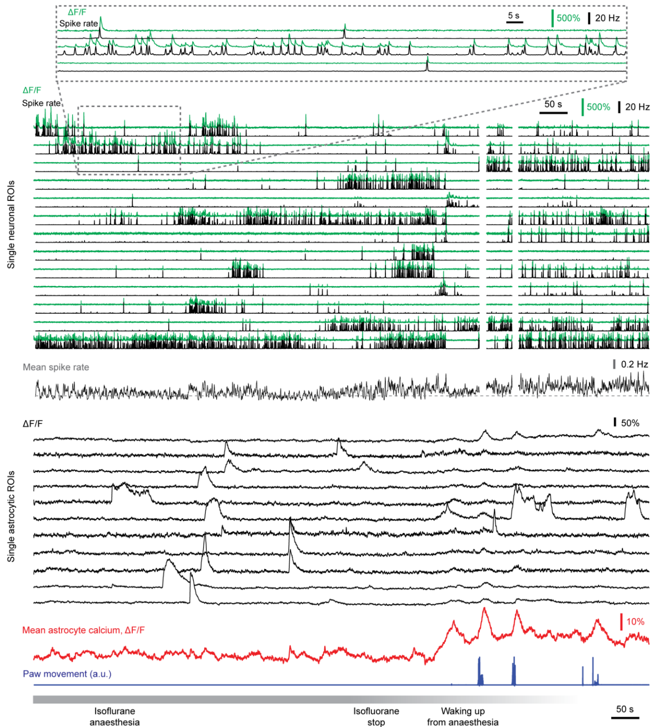
Figure S5 | Calcium imaging of astrocytes and pyramidal neurons in CA1 during isoflurane anesthesia. Examples of extracted neuronal \Delta F/F traces (green) and associated deconvolved spike rates (black) are shown (see also zoom-in at the top). White blanked time points were discarded due to excessive movement of the brain during the waking-up. Example astrocytic \Delta F/F traces (black) are shown below, highlighting uncoordinated local but no global events before the waking up. Waking up (bottom; 1.5% in the beginning, set to 0% at “isoflurane stop”) is reflected by small and large paw movements (blue) and resulted in global astrocytic calcium signals (mean astrocytic calcium, red).
