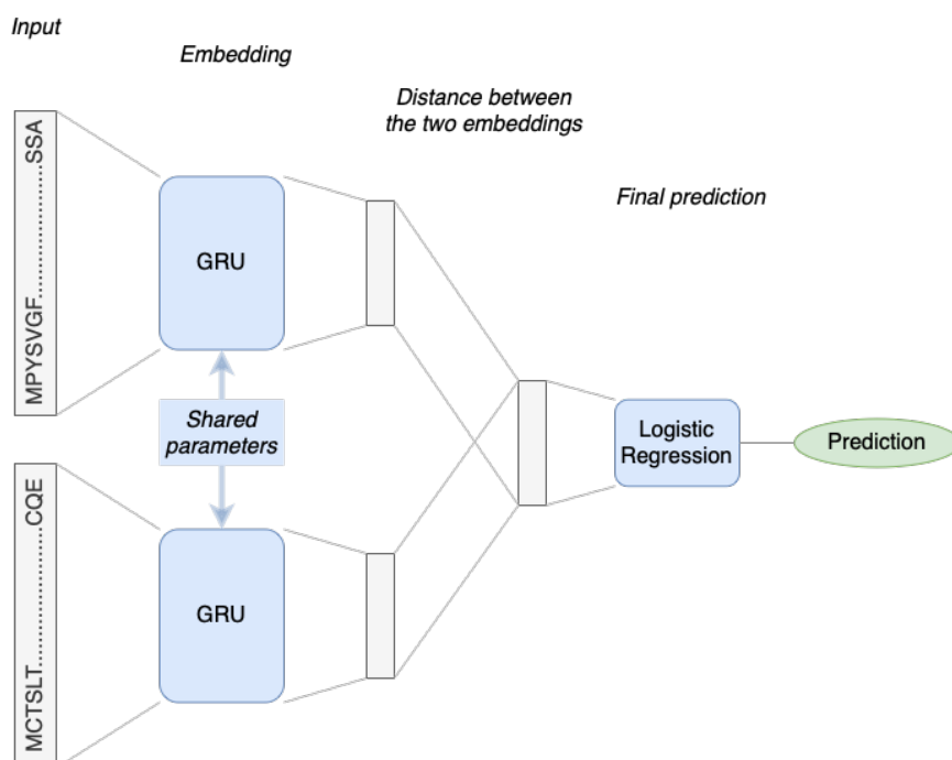
Figure 9: Diagram of the deep learning architecture used to predict interactions from a pair of protein sequences.
