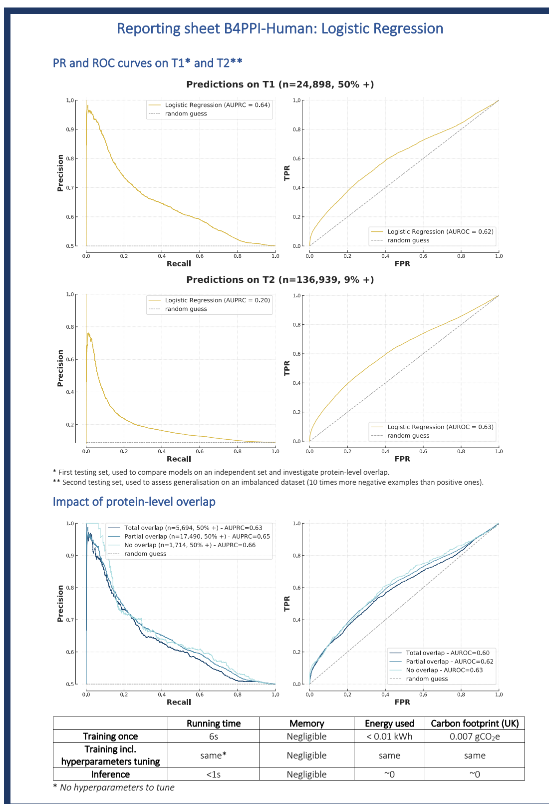
Figure 1: Reported performance sheet of the logistic regression (FG-based) on B4PPI-Human.
