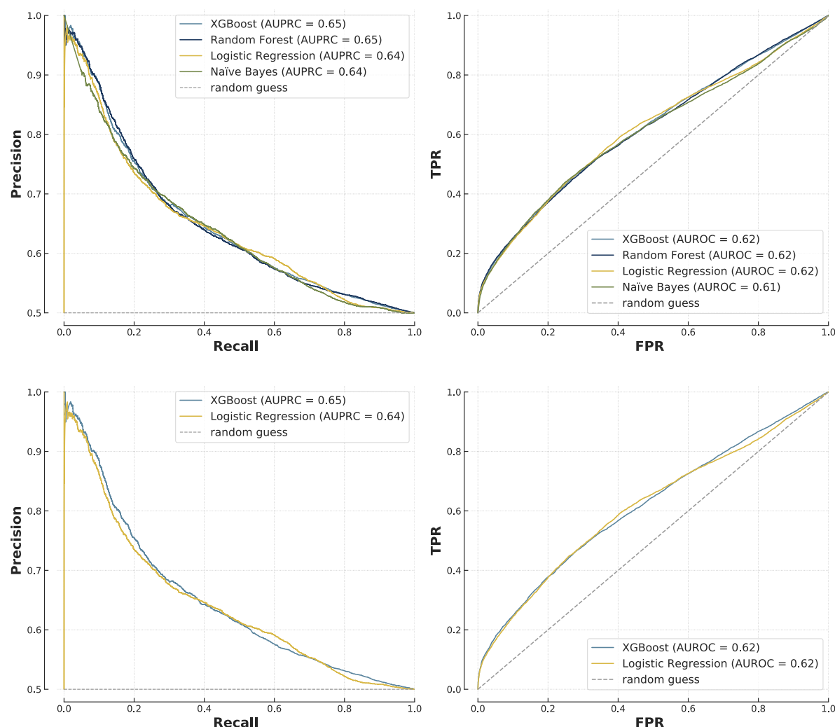
Figure 3: Comparison of FG-based models on T1 (n=24,898, 50% positive), with PR curves (left) and ROC curves (right) for all the models tested (top) and then only XGBoost and Logistic Regression for clarity (bottom).
