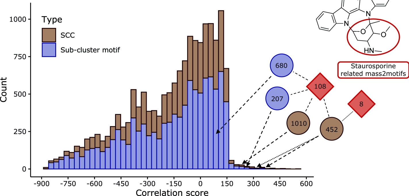
Correlation scores between mass2motifs and the two sub-cluster types
