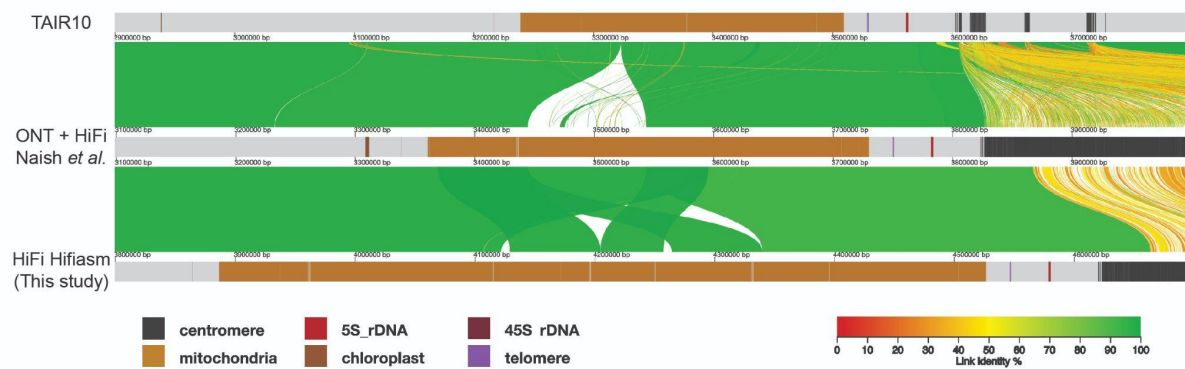
Supplementary Figure 9. Alignment of multiple assembly versions of the mitochondrial DNA insertion downstream of the centromere in Chromosome 2 in Col-0 visualized by AliTV (35). Co-linear horizontal gray bars represent portions of the TAIR10 reference genome ( top ; (1)), the assembly from Naish et al. ( middle ; (18)) and our HiFi-Hifiasm assembly of Col-0 ( bottom ), with sequence annotated as repetitive elements (centromeres, 5S and 45S rDNAs, telomeres, mitochondrial and chloroplast nuclear insertions) displayed as shades. Distance between ticks equals 100 kb. Colored ribbons connect corresponding regions in the alignment.
