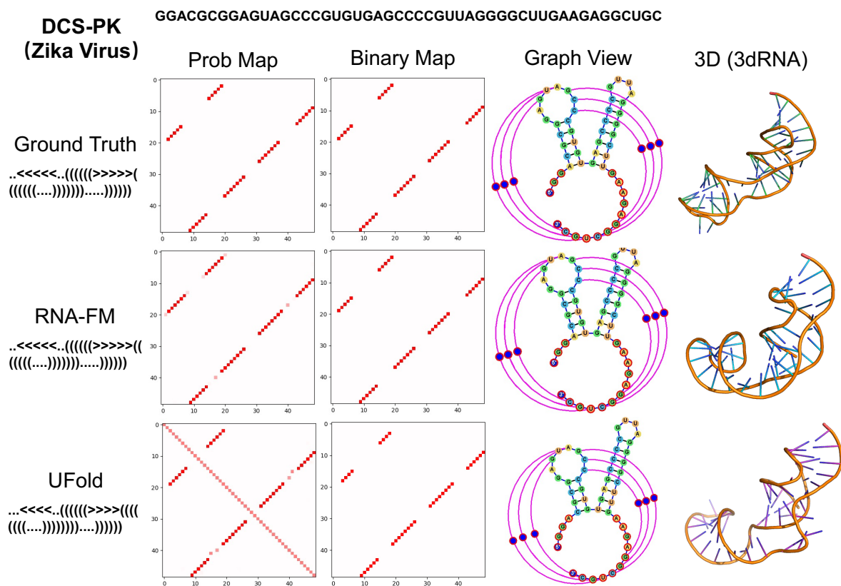
Appendix Figure 10: 3D reconstruction of RNA. The probability maps and binary maps are generated by different predictors. The graph views are obtained by jViz.Rna 4.0 [50]. The 3D structures are modelled by 3dRNA. a. An instance from PDB (5m73-1-A). b. The DCS-PK of Zika Virus.
