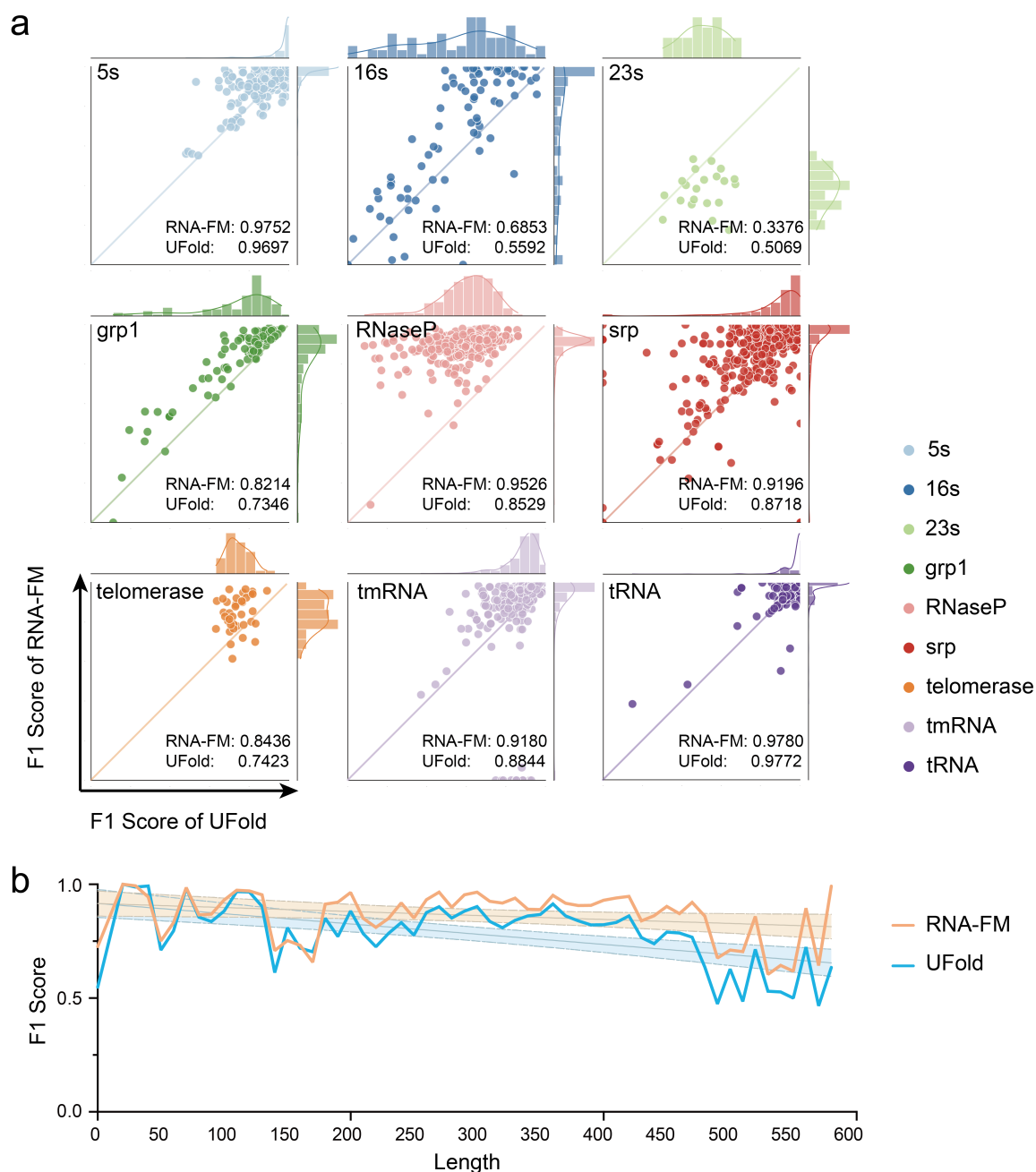
Appendix Figure 7: Detailed performance comparison between RNA-FM and UFold on the ArchiveII dataset. The experiment is cross-dataset validation of the trained model without re-training on ArchiveII. a. Scatter plots of F1 score comparison across 9 RNA types, with the performance of RNA-FM as the y-axis and that of UFold as the x-axis. Each point represents an RNA structure. Almost all the points are above the diagonal, which means RNA-FM beats UFold on nearly all the instances. b. F1 scores as a function of RNA sequence lengths. RNA-FM always outperforms UFold across all the lengths, especially when the length is over 150.
