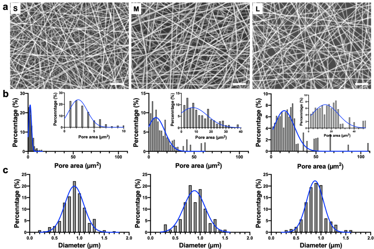
Fig. 2. Characterization of electrospun nanofibrous membranes. (a) Scanning electron micrographs (SEM) of nanofibrous membranes of small (S), medium (M), and large (L) pore sizes. Scale bars: 20 \mu\text{m} . (b) Pore size distributions of these nanofibrous membranes. The insets magnify the main pore size distributions. (c) Fiber diameter distributions of these nanofibrous membranes.
