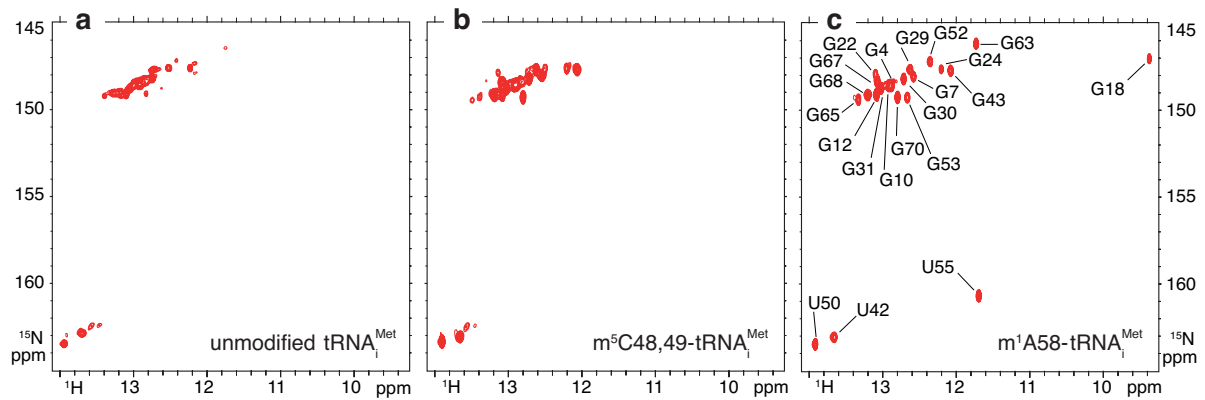
Figure 4: Effect of m 5 C48,49 and m 1 A58 on the structural properties of yeast tRNA i Met Imino ( 1 H, 15 N) correlation spectra of 15 N-labelled tRNA i Met with different modification status measured at 38°C. (a) unmodified tRNA i Met , (b) m 5 C48,49-tRNA i Met , and (c) m 1 A58-tRNA i Met . The assignment of the imino resonances of the m 1 A58-tRNA i Met was obtained following standard methods.
