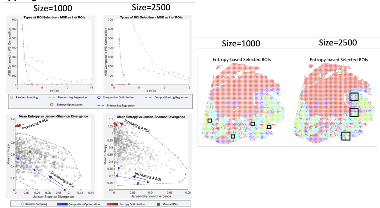
Supp. Figure 4: Optimization of ROI selection within a restricted set of cells. For two ROI sizes (1000 pixel, 2500 pixel) and three sampling techniques (random sampling, convex optimization using cell type composition, convex optimization using cell type composition, and regional entropy), we calculate the optimal selection of ROI. Before calculation, we restrict the cell types of interest to only tumor and immune type cells targeted by manual annotation. (Top row) By calculating the MSE for a range of ROI, we can evaluate each technique's rate and quality of convergence. (Middle row) Selections of representative ROIs are evaluated based on two metrics (Entropy for tissue heterogeneity and Jensen-Shannon Divergence for composition similarity.) Random sets of 7 ROIs are generated 1000 times to portray the baseline pattern. Selections from convex optimizations are plotted with increasing numbers of ROIs to show the change in performance. The performance of the manually selected ROIs is also shown to emphasize the bias in targeted sampling. (Bottom row) The optimal ROIs are shown for convex entropy optimization at each size of ROI. Image colors portray the XAE-labeled cell types (red being cell types not considered in this analysis).
