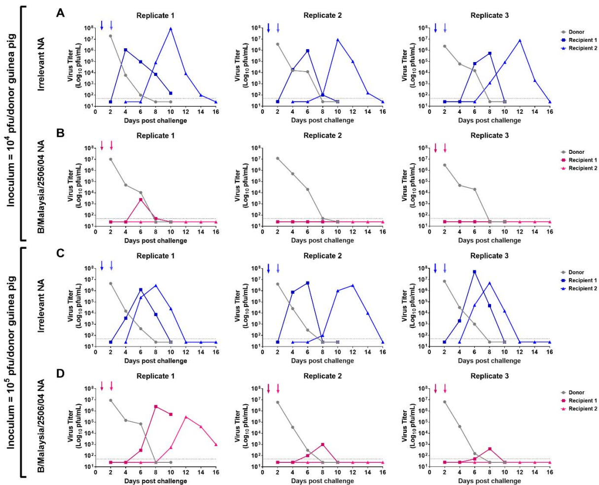
Figure 3. Assessment of B/Malaysia/2506/2004 transmission between vaccinated guinea pigs following a single day exposure to an infected donor.
