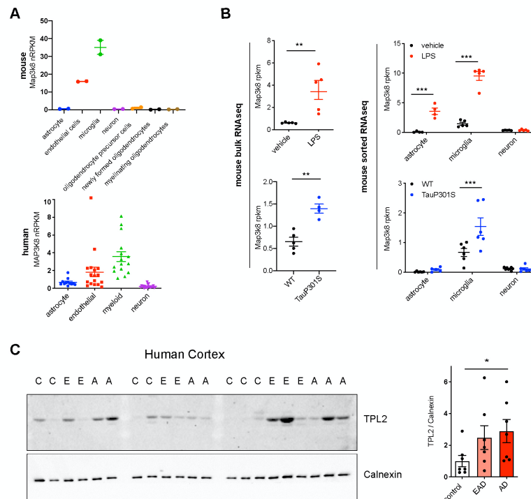
Fig. S1. TPL2 is upregulated in Tauopathy mice and AD patients.
