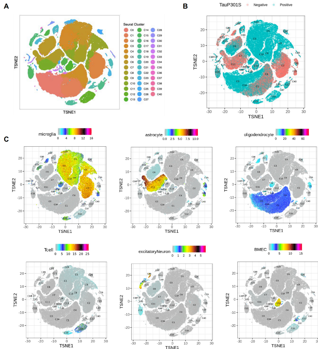
Fig. S6: Dimensional reduction and interpretation of cell clusters by gene set scores (related to Figure 5).
