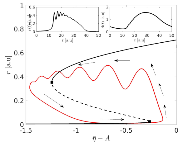
FIG. 3. Single neural mass with SFA The population firing rate r versus \bar{\eta} - A for the population burst solution displayed in 2 (b) (bottom). The solid (dashed) black lines refer to stable (unstable) fixed points of the fast sub-system (9a,9b,9c). The filled black squares denote the saddle-node bifurcations in the fast sub-system. The red solid line is the bursting solution of the complete system (9), where the black arrows indicate the time evolution along such a solution. In the upper insets are shown the population firing rate r(t) and the adaptation variable A(t) as a function of time during the evolution of the population burst. Parameters as in 2.
