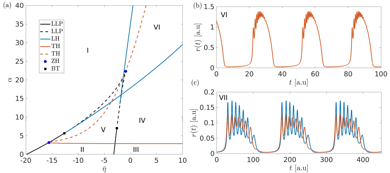
FIG. 9. Two symmetrically coupled excitatory populations with SFA a) Phase diagram in the (\bar{\eta}, \alpha) space showing 6 regions with different dynamics. Parameters for this diagram: J_c = 20 , J_s = 8 , \Delta = 0.5 , \tau_A = 10 and \tau_s = 2 . Regions I - V as in Fig. 6 (b). b) Region VI: symmetric bursting dynamics (\bar{\eta}, \alpha) = (5, 30) . c) An example of bursting with broken symmetry for parameters (\bar{\eta}, \alpha) = (23, 70) .
