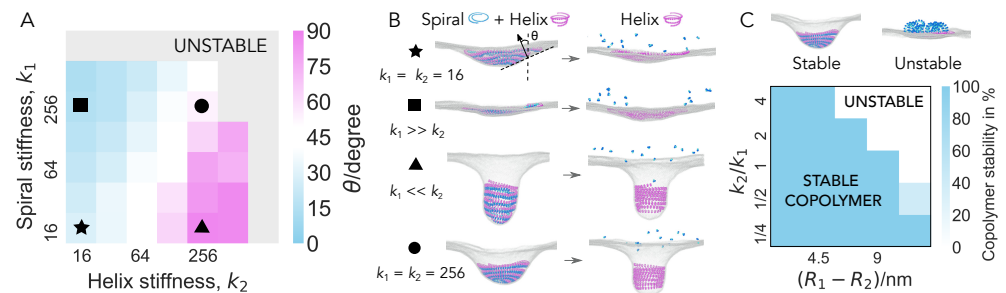
Fig 2. Relative filament stiffness controls the membrane deformation. A: Membrane deformation as a function of bond stiffness of the Flat Spiral ( k_1 ) and the Wide Helix ( k_2 ), ( k_1, k_2 are in units of k_B T / \sigma^2 , \sigma is the MD unit of length). The membrane deformation angle \theta is characterized by the angle between the vertical axis (normal to the original flat membrane plane) and the membrane normal at half depth of the deformation, as illustrated in the first snapshot in panel B. \theta = 0^\circ when the membrane is flat and \theta = 90^\circ when the membrane forms a tubule. Conical membrane deformations lie in between. The membrane deformation angle is calculated from the average of five independent runs. B: Representative simulation snapshots before and after the disassembly of the Flat Spiral, obtained for representative parameter sets as indicated by the matching labels in A. C: Copolymer stability as a function of the mismatch in the radius and ratio of stiffness between the Wide Helix and the Flat Spiral. Copolymer stability is quantified by a proportion of simulations in which the copolymerizing filaments remain attached to the membrane. The Flat Spiral is fixed at target radius R_1 = 19.4 nm with filament bond stiffness k_1 = 128 k_B T / \sigma^2 . All data points are averaged over ten simulations.
