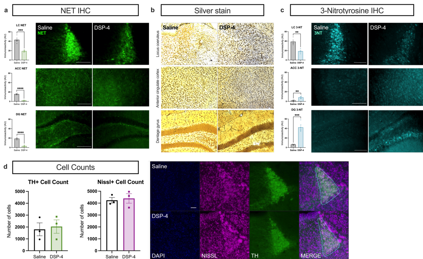
Fig. 2. DSP-4 induces degeneration of noradrenergic terminals and oxidative stress but leaves LC cell bodies intact. Mice received saline or DSP-4 (2 x 50 mg/kg, i.p.) and assessed for locus coeruleus (LC) neuron damage 1 week later. (a) DSP-4 results in substantial loss of axon terminals as measured by norepinephrine transporter (NET) immunoreactivity in the dentate gyrus (DG) and anterior cingulate cortex (ACC), with a similar decrease in NET also present in the LC itself. (b) Representative images of silver stained brain tissue indicates neurodegenerative processes in the LC, ACC, and DG following DSP-4. (c) The oxidative stress marker 3-nitrotyrosine (3-NT) was increased in the ACC and DG but decreased in the LC by DSP-4. (d) Despite NE fiber damage and the evidence of neurodegenerative and oxidative processes following DSP-4, LC cell body number was unaffected as measured by TH and NeuroTrace Nissl immunoreactivity. Data shown as mean \pm SEM. N=3-4 per group. ** p < 0.01 , *** p < 0.001 , **** p < 0.0001 .
