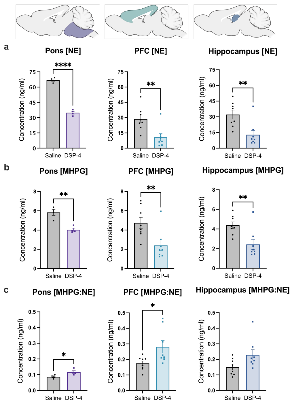
Fig. 1. DSP-4 decreases tissue NE and metabolite levels and increases turnover. Mice received saline or DSP-4 (2 x 50 mg/kg, i.p.), and tissue monoamine and metabolite levels were measured 1 week later by HPLC in the pons, prefrontal cortex (PFC), and hippocampus (color shaded images at top represent the approximate regions dissected for analysis). DSP-4 significantly decreased NE ( a ) and its primary metabolite MHPG ( b ) in all 3 brain regions. ( c ) NE turnover, defined as the MHPG:NE ratio, was increased in the pons and PFC by DSP-4, with a similar trend in the hippocampus. Data shown as mean \pm SEM. N=8 per group. * p <0.05, ** p <0.01, **** p <0.0001.
