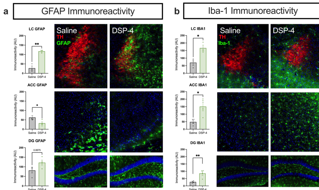
Fig. 3: DSP-4 alters astrocyte and microglia activation across the LC-NE system. Mice received saline or DSP-4 (2 x 50 mg/kg, i.p.) and assessed for neuroinflammation 1 week later. (a) Astrocyte reactivity, as measured by GFAP immunostaining, was significantly increased in the locus coeruleus (LC) with a trend in the dentate gyrus (DG) following DSP-4 treatment, while the anterior cingulate cortex (ACC) showed a decreased astrocytic response. (b) Microglial response, indicated by Iba-1 immunoreactivity, was increased across all regions assessed. Data shown as mean \pm SEM. N=3-4 per group. * p <0.05, ** p <0.01.
