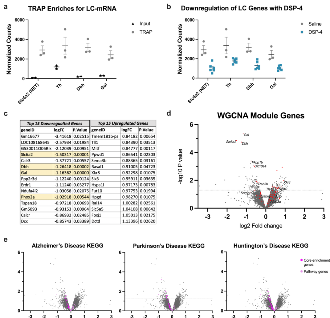
Fig. 4. DSP-4 triggers changes in the LC transcriptome. Mice received saline or DSP-4 (2 x 50 mg/kg, i.p.) and LC gene expression was assessed 1 week later. (a) TRAP allows for purification of mRNA from LC neurons through immunoprecipitation (TRAP, grey), resulting in enrichment of noradrenergic genes compared with mRNA from the entire hindbrain sample (input, black). (b) Differential gene expression (DGE) was assessed between DSP-4 (blue) and saline control (grey) TRAP samples, and revealed that noradrenergic-specific genes, including galanin ( Gal ), norepinephrine transporter ( Slc6a2 ), dopamine \beta -hydroxylase ( Dbh ) and tyrosine hydroxylase ( Th ), were among the most significantly and robustly downregulated transcripts in the LC of DSP-4 treated mice. Data for a and b shown as mean \pm SEM, N=2-6 per group. (c) List of top 15 downregulated and top 15 upregulated DGE, sorted by fold change (logFC) with p < 0.05 . (d) Volcano plot of all filtered, normalized genes (~11,500) with genes from WGCNA-defined module in red. Labeled genes from this module are those of interest based on published connections to neurodegenerative disease. (e) Volcano plots (as shown in d )) highlighting genes from 3 significantly enriched KEGG pathways in our LC data, with GSEA-identified “core enrichment genes” colored magenta, and remaining pathway genes colored light pink.
