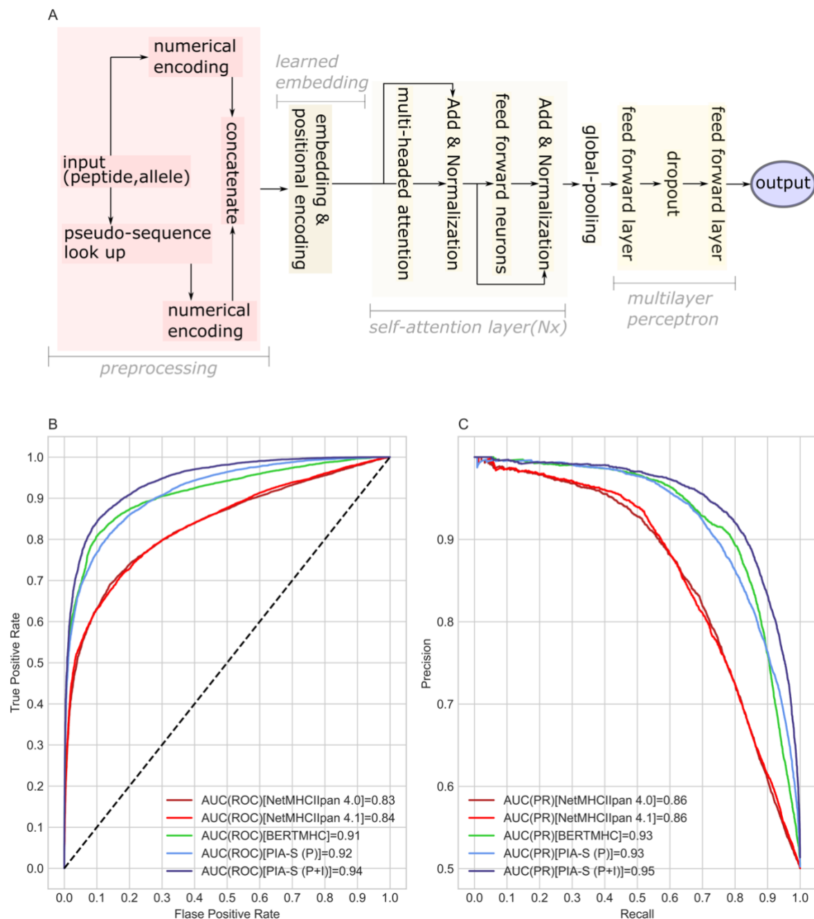
Figure 5: The performance of PIA-S against different publicly available prediction methods. (A) The blueprint of PIA-S (Material and Methods) where, briefly, input peptides and pseudo-sequences are tokenized and then concatenated together. Next, the resulting sequence is fed to a learned embedding layer and subsequently to a stack of self-attention layers. Lastly, the resulting tensor is pooled through a global-average pooling and is fed to a multilayer perceptron to calculate the presentability score. The performance of PIA-S was benchmarked against NetMHCIIpan 4.0 (12), NetMHCIIpan 4.1 and BERTMHC (15) using three HLA-DR immunopeptidomics test datasets that were obtained in the current study. (B) Shows the receiver operating curve (ROC) along with the area under the curve (AUC(ROC)) using the predictions on the three datasets combined. (C) Shows the precision-recall (PR) curve along with the area under the curve (AUC(PR)) using the predictions on the three datasets combined.
