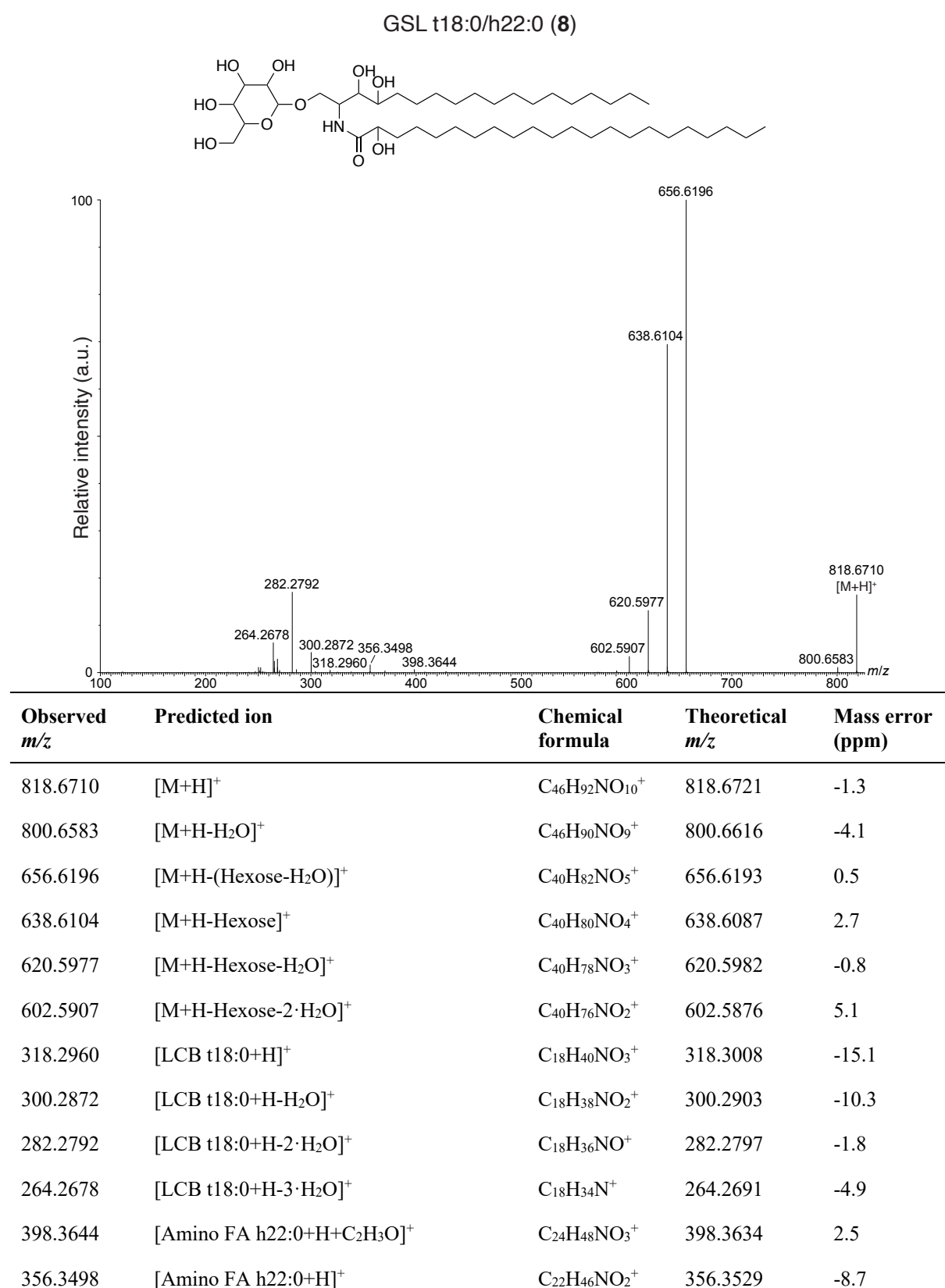
Figure S22: LC-MS/MS analysis of GSL t18:0/h22:0 (8). A putative structure is presented, supported by a list of fragments detected in MS/MS mode (Metabolomics Standards Initiative level 2 annotation 2 ). Fragments were detected in positive ionization MS/MS mode using [M+H]^+ = 818.6702 as the precursor ion (Table 1). The positions of the functional groups were assigned based on the most common structures in the Lipid Maps Structure Database (LMSD) 1 .
