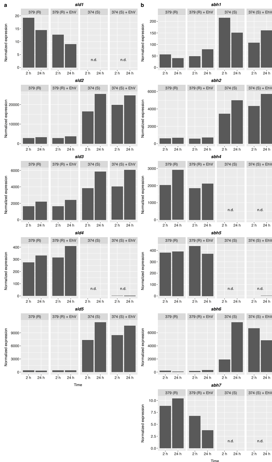
Figure S27: Expression of sphingolipid desaturase ( sld ) and sphingoid base hydroxylase ( sbh ) genes in the resistant E. huxleyi strain 379 and in the susceptible E. huxleyi strain 374 with and without addition of EhV. Normalized expression of (a) sld and (b) sbh genes in the resistant (R) E. huxleyi strain 379 and in the susceptible (S) E. huxleyi strain 374 with and without addition of EhV at 2 h and 24 h ( n = 1 ). Expression of sbh3 was below the limit of detection in all strains and conditions tested. Data was taken from the Marine Microbial Eukaryote Transcriptome Sequencing Project (MMETSP, n = 1 , available at https://www.imicrobe.us , 3 ), samples MMETSP0994-MMETSP0997 ( E. huxleyi 379) and MMETSP1006-MMETSP1009 ( E. huxleyi 374). n.d., not detected.
