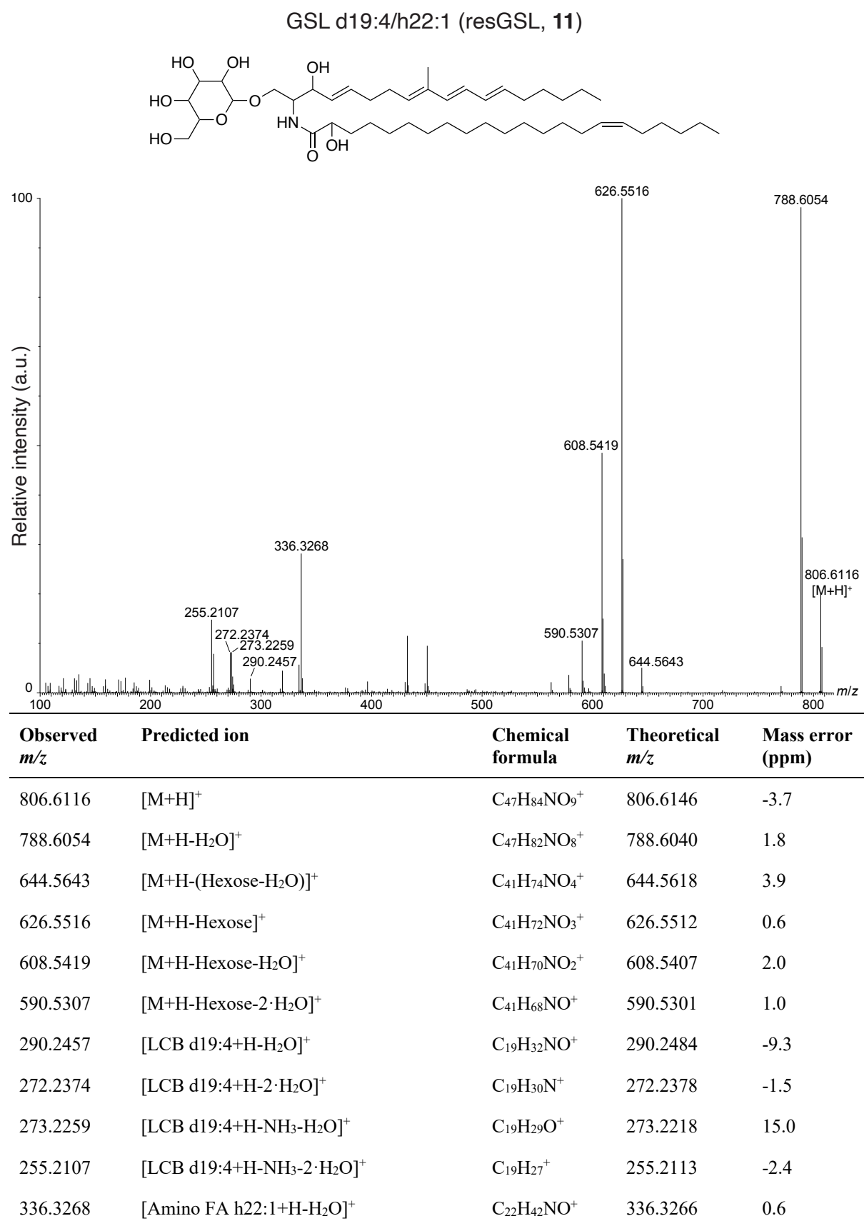
Figure S24: LC-MS/MS analysis of GSL d19:4/h22:1 (resGSL, 11). A putative structure is presented, supported by a list of fragments detected in MS/MS mode (Metabolomics Standards Initiative level 2 annotation 2 ). Fragments were detected in positive ionization MS/MS mode using [M+H]^+ = 806.6127 as the precursor ion (Table 1). The positions of the double bonds and functional groups were assigned based on the most common structures in the Lipid Maps Structure Database (LMSD) 1 .
