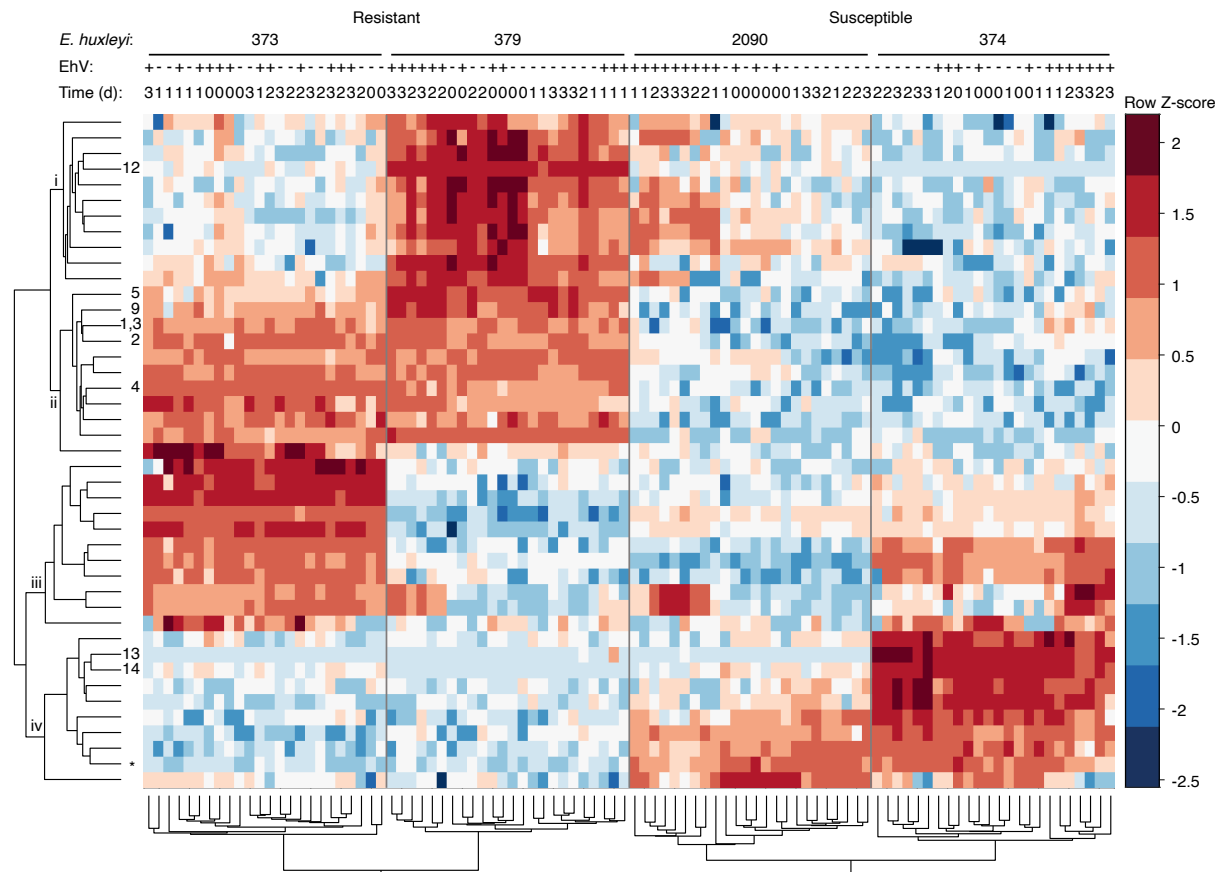
Figure S9: Two-dimensional hierarchical clustering of 43 differential lipid species (Table S1) in four E. huxleyi strains with and without EhV throughout a time course of four days. Clustering was performed on log-transformed and standardized peak areas of the adduct ion with the highest intensity. As in Fig. 2a, the samples are grouped into two main clusters that separate samples of the resistant (R) strains from the susceptible (S) ones ( n = 96 ). Each cluster forms two sub-clusters that further separate the strains. The putative lipid species are also divided into four sub-clusters (i-iv), as in Fig. 2a. Nine GSL species were identified and are marked by numbers (Table 1). The peaks of GSLs 1 and 3, structural isomers with a similar retention time (Table 1), were integrated together as they were not baseline separated. * sGSL d18:2/c22:0.
