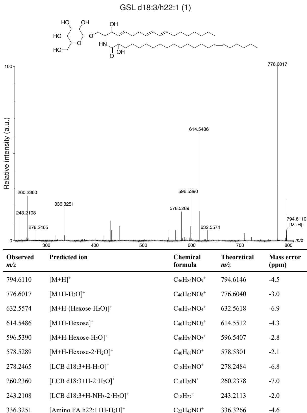
Figure S11: LC-MS/MS analysis of GSL d18:3/h22:1 (1). A putative structure is presented, supported by a list of fragments detected in MS/MS mode (Metabolomics Standards Initiative level 2 annotation 2 ). Fragments were detected in positive ionization MS/MS mode using [M+H] + = 794.6107 as the precursor ion (Table 1). The positions of the double bonds and functional groups were assigned based on the most common structures in the Lipid Maps Structure Database (LMSD) 1 .
