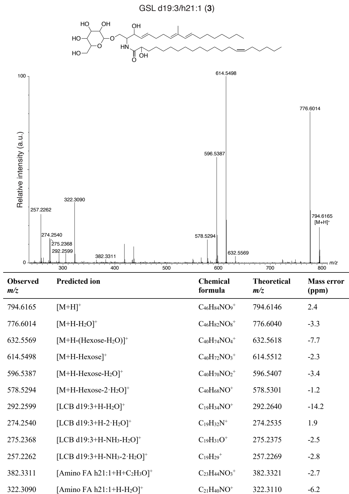
Figure S13: LC-MS/MS analysis of GSL d19:3/h21:1 (3). A putative structure is presented, supported by a list of fragments detected in MS/MS mode (Metabolomics Standards Initiative level 2 annotation 2 ). Fragments were detected in positive ionization MS/MS mode using [M+H]^+ = 794.6107 as the precursor ion (Table 1). The positions of the double bonds and functional groups were assigned based on the most common structures in the Lipid Maps Structure Database (LMSD) 1 .
