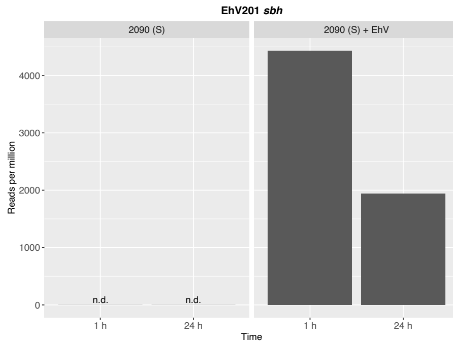
Figure S29: Expression of EhV201 sphingoid base hydroxylase ( sbh ) during infection of the susceptible E. huxleyi strain 2090. Data taken from Rosenwasser et al. , 2014 5 ( n = 1 ). n.d., not detected.
