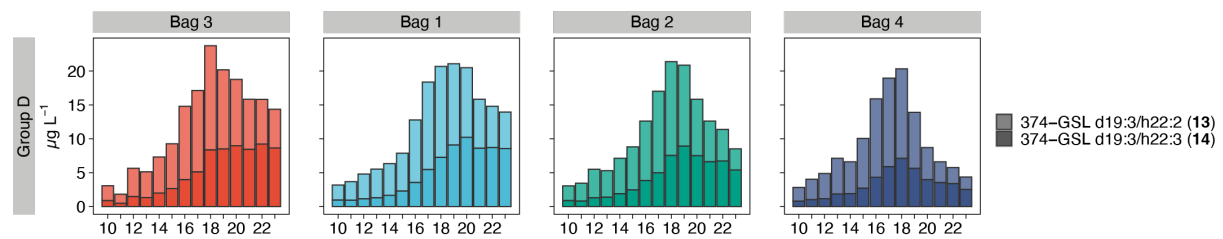
Figure S30: Changes in in cellular content of 374-GSL species (group D) in response to viral infection of natural E. huxleyi populations in a mesocosm experiment. Concentration of 374-GSL species correlates with the population dynamics in the four bags (Table S7). Bags are ordered by increasing EhV abundance, with the lowest abundance in bag 3 and the highest in bag 4, as presented in Fig. 5b.
