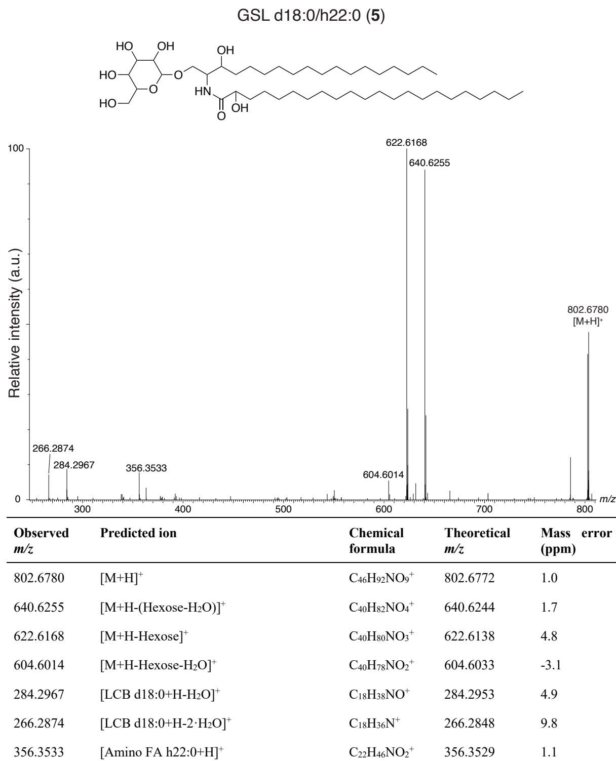
Figure S15: LC-MS/MS analysis of GSL d18:0/h22:0 (5). A putative structure is presented, supported by a list of fragments detected in MS/MS mode (Metabolomics Standards Initiative level 2 annotation 2 ). Fragments were detected in positive ionization MS/MS mode using [M+H]^+ = 802.6722 as the precursor ion (Table 1). The positions of the functional groups were assigned based on the most common structures in the Lipid Maps Structure Database (LMSD) 1 .
