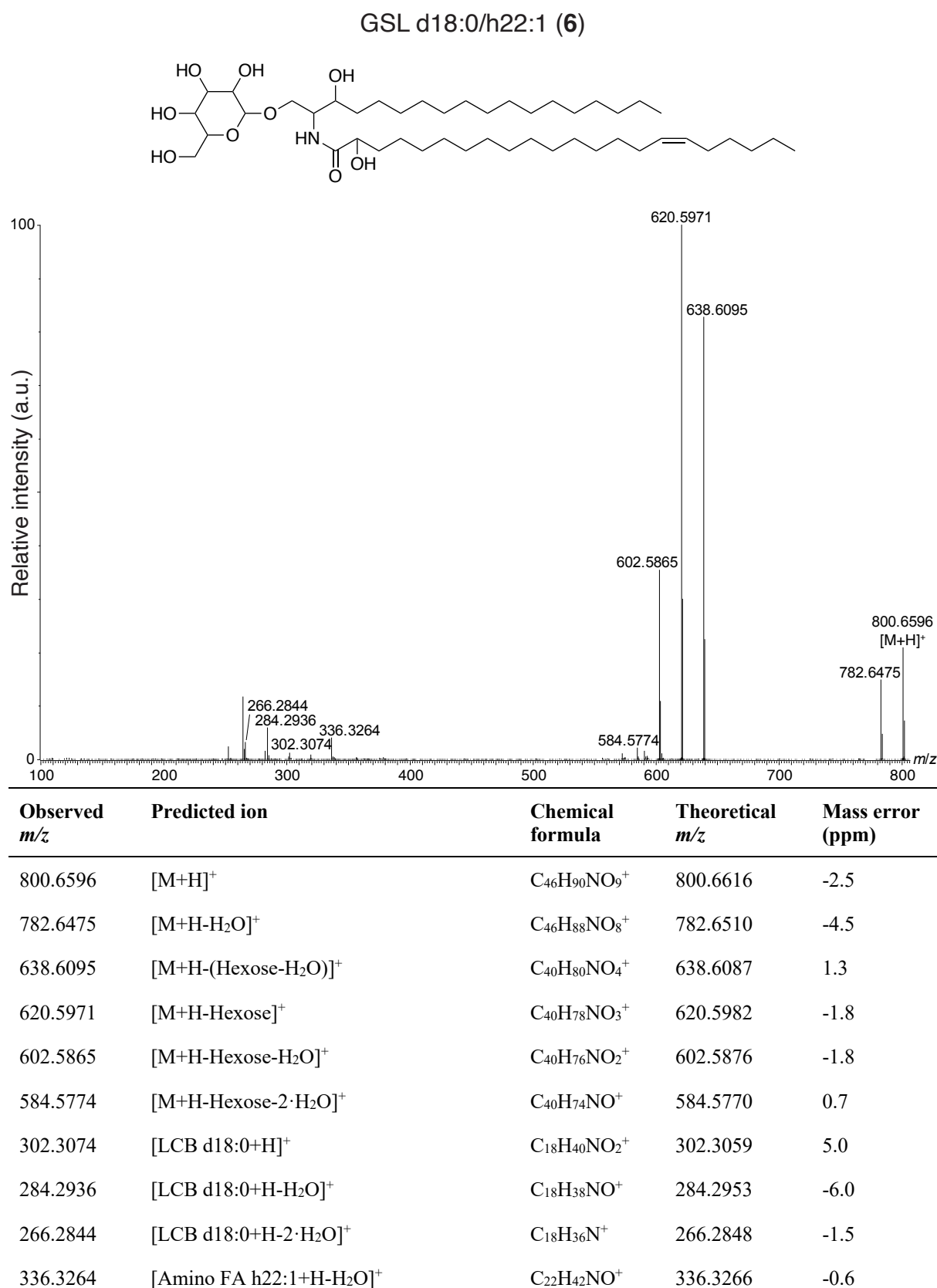
Figure S20: LC-MS/MS analysis of GSL d18:0/h22:1 (6). A putative structure is presented, supported by a list of fragments detected in MS/MS mode (Metabolomics Standards Initiative level 2 annotation 2 ). Fragments were detected in positive ionization MS/MS mode using [M+H]^+ = 800.6600 as the precursor ion (Table 1). The positions of the double bond and functional groups were assigned based on the most common structures in the Lipid Maps Structure Database (LMSD) 1 .
