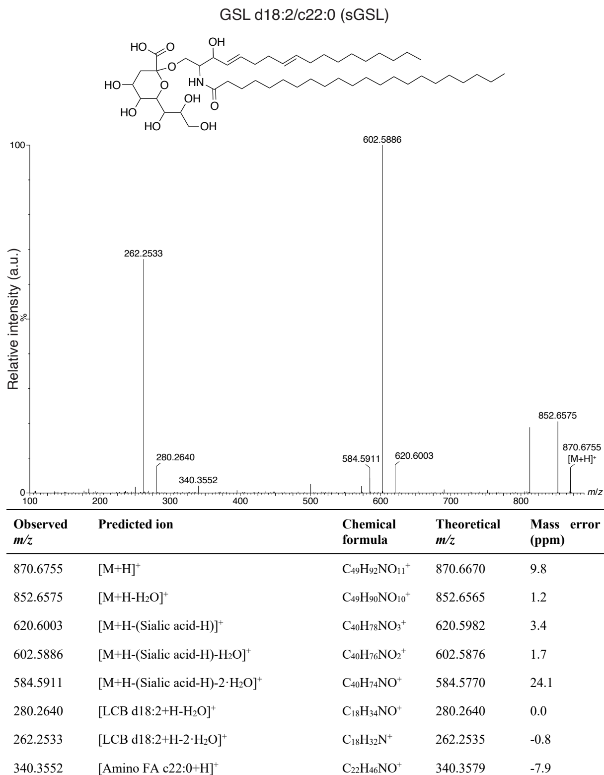
Figure S40: LC-MS/MS analysis of sGSL d18:2/c22:0. A putative structure is presented, as reported previously 7 . The structure is supported by a list of fragments detected in MS/MS mode (Metabolomics Standards Initiative level 2 annotation 2 ). Fragments were detected in positive ionization MS/MS mode using [M+H]^+ = 870.6670 as the precursor ion (Table S3).
