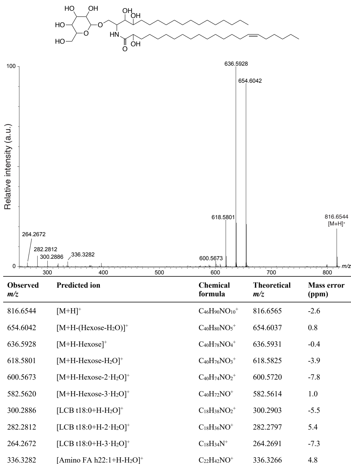
Figure S16: LC-MS/MS analysis of GSL t18:0/h22:1 (9). A putative structure is presented, supported by a list of fragments detected in MS/MS mode (Metabolomics Standards Initiative level 2 annotation 2 ). Fragments were detected in positive ionization MS/MS mode using [M+H]^+ = 816.6531 as the precursor ion (Table 1). The positions of the double bonds and functional groups were assigned based on the most common structures in the Lipid Maps Structure Database (LMSD) 1 .
