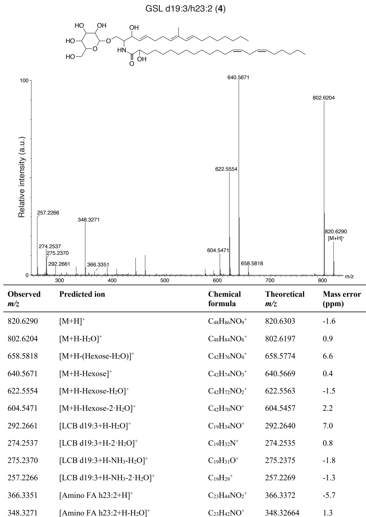
Figure S14: LC-MS/MS analysis of GSL d19:3/h23:2 (4). A putative structure is presented, supported by a list of fragments detected in MS/MS mode (Metabolomics Standards Initiative level 2 annotation 2 ). Fragments were detected in positive ionization MS/MS mode using [M+H] + = 820.6278 as the precursor ion (Table 1). The positions of the double bonds and functional groups were assigned based on the most common structures in the Lipid Maps Structure Database (LMSD) 1 .
