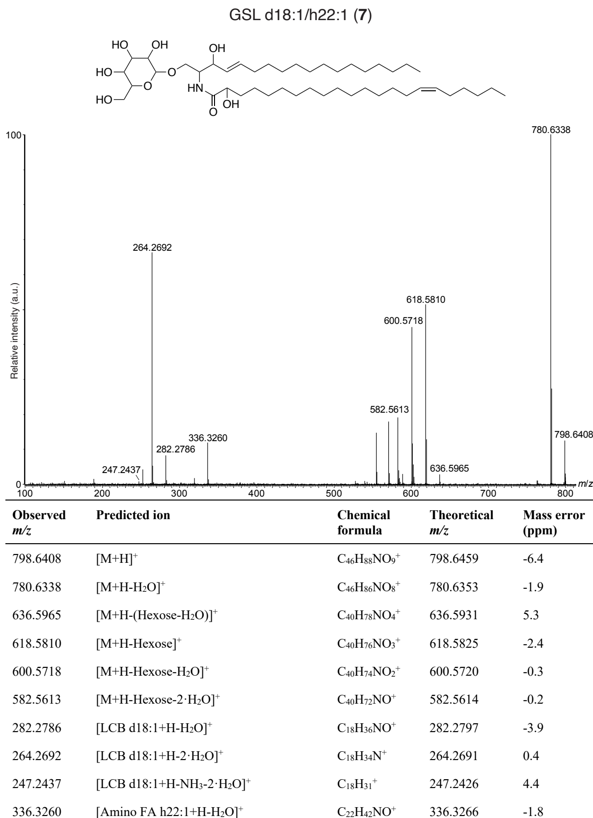
Figure S21: LC-MS/MS analysis of GSL d18:1/h22:1 (7). A putative structure is presented, supported by a list of fragments detected in MS/MS mode (Metabolomics Standards Initiative level 2 annotation 2 ). Fragments were detected in positive ionization MS/MS mode using [M+H] + = 798.6440 as the precursor ion (Table 1). The positions of the double bonds and functional groups were assigned based on the most common structures in the Lipid Maps Structure Database (LMSD) 1 .
