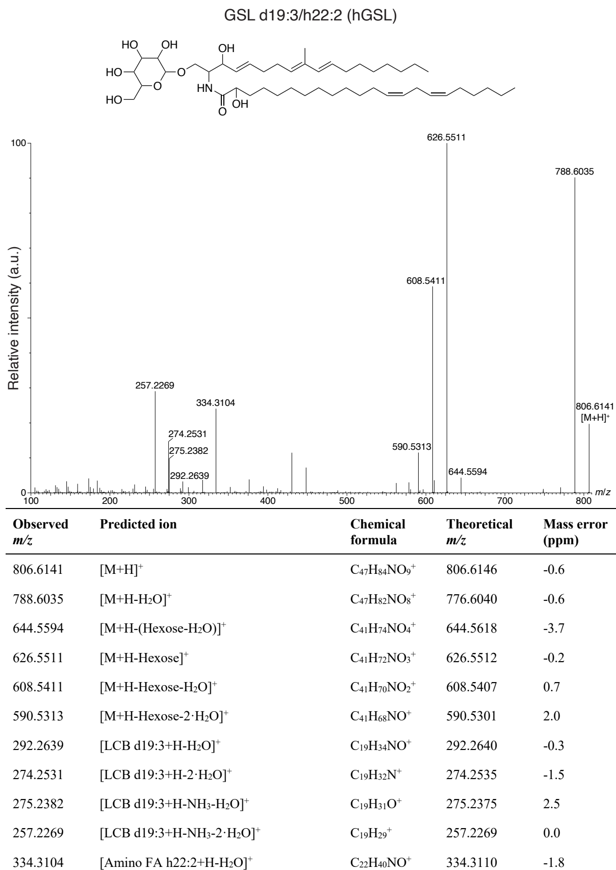
Figure S39: LC-MS/MS analysis of hGSL d19:3/h22:2. A putative structure is presented, as reported previously 6 . The structure is supported by a list of fragments detected in MS/MS mode (Metabolomics Standards Initiative level 2 annotation 2 ). Fragments were detected in positive ionization MS/MS mode using [M+H]^+ = 806.6146 as the precursor ion (Table S3).
