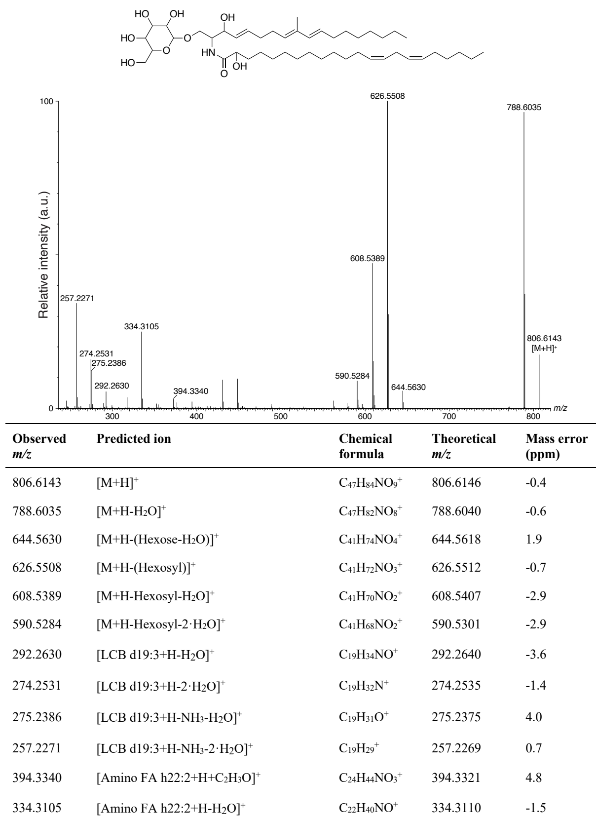
Figure S18: LC-MS/MS analysis of GSL d19:3/h22:2 (374-GSL, 13). A putative structure is presented, supported by a list of fragments detected in MS/MS mode (Metabolomics Standards Initiative level 2 annotation 2 ). Fragments were detected in positive ionization MS/MS mode using [M+H] + = 806.6143 as the precursor ion (Table 1). The positions of the double bonds and functional groups were assigned based on the most common structures in the Lipid Maps Structure Database (LMSD) 1 .
