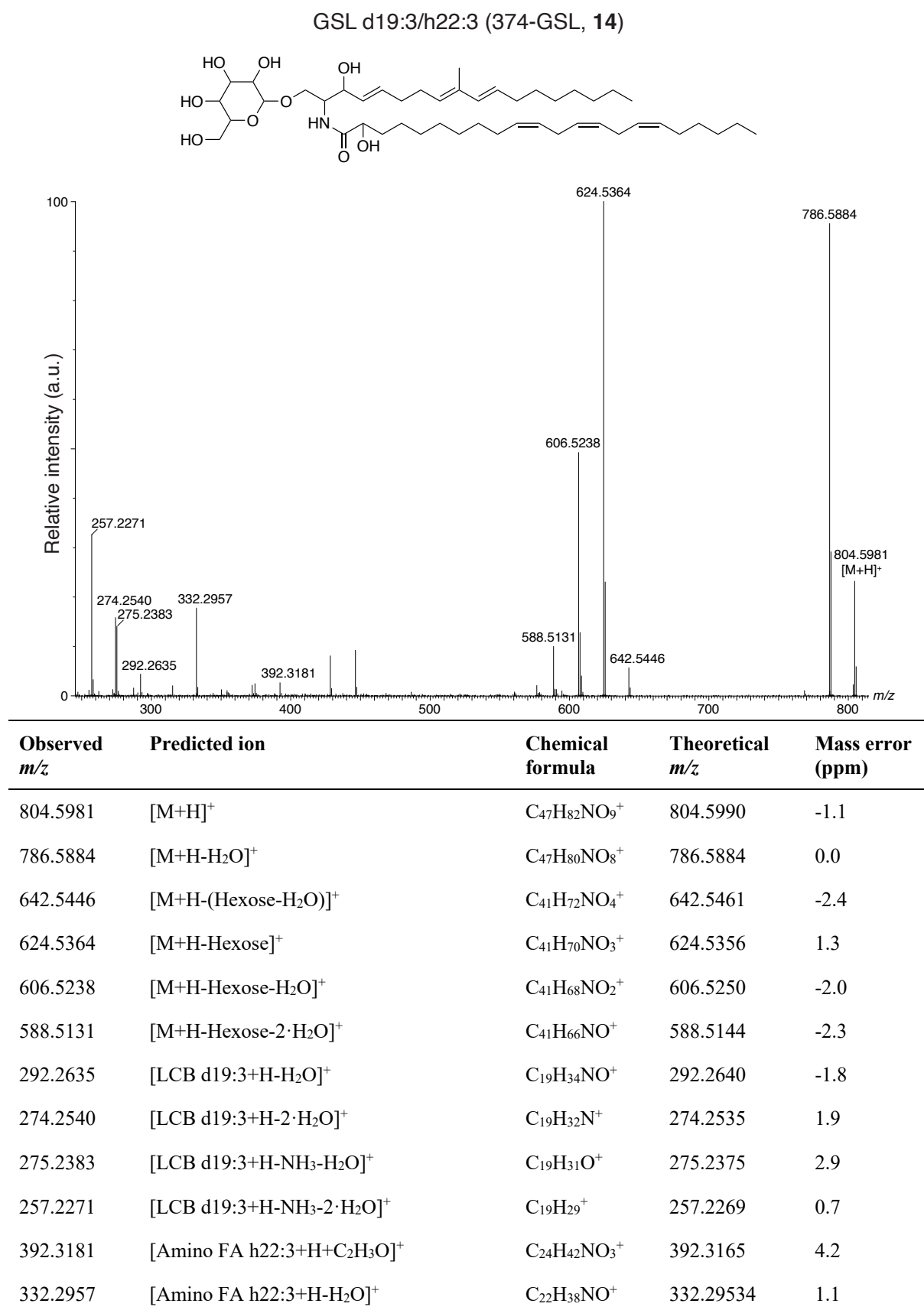
Figure S19: LC-MS/MS analysis of GSL d19:3/h22:3 (374-GSL, 14). A putative structure is presented, supported by a list of fragments detected in MS/MS mode (Metabolomics Standards Initiative level 2 annotation 2 ). Fragments were detected in positive ionization MS/MS mode using [M+H]^+ = 804.5981 as the precursor ion (Table 1). The positions of the double bonds and functional groups were assigned based on the most common structures in the Lipid Maps Structure Database (LMSD) 1 .
