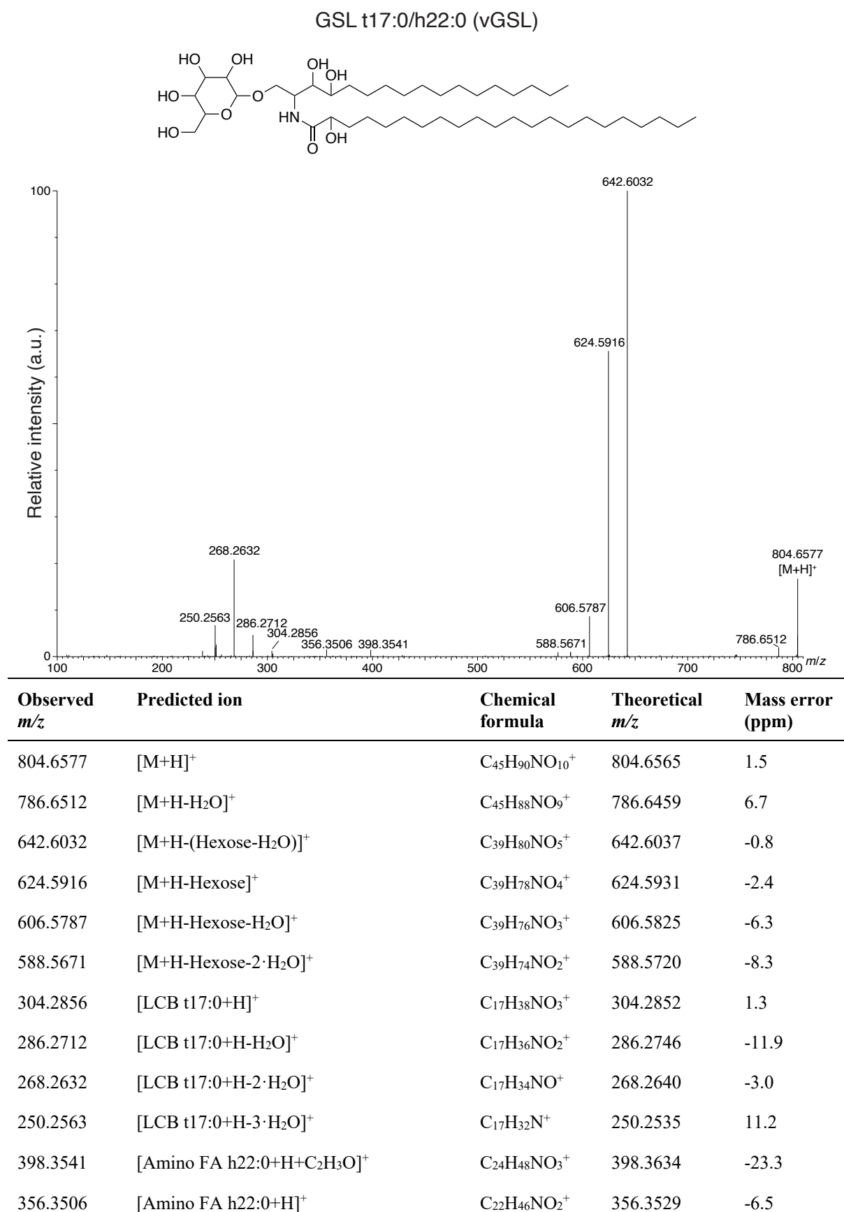
Figure S41: LC-MS/MS analysis of vGSL t17:0/h22:0. A putative structure is presented, as reported previously 8 . The structure is supported by a list of fragments detected in MS/MS mode (Metabolomics Standards Initiative level 2 annotation 2 ). Fragments were detected in positive ionization MS/MS mode using [M+H] + = 804.6565 as the precursor ion (Table S3).
