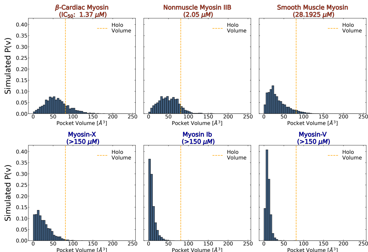
Figure 4. The probability of adopting open pocket conformations is greater among blebbistatin-sensitive isoforms (top row) than insensitive isoforms (bottom row). MSM-weighted distributions of blebbistatin pocket volumes in simulations of nucleotide-free isolated myosin motor domains show that myosin-IIs (top row) are more likely to exceed the blebbistatin pocket volume of a holo crystal structure (PDB: 1YV3, orange line) than non-class II myosins. Among myosin-IIs, those with lower IC_{50} s 22,25–28,38 have more right-shifted pocket volume distributions.
