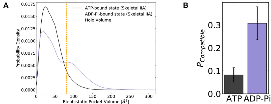
Figure 3. Blebbistatin pocket opening preferentially occurs in the ADP*Pi state. A.
