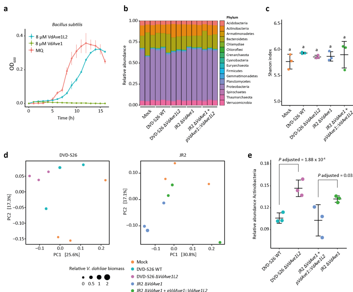
Figure 4. VdAve1L2 impacts Actinobacteria in the tomato root microbiota. (a) VdAve1L2 is an antibacterial effector protein. In vitro growth of Bacillus subtilis is inhibited by VdAve1L2. The previously characterized antibacterial effector VdAve1 (Snelders et al. , 2020) was included as positive control for bacterial growth inhibition and displays a differential activity compared to VdAve1L2. Ultrapure water (MQ) was included as negative control. Graph displays the average OD 600 of three biological replicates ± SD. (b) Relative abundance of bacterial phyla in tomato root microbiota ten days after inoculation with wild-type V. dahliae strain DVD-S26, the corresponding DVD-S26 VdAve1L2 deletion mutant, a V. dahliae strain JR2 VdAve1 deletion mutant and the corresponding VdAve1L2 expression mutant as determined by 16S ribosomal DNA profiling. (c) V. dahliae colonization does not impact α-diversity of tomato root microbiota. The plot displays the average Shannon index ± SD (one-way ANOVA and Tukey's post-hoc test; p<0.05; N=3). (d) Principal coordinate analysis based on Bray-Curtis dissimilarities uncovers separation of root microbiome compositions based on presence of VdAve1L2. (e) Differential abundance analysis of bacterial phyla reveals a repression of Actinobacteria in the tomato root microbiota colonized by V. dahliae strains that secrete VdAve1L2 (Wald test, N=3).
