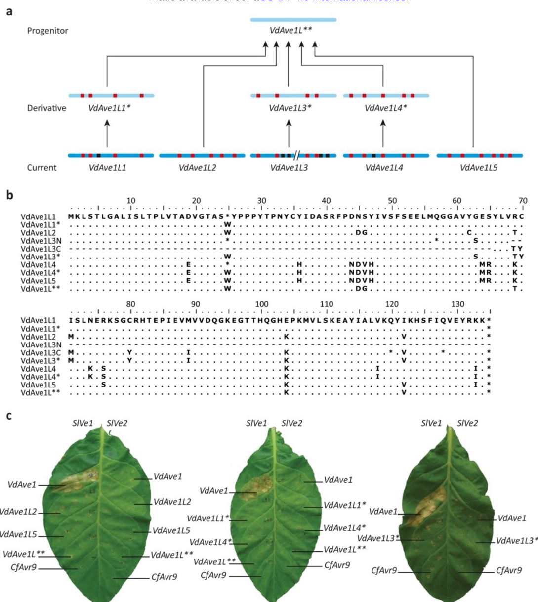
Figure 2. VdAve1L proteins are not recognized by the immune receptor SIVe2. (a) Schematic overview of the relationship between the currently identified VdAve1L alleles (excluding VdAve1L6 ), the derived alleles VdAve1L1* , VdAve1L3* , VdAve1L4* and the putative progenitor allele ( VdAve1L** ). The blue bars indicate the alleles, the line with arrows indicates the relationship between the current alleles, the artificial derivatives, and the progenitor. Within the blue bars the red blocks indicate point mutations, the black blocks indicate premature stop codons and the double slash (//) indicates discontinuity. (b) Alignment of VdAve1L proteins ( VdAve1L1 – VdAve1L5 ), derivatives ( VdAve1L1* , VdAve1L3* and VdAve1L4* ), the progenitor ( VdAve1L** ), the N-terminal sequence of VdAve1L3 ( VdAve1L3N ) and the C-terminal sequence of VdAve1L3 ( VdAve1L3C ). Dots (.) indicate amino acid conservation, lines (-) indicate the absence of an amino acid, and an asterisk (*) indicates a stop codon at the respective position. (c) Co-expression of VdAve1L alleles with the tomato immune receptors SIVe1 and SIVe2 . Co-expression of VdAve1 with SIVe1 serves as positive control for the induction of a hypersensitive response. The sequence unrelated Cladosporium fulvum effector Avr9 serves as a negative control for recognition by SIVe1 and SIVe2 .
