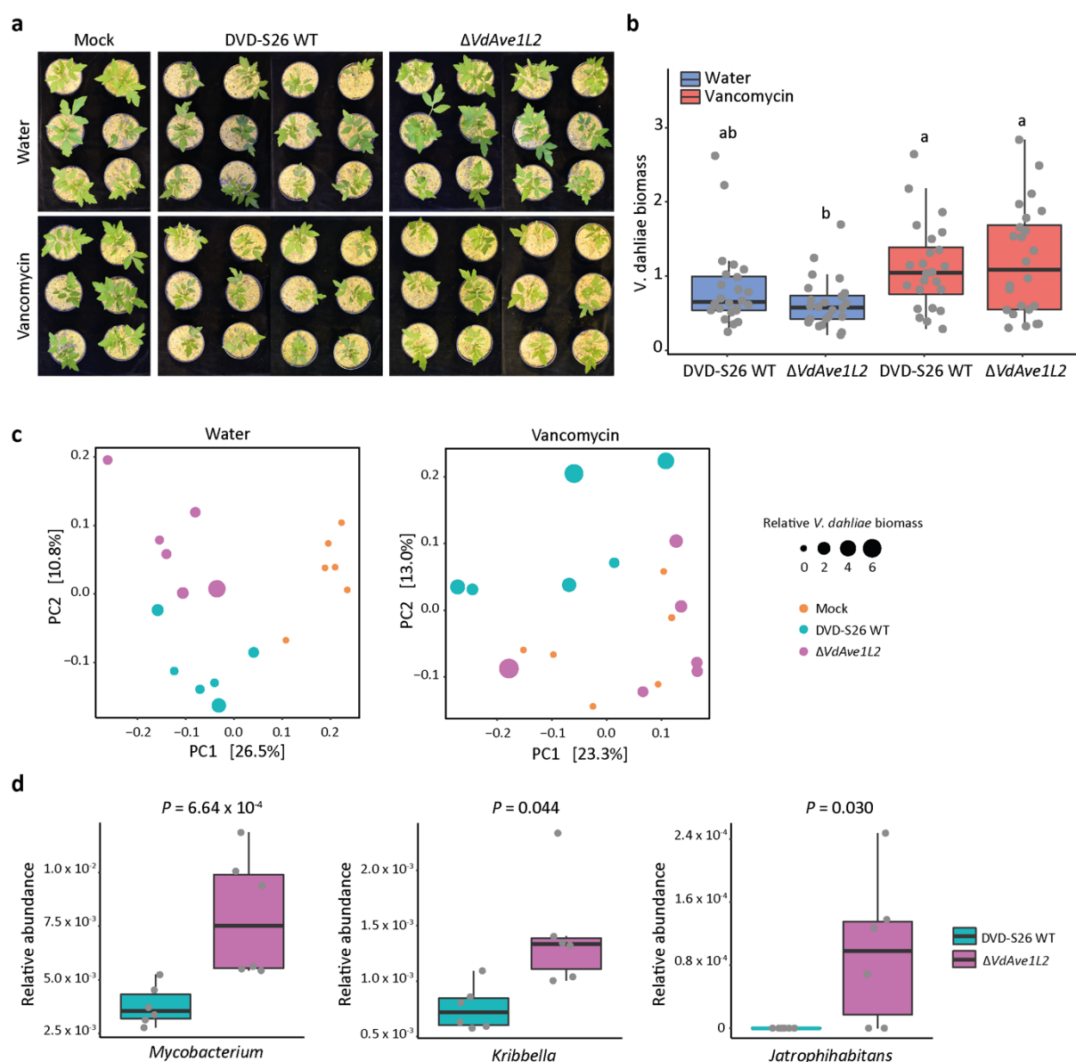
Figure 6. Treatment of tomato root microbiota with vancomycin diminishes the virulence contribution of VdAve1L2. (a) Phenotypes of tomato plants harboring vancomycin-treated or water-treated microbial communities infected by wild-type V. dahliae and the VdAve1L2 deletion mutant at 19 days post inoculation. (b) Relative V. dahliae biomass in tomato stem tissue determined with real-time PCR (one-way ANOVA and Tukey's post-hoc test; p < 0.05 ; N = 24 ) (c) Principal coordinate analysis based on Bray-Curtis dissimilarities uncovers separation of root microbiota compositions in tomato plants harboring water-treated microbial communities, but not vancomycin-treated microbial communities colonized by both V. dahliae strains and upon mock treatment. (d) Relative abundance of the three Actinobacterial genera that are depleted from the tomato plants harboring the water-treated microbial community colonized by V. dahliae WT when compared with colonization by the VdAve1L2 deletion mutant (Wald test; N = 6 ).
