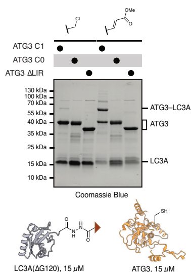
Extended Data Fig. 3| Modification of ATG3 with LC3A is dependent on LIR ATG3 . Coomassie Blue stained SDS-PAGE gel showing the reaction of LC3A probes 3 and 4 (15 \mu M) with ATG3 C1, C0 and \Delta LIR (15 \mu M). Source data and full-gel images are available in the Source Data File.
