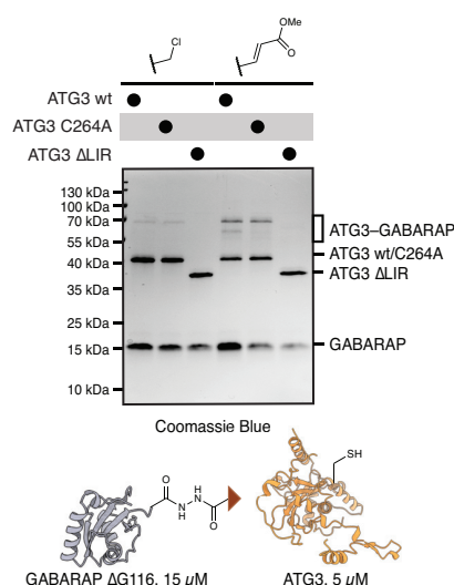
Extended Data Fig. 2| Modification of ATG3 wild-type is dependent on LIR ATG3 . Coomassie Blue stained SDS-PAGE gel showing the reaction of GABARAP probes 1 and 2 (15 \mu M) with ATG3 wt, C264A and \Delta LIR (5 \mu M). Source data and full-gel images are available in the Source Data File.
