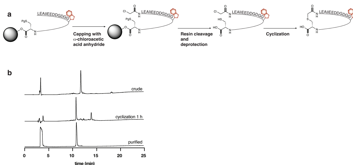
Extended Data Fig. 4| Preparation of cyclized LIR ATG3 peptide 6. a , Synthetic scheme describing the preparation of 6 . A cysteine residue is introduced at the C-terminus of the LIR motif. Following standard Fmoc-SPPS the LIR peptide is capped at its N-terminus with \alpha -chloroacetic acid anhydride. Following resin cleavage, the peptide is cyclized by cysteine alkylation. b , Analytical RP-HPLC chromatograms showing the cyclization of the LIR peptide to provide 6 . Upper chromatogram shows the linear peptide prior to cyclization. Middle chromatogram shows the cyclization reaction after 1 h. Lower chromatogram shows purified peptide 6 .
