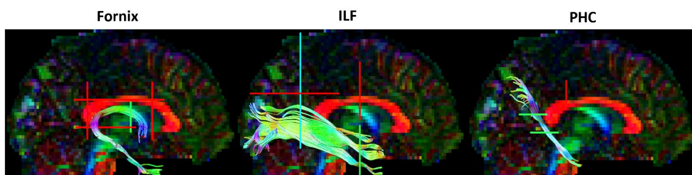
Figure 3. Construction of Tract Streamlines.
