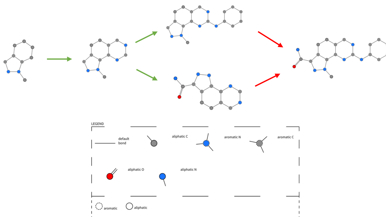
Figure S8: Diagrams showing our various routes used in attempts to generate molecules that included the final substructure. Green arrows represent successful steps where the molecule following the arrow was included in generated molecules. Red arrows are unsuccessful steps.
