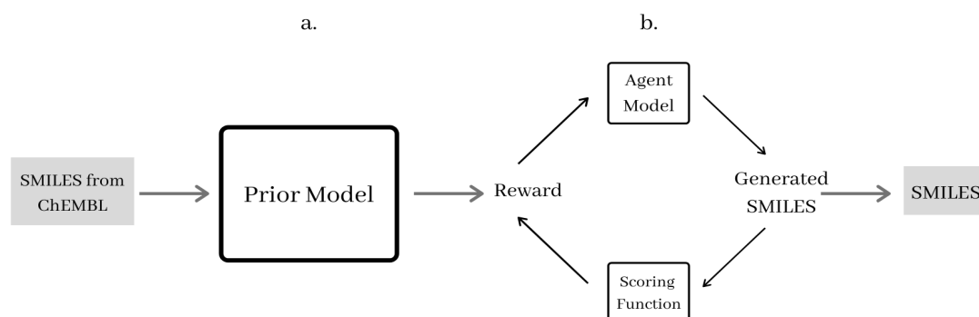
Figure 1: High-level diagram displaying the architecture of the deep reinforcement learning model used by Popova et al and Olivecrona et al. 29,30 (a) Supervised learning language model. The prior model learns to generate novel SMILES from a large dataset of SMILES from ChEMBL. 31 (b) Reinforcement Learning. The agent model (based on the prior model) is trained to generate SMILES that return a favourable reward.
