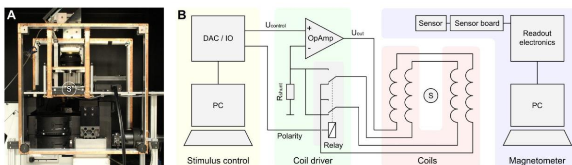
Figure 1: Electrophysiological setup with an integrated three-axis Helmholtz coil system. A: Extracellular multielectrode recording setup with integrated coils. B: Schematic overview of the setup components for the generation and measurement of magnetic field stimuli. Coil driver and coils are shown for one of three axes. The placement of the specimen is indicated by the letter S in A and B.
