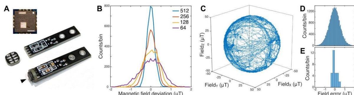
Figure 2: Miniature vector magnetometer. A: Two-part sensor board design. The QMC5883L magnetic sensor is marked by an arrowhead. Sensor 3 mm x 3 mm. Inset top left: Position of the sensor dies inside the QMC5883L package, top view onto the package. White dot marks pin 1. Inset scale bar = 1 mm. B: Noise floor of an exemplary QMC5883L for the four available oversampling settings 64x - 512x. C: Trajectory of rotating the sensor in the natural earth magnetic field (49 \mu T) for approximately 3 minutes after calibration on the smallest oversampling setting. D: Residuals between the trajectory data in C and a homogeneous natural field. E: Residuals as in D averaged over 15 s to reduce noise for 30 stationary orientations in the natural magnetic field.
