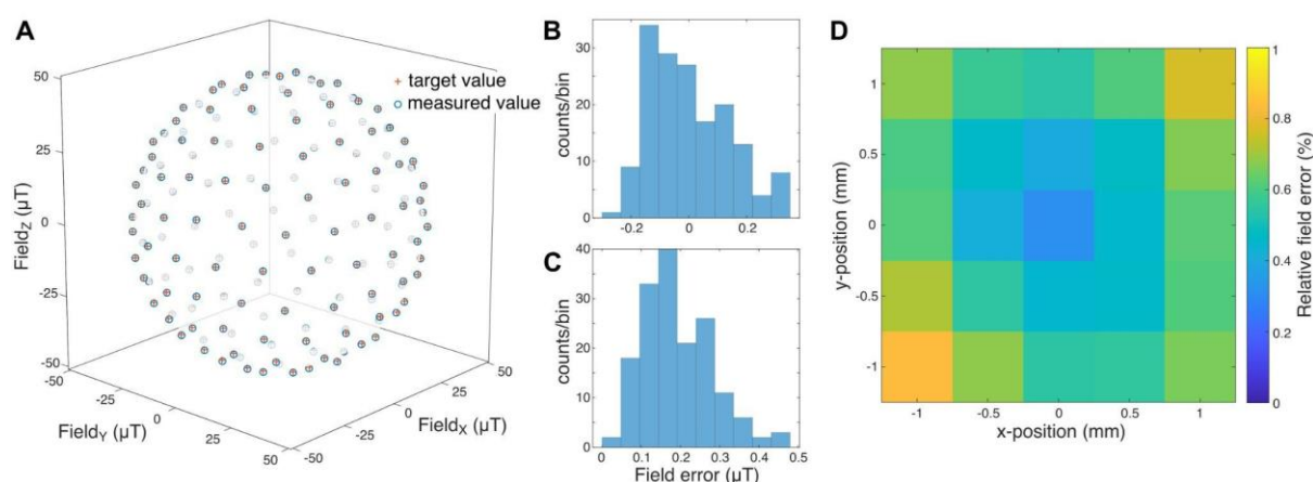
Figure 4: Setup calibration. A: Precision of 162 uniformly distributed field vectors in the calibrated setup. Red crosses: target vector, blue circles: measured field vector B: Magnitude deviations from the target of 50 μT. C: Euclidean distance between target and measured field vector. D: Field homogeneity in a 2 mm * 2 mm area in the recording chamber. At each location a spherical magnetic field stimulus with 44 vectors was analyzed. For each location, the mean Euclidean error is shown in percent of the target radius.
