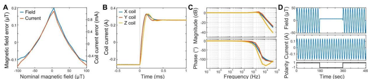
Figure 3: Coil amplifier. A: Coil amplifiers show an approximately linear response over a large range. Magnetic field strength and coil current were measured for a control voltage sweep corresponding to a magnetic field strength of approx -100 μT to 100 μT. Residuals of a linear fit of magnetic field and coil current are shown. Average of 3 repeats, error bars: ±SD. B: Coil current responses to a control voltage step for the three coils corresponding to a transition from -100 to 100 μT. Frequency compensation was adjusted for maximal speed of the transition and minimal overshoot. C: Bode plots of amplitude attenuation (top) and phase shift (bottom) of the coil current for sinusoidal control voltages from 0.1 Hz to 50 kHz at ± earth magnetic field strength. D: Field blanking. By switching the coil wiring from serial to anti-serial (bottom) the magnetic field produced by the coils is canceled out (top) though the coils are still under current (middle). Note that the offset corresponds to the remaining natural magnetic field.
