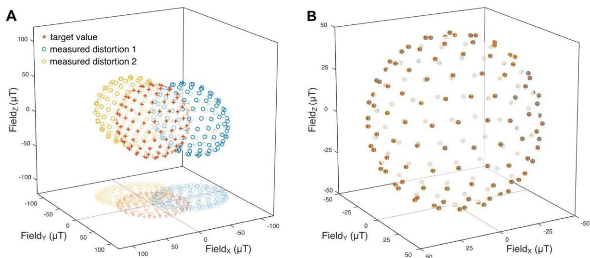
Figure 5: Compensation of strong distortions. A: A ferromagnetic steel bar was placed inside a previously calibrated setup in two orientations and a magnetic sphere stimulus with a target radius of 50 \mu\text{T} was applied (red crosses). The resulting sphere was offset and deformed for both positions of the metal bar (blue and yellow circles). B: After calibration, offset and deformation of the sphere were largely reduced, yielding average errors of 0.63% (distortion 1, blue circles) and 0.51% (distortion 2, yellow circles).
