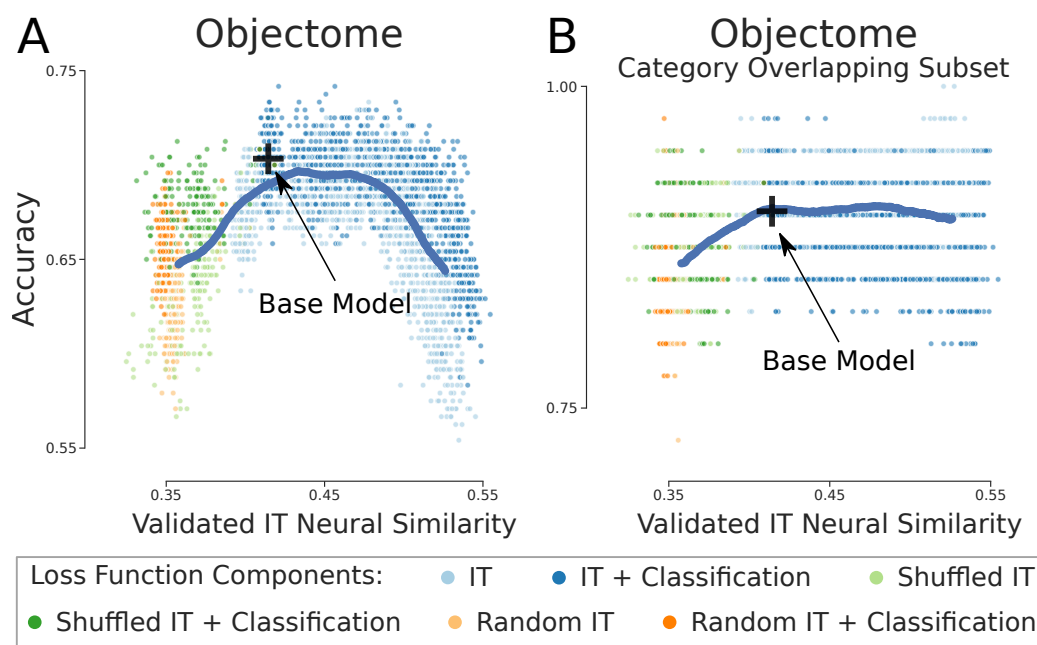
Figure A.1: Higher levels of validated IT neural similarity are associated with decreasing classification accuracy on Objectome images over all, but not Objectome images with categories overlapping the IT training set categories. A) Classification accuracy versus validated IT neural similarity for all model optimization conditions at all validation checkpoints reveals decreasing accuracy on the full Objectome image set which contains 20 categories not overlapping with the IT training set. B) Like in A but for the Objectome image set filtered to overlapping categories with the IT training set has relatively stable classification accuracy. In all plots, the black cross represents the average base model position, and the heavy blue line is a sliding X, Y average of all conditions merely to visually highlight trends. Five seeds for each condition are plotted.
