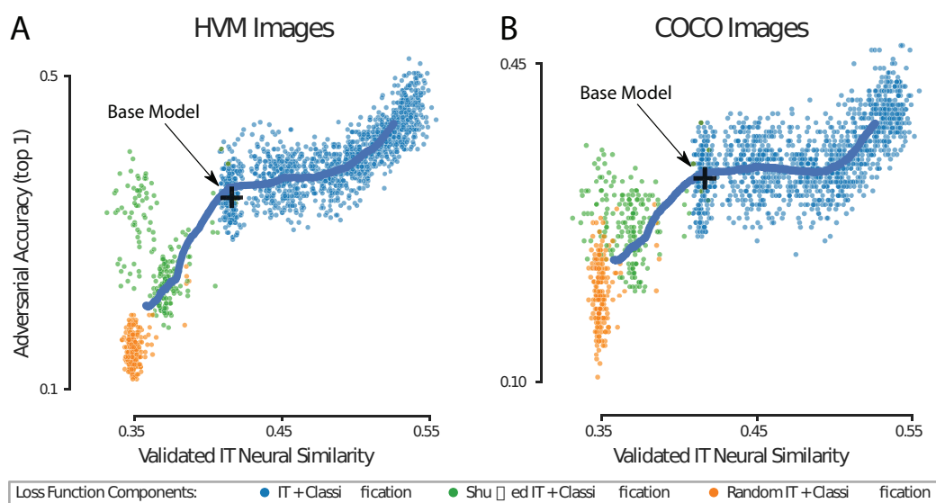
Figure 4: IT neural similarity correlates with improved white box adversarial robustness. A) held out animal and image IT neural similarity is plotted against white box adversarial accuracy (PGD L_{\infty} \epsilon = 1/1020 ) on the HVM image set measured across multiple training time points for all neural loss ratio conditions, random IT target matrix conditions, and image shuffled IT target matrix conditions. B) Like in A) but for COCO images. In all plots, the black cross represents the average base model position, and the heavy blue line is a sliding X, Y average of all conditions merely to visually highlight trends. Five seeds for each condition are plotted.
