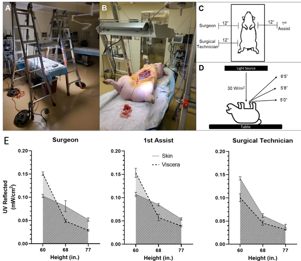
Figure 5: Model of provider exposure to UV light. (A) Overhanging light to achieve UV-A irradiance of 30 W/m². (B) Light source overlying pig with adjustable light source using pulley/lever system. (C) Operative team positions around the porcine subject for reflected UV-A measurements. (D) Height variables for light measurements. (E) Comparison of reflected UV-A irradiance measured at the surgeon, 1 st assist, surgical technician locations. Solid line marks reflected irradiance based off skin only measurements. Dotted line represents reflected irradiance based off visceral intensities.
