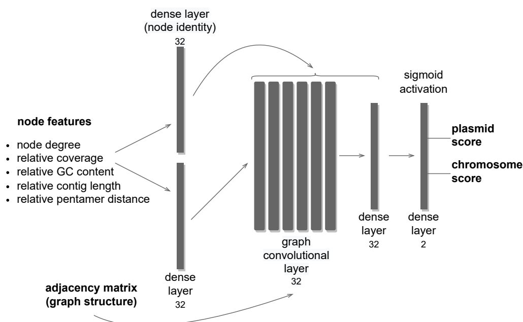
Figure 1 Model architecture of pIASgraph. The model uses as inputs the assembly graph structure and five input features per node (contig). The core of the architecture is composed of six graph convolutional layers. The model generates two outputs per node, which facilitate the classification of plasmids and chromosomes as two separate classification tasks.
