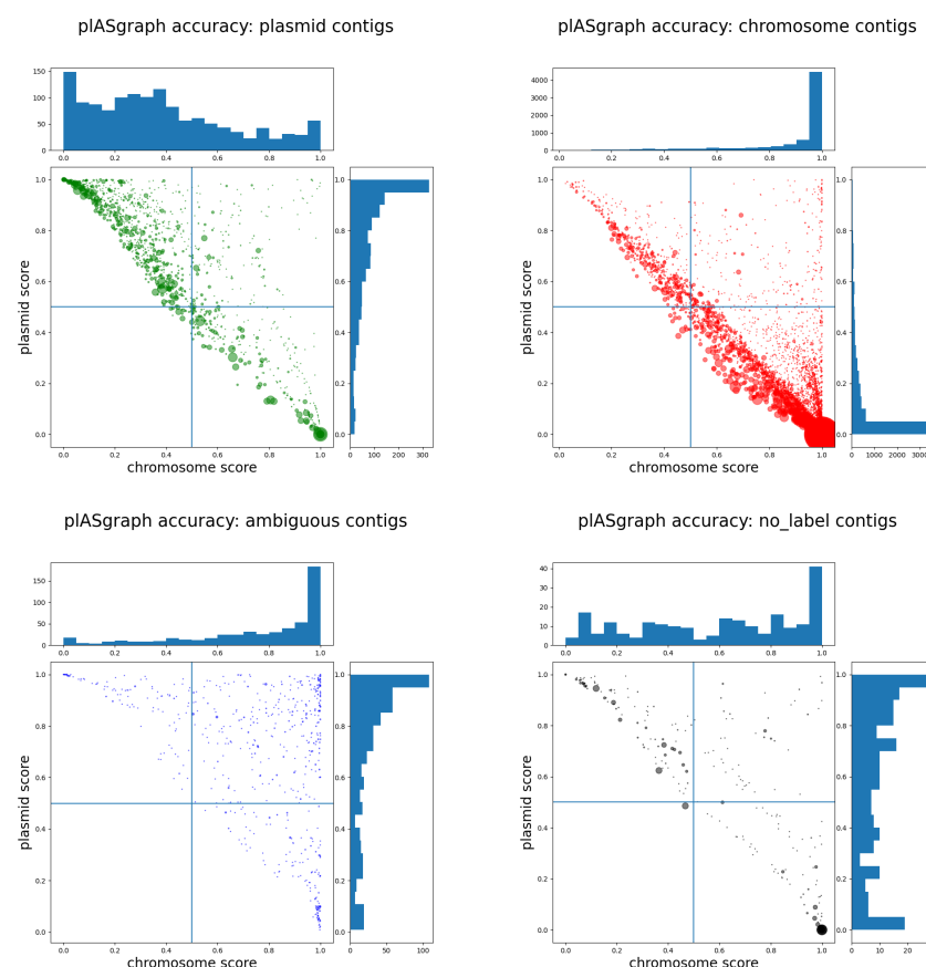
Figure S7 Results on the 96 C. freundii samples (9118 contigs). Each dot represents a contig, its radius being proportional to the contig length. Contigs are split in four panels according to their ground truth label. Each contig is shown with coordinates being its chromosome score (x-axis) and its plasmid score (y-axis).
