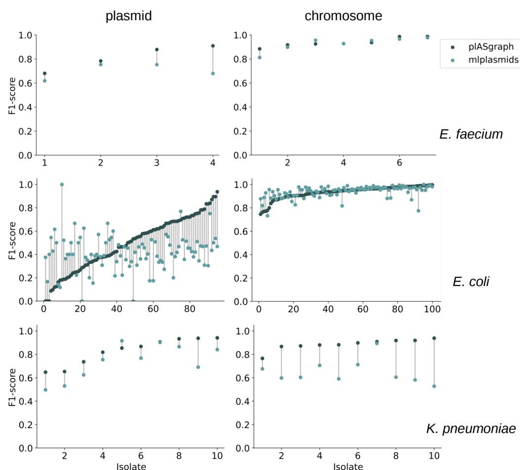
Figure 2 Evaluation of the species-specific plASgraph models in comparison to mplasmids. Each row compares the F1-score of plASgraph to mplasmids on individual testing isolates for both plasmid (left) and chromosome (right) classification tasks. The isolates without plasmids are not shown in graphs on the left, as F1-score is then undefined. Rows from top to bottom correspond to E. faecium , E. coli , and K. pneumoniae data sets respectively. The models are always trained and tested on the same species.
